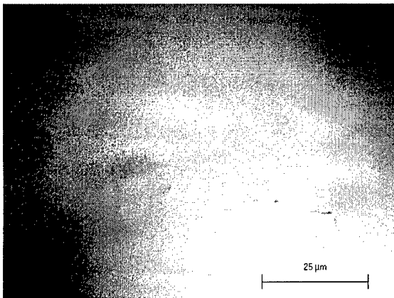
Wafer 5 – Trench 4 at 1000x magnification – post 60 minute polish, pressure = 5 lb/in 2 , rpm = 180 condition
