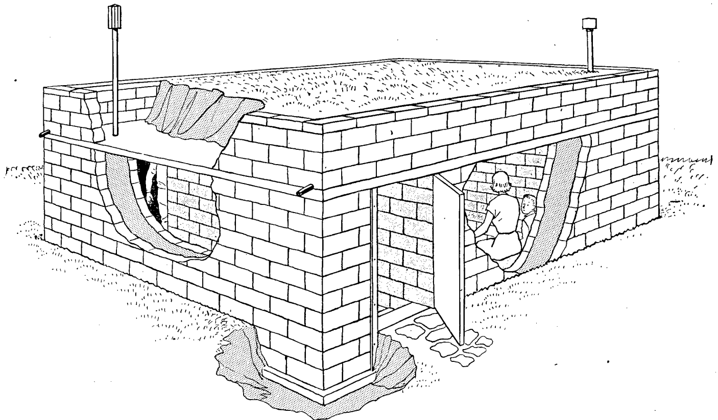
Figure 9.—Aboveground double-wall shelter
