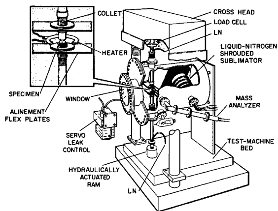
Figure 1.- Test apparatus used to investigate the influence of environment on adhesion.
