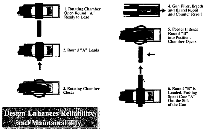
Figure 2. "Push-Through" Principle of 40-mm CTWS Weapon.
