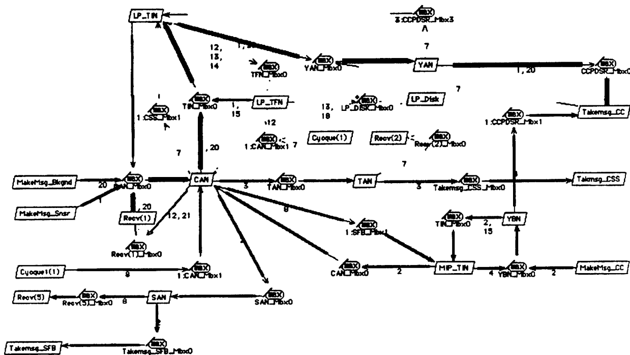
Figure 2. CPN model of the communications switching system
