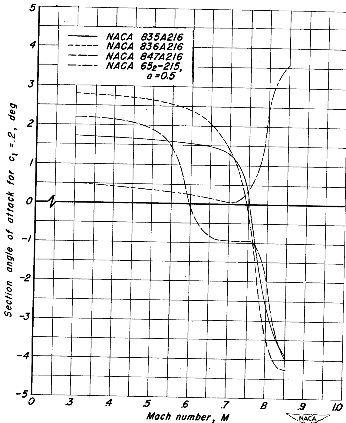
Figure 6.- The variation with Mach number of the section angle of attack for a lift coefficient of 0.2 for the NACA 835A216, 836A216, 847A216 and 65 2 -215, \alpha = 0.5 , airfoils.
