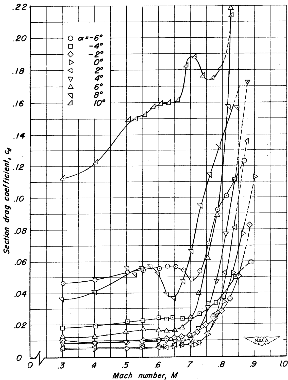
Figure 21.—The variation of section drag coefficient with Mach number at various angles of attack for the NACA 836A110 airfoil.
