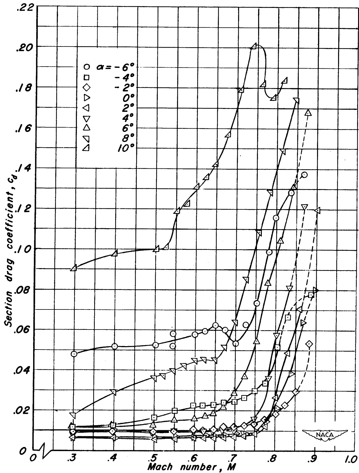
Figure 36.- The variation of section drag coefficient with Mach number at various angles of attack for the NACA 847A110 airfoil.
