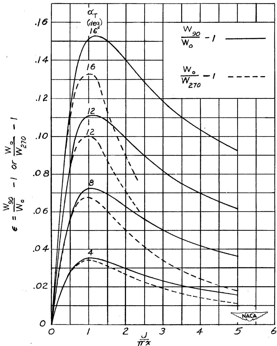
Figure 4.— Variation in fractional amplitude of resultant velocity.
