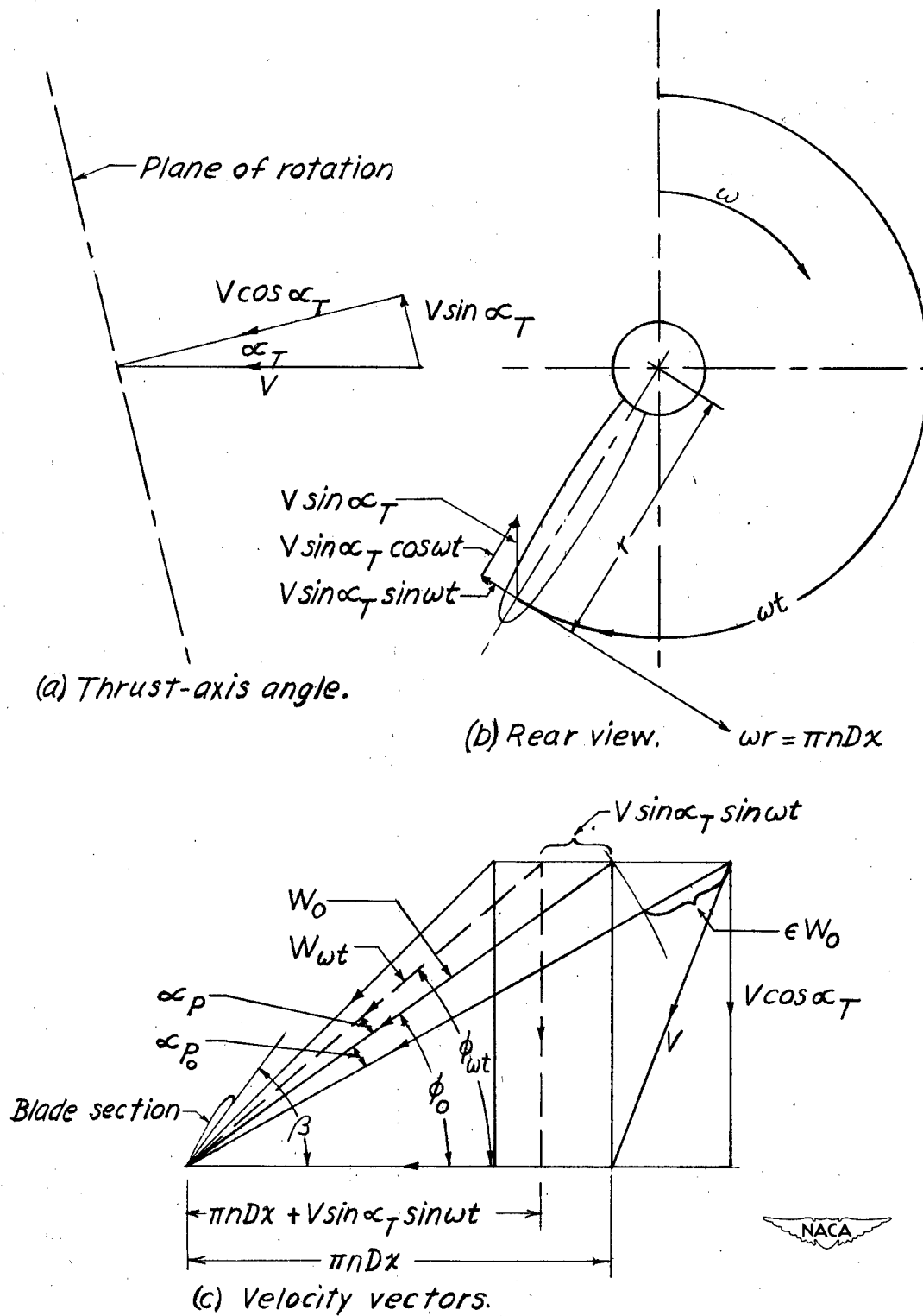
Figure 1.— Velocity diagram of inclined propeller.
