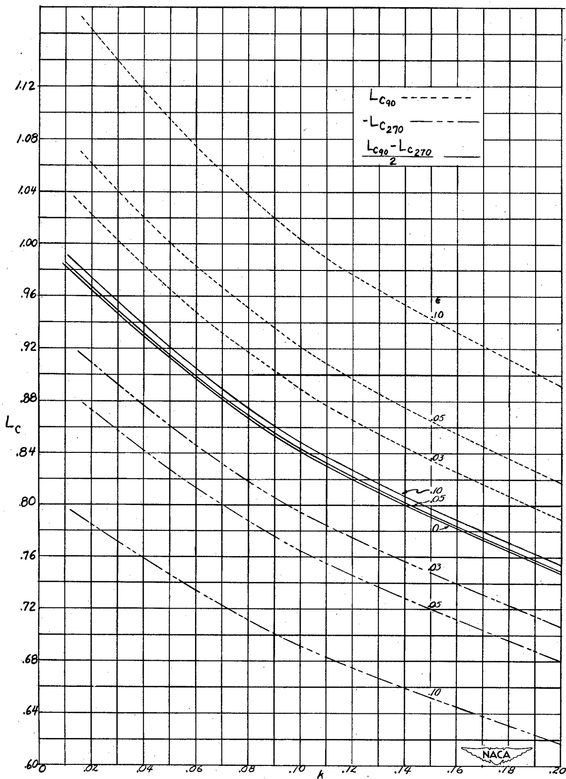
Figure 11.— Variation of force coefficient with k . \frac{\alpha}{\alpha_{P_0}} = 0 .
