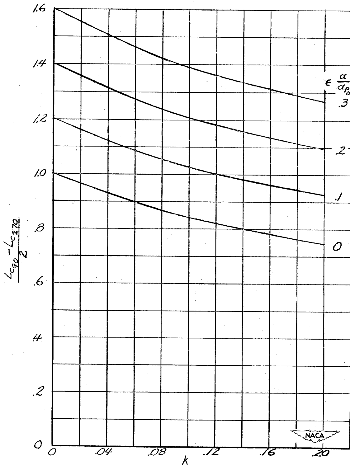
Figure 13.— Variation of force coefficient with k and with \epsilon \frac{\alpha}{\alpha_{p0}} . ( \epsilon < 0.1 ).
