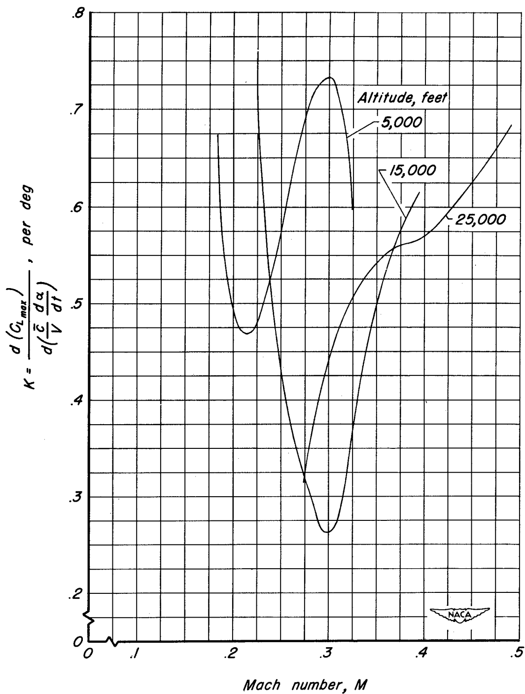
Figure 7.- Variation of K with change in Mach number for various altitudes.
