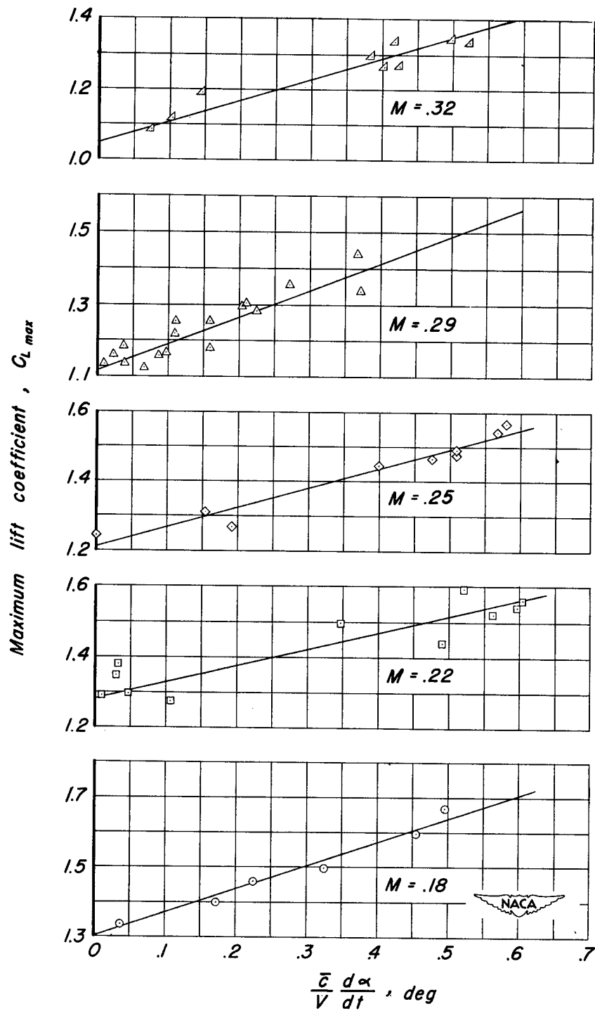
Figure 4.- The effect of rate of change of angle of attack on maximum lift coefficient at 5,000 feet altitude.
