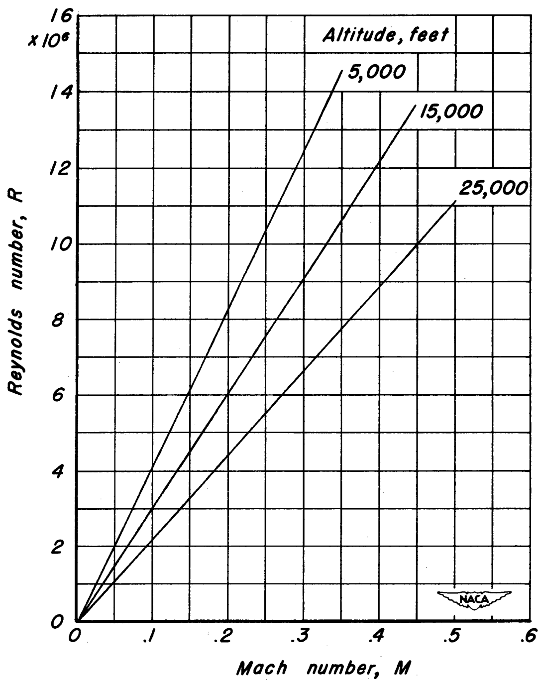
Figure 3.- Variation of Reynolds number with Mach number occurring during the flight tests.
