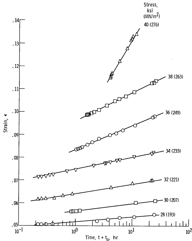
Figure 5. - Logarithmic creep of Mo-Ti-C alloy at 1800^\circ\text{F} ( 1255\text{ K} ). Time under given creep stress, 24 hours; change in stress during incremental creep test, 2 kips per square inch ( 14\text{ MN/m}^2 ).
