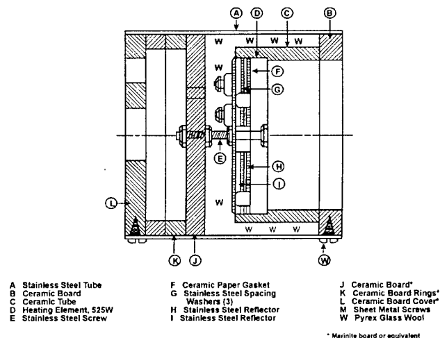
Figure 9-4. Furnace Details
