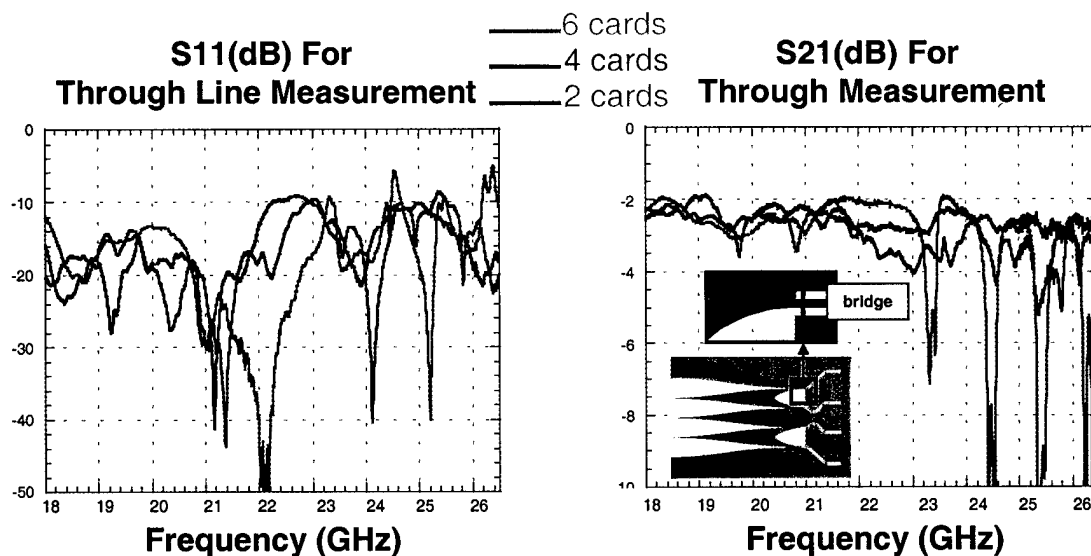
Figure 12 – Measurements on the passive combiner system using a through-line between input and output antennas.
