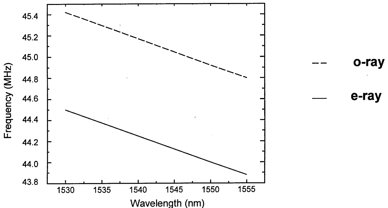
Figure 43 Measured Tuning Curve of EPIF
