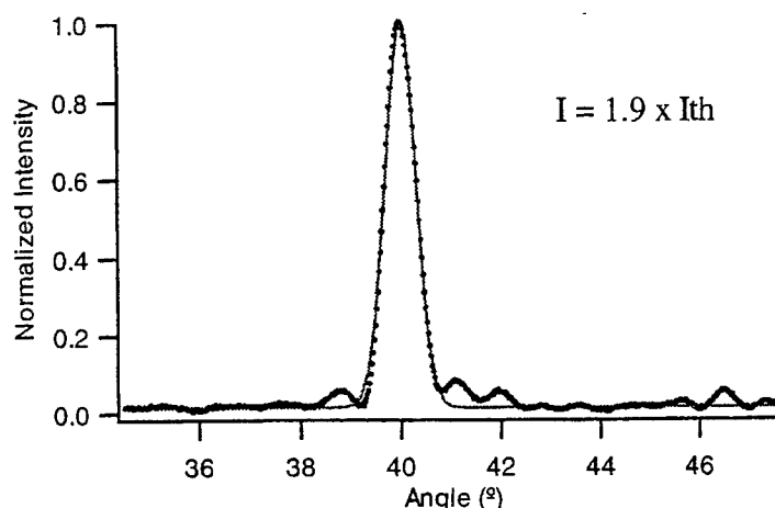
Figure 5: Far field pattern near 40° incidence for a 1:5 laser 800μm long and 200μm wide. The beam waist of 0.4° is 1.6 times the diffraction limit for a 200μm aperture. Dots are measured data, solid line is a gaussian fit.
