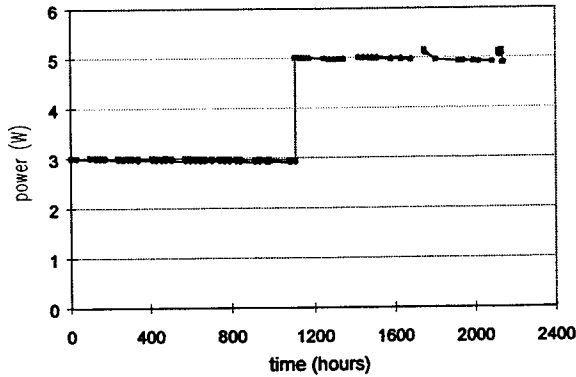
Figure 4. Constant-current lifetest of two 670-nm bars at 25 °C. Initial power was 3 W; after 1100 hours, power was increased to 5 W. Degradation was approximately 3% in 1000 hours at 5 W. (Discontinuities correspond to excursions in the cooling-water temperature.)
