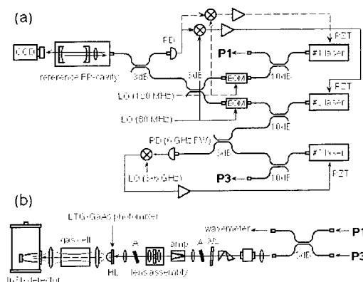
Figure 1: Schematic diagram of (a) the three DBR laser system that synthesizes a precise difference frequency, and (b) the MOPA system and the setup for spectroscopy.
