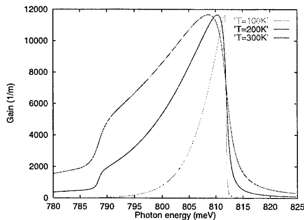
Fig. 2 Optical gain of the structure at various lattice temperatures ( T_L = 100\text{-}300 \text{ K} ). The threshold currents are J_{th} = 40 \text{ A/cm}^2 (100 K), J_{th} = 107 \text{ A/cm}^2 (200 K) and J_{th} = 180 \text{ A/cm}^2 (300 K).
