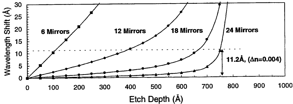
Fig. 2 Theoretical data from transmission line modeling showing the wavelength shift, \Delta\lambda as a function of etch depth into the top \lambda/2 GaAs phase matching layer. The position of the required etch depth for devices with \Delta n=0.004 is indicated. Results are shown for devices with 6, 12, 18 and 24 mirror pairs in the top DBR.
