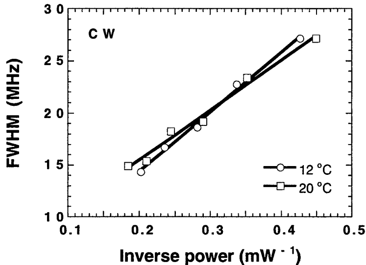
Fig. 3. Spectral linewidth of the DFB emission from an as-cleaved facet as a function of the facet output power.
