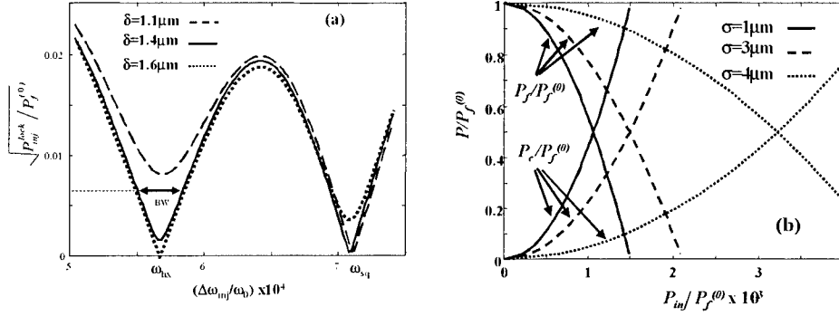
Fig. 3. Switching properties of the 10 \times 10 strained lattice of Fig. 2. (a) Square root of the normalized switching average power density P_{inj}^{lock} / P_f^{(0)} as a function of \Delta\omega_{inj}/\omega_0 for three different strain values of the lattice; and (b) The normalized free running P_f/P_f^{(0)} and driven P_c/P_f^{(0)} average power densities as a function of the normalized injected power density P_{inj}/P_f^{(0)} for three values of \sigma .
