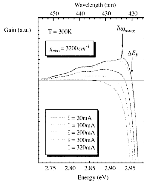
Figure 1: Gain/absorption spectrum of an InGaN MQW diode laser at different injection levels. Spectral position of laser emission and the quasi-Fermi level separation at threshold are shown.
