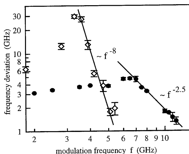
Fig. 2. Measured modulation efficiency in terms of the resulting frequency deviation for the VCSEL (circles) and an edge-emitting diode laser (diamonds). The data was obtained from the relative strengths of the carrier and the modulation sidebands.
