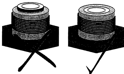
Figure 6: Correct positioning with the end of the transducer flush with the base of the thread adaptor.
