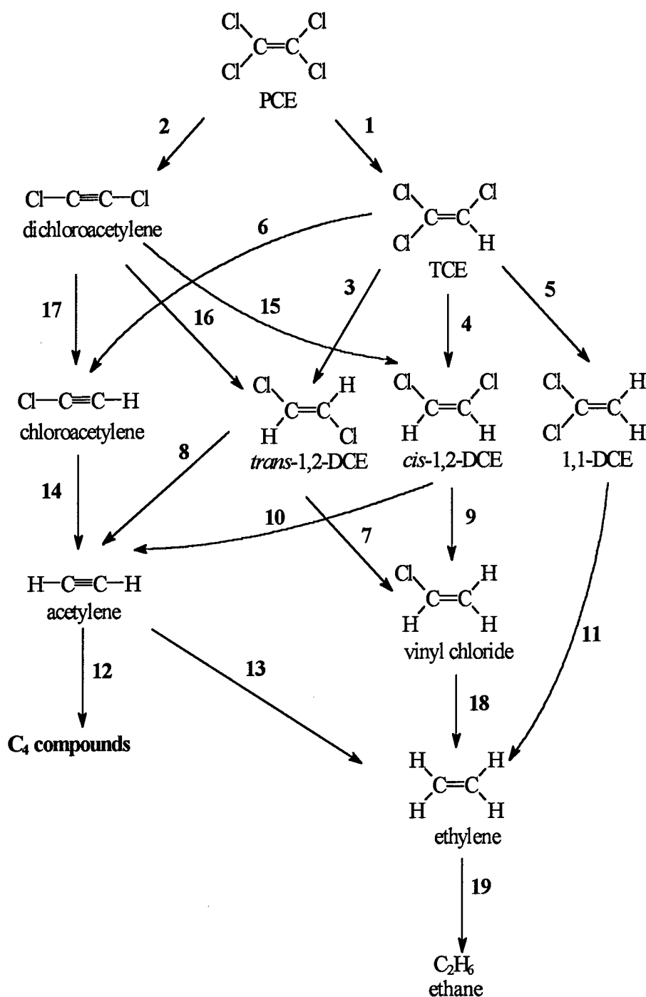
Figure 60. Hypothesized reaction pathways for the chlorinated ethylenes and other intermediates during reduction by Fe(0). Numbering corresponds to Table 10. Reactions 1, 3, 4, 5, 7, 9, 14, 17, and 18 correspond to hydrogenolysis reactions, while reactions 2, 6, 8, and 10 are reductive \beta -elimination reactions, reaction 11 results from reductive \alpha -elimination, and reactions 13, 15, 16, and 19 are hydrogenation reactions.
