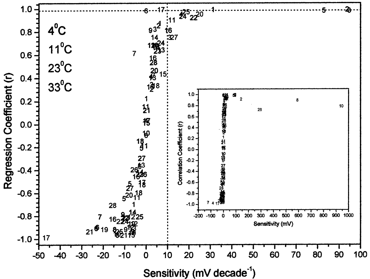
FIG. 28. The majority of biosensor test results for longevity experiments conducted between 4°C and 33°C fell between -50 and 100 \text{ mV decade}^{-1} sensitivity. Only three of the sensors fell within the criteria. Axes at 10 \text{ mV decade}^{-1} and 0.98 are the minimum acceptable criteria for a successfully performing biosensor. Inset: test results of all biosensors in immersion experiments. Biosensors for each experiment are shown by numerical designation.
