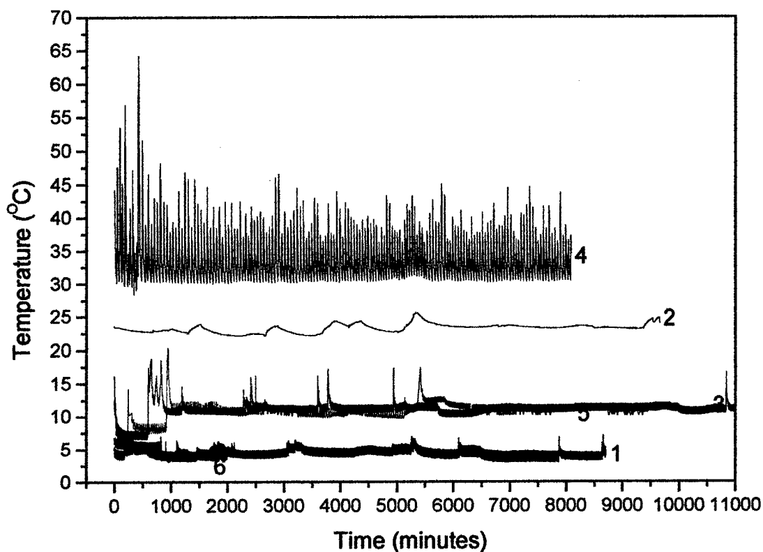
FIG. 22. Temperature monitoring of immersed biosensors during longevity experiments. 1. n = 8706 , mean = 4.38^{\circ}\text{C} ; 2. n = 9661 , mean = 23.23^{\circ}\text{C} ; 3. n = 15241 , mean = 11.02^{\circ}\text{C} ; 4. n = 8094 , mean = 33.72^{\circ}\text{C} ; 5. n = 9732 , mean = 10.72^{\circ}\text{C} ; 6. n = 2127 , mean = 4.73^{\circ}\text{C} (experiment 2). The incubator's (4) large deviation is a result of the instability of the temperature control apparatus.
