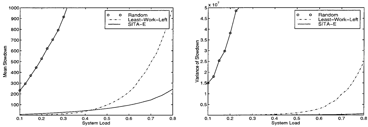
Figure 3: Experimental comparison of task assignment policies which balance load for a system with 4 hosts.
