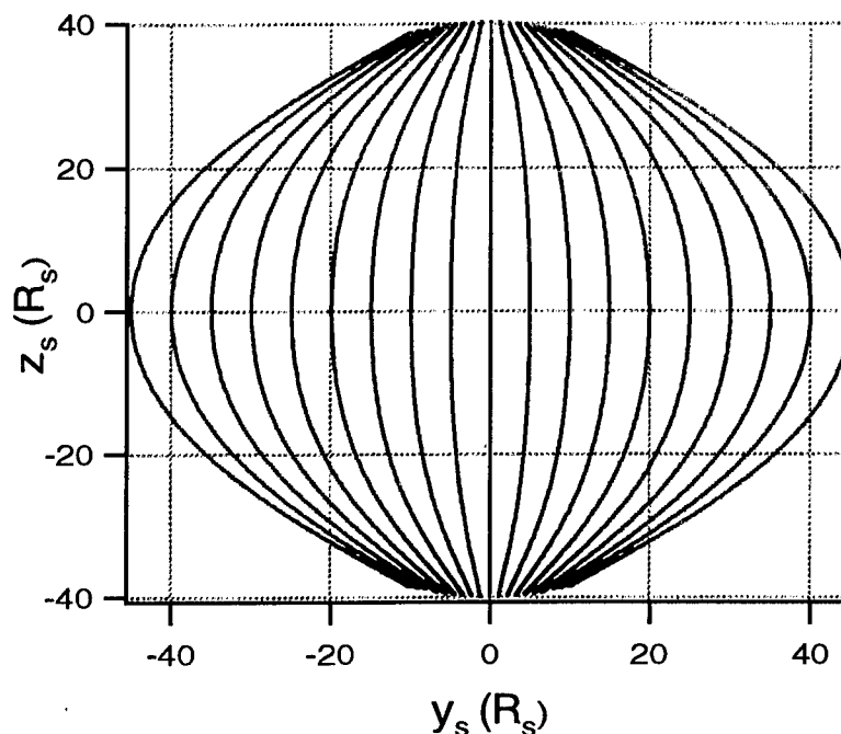
Figure 11. Projection of the magnetotail magnetic field for Saturn in the y-z plane. The coordinate system is centered on the planet with the x-y plane parallel to the magnetic equator and the z axis aligned with the magnetic dipole axis of Saturn. Notice the ellipsoidal characteristics of the Saturnian magnetotail due to the transformation via equation (31).
