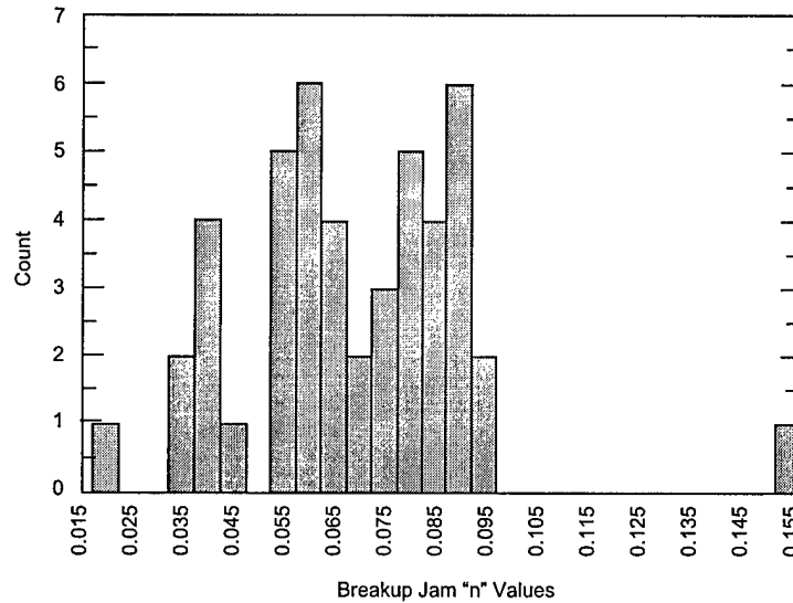
a. Distribution of Manning's n values for the underside of the ice from calibrated numerical models of breakup ice jams at three sites.
