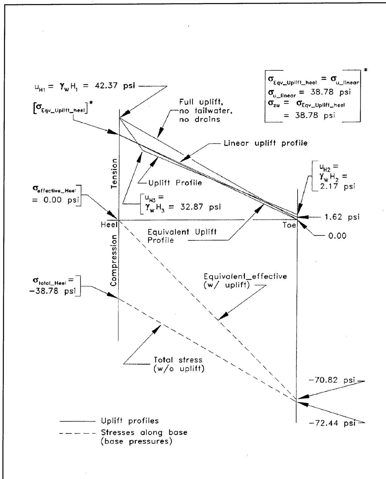
Figure 33. Reservoir elevation H_1 = 97.62 \text{ ft} resulting in \sigma_{total\_Heel} equal to \sigma_{zu} using Reclamation criteria (1 ft = 0.305 m, 1 psi = 6.894 kPa)
