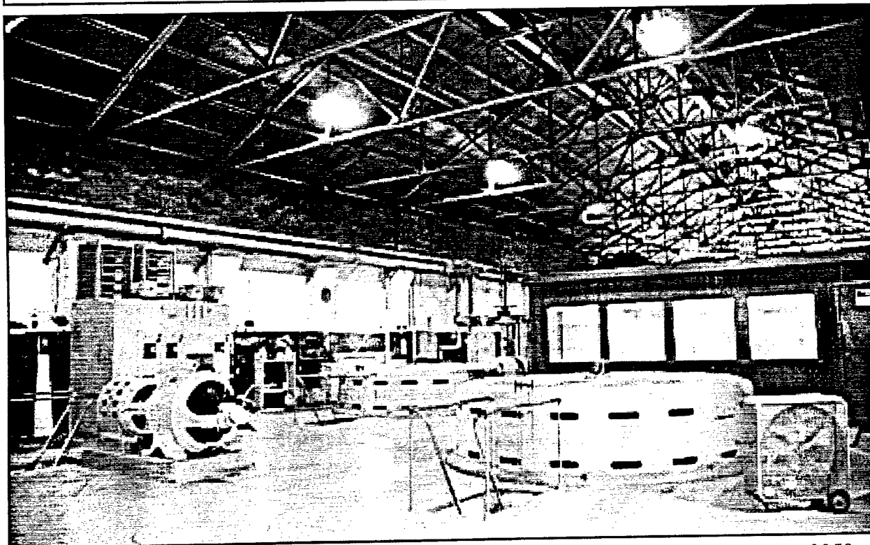
Figure 64. Drainage Pumping Station No. 7. View of interior, showing motor covers of 250 cfs centrifugal "flathead" pumps.
