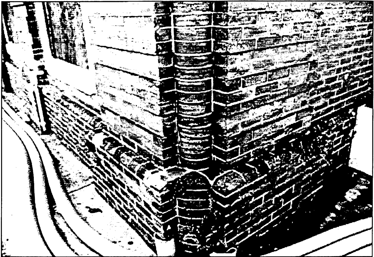
Figure 92. Drainage Pumping Station No. 1. View of lower portion of northwest corner of building, showing special round bricks and pilaster bases at corner.
