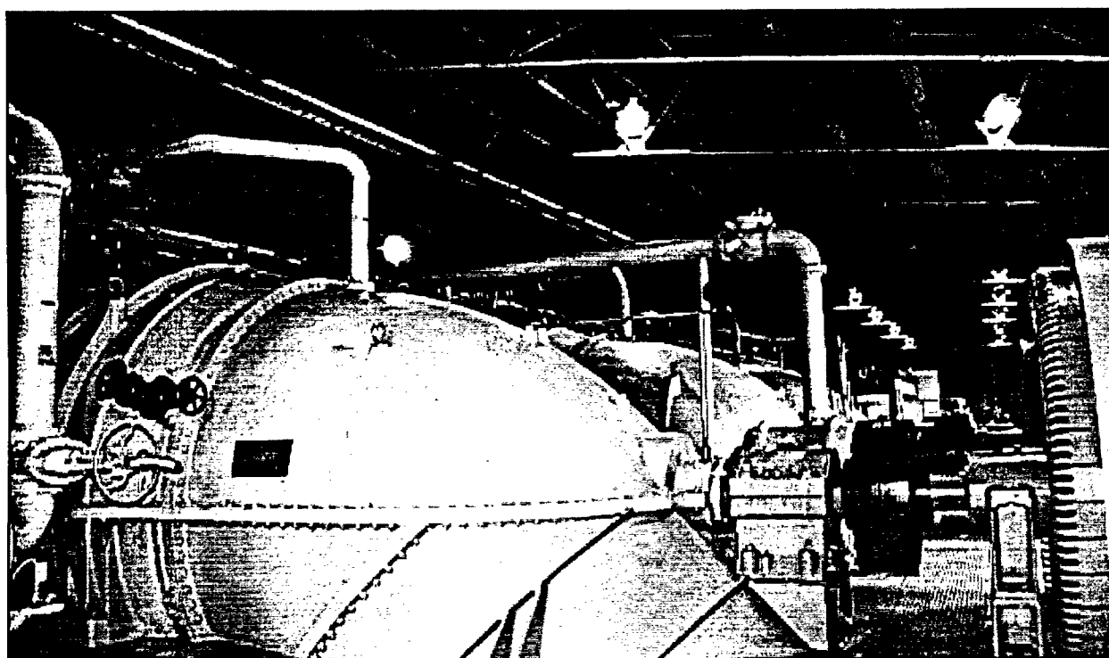
Figure 37. Drainage Pumping Station No. 1. View of interior looking south from central portion of building. Foreground, prototype Wood screw pump on display; center, 250 cfs vertical screw pump motors.
