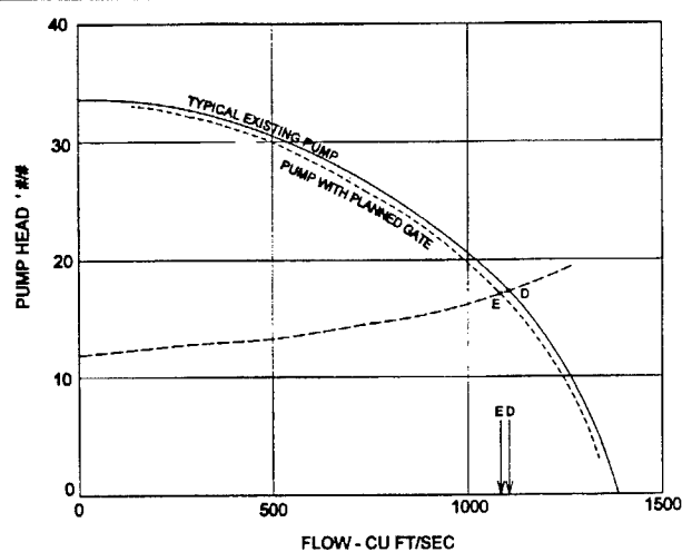
Figure 114. Pump flow rates of existing pump and pump with planned fronting protection sluice gates.
