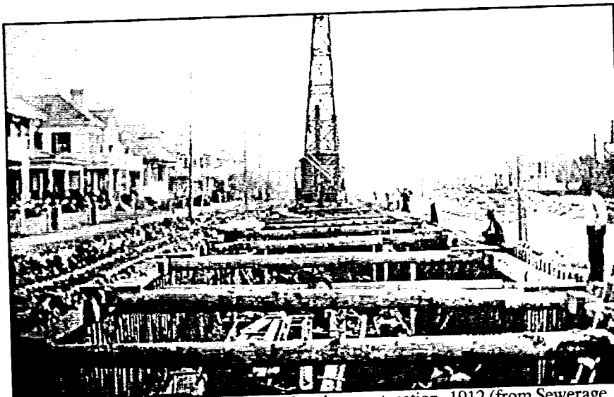
Figure 73. Napoleon Avenue Canal under construction, 1912 (from Sewerage & Water Board, 1912).
