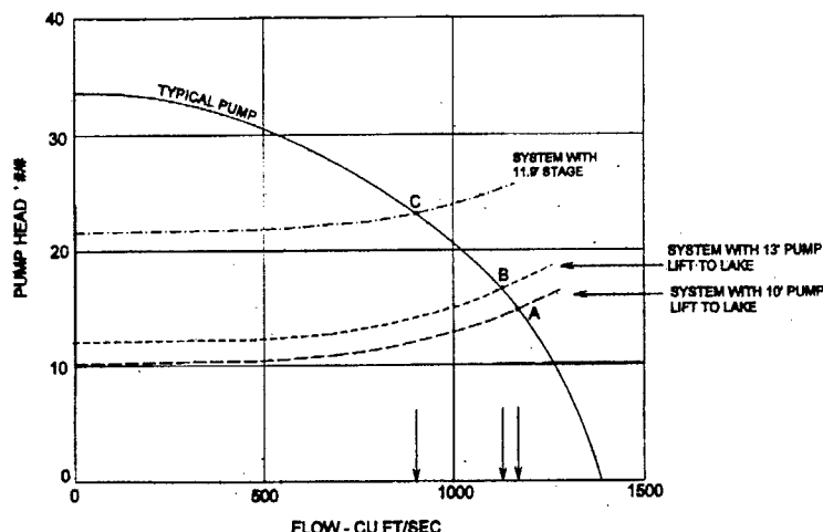
Figure 113. Suction and discharge head levels versus flow rate.
