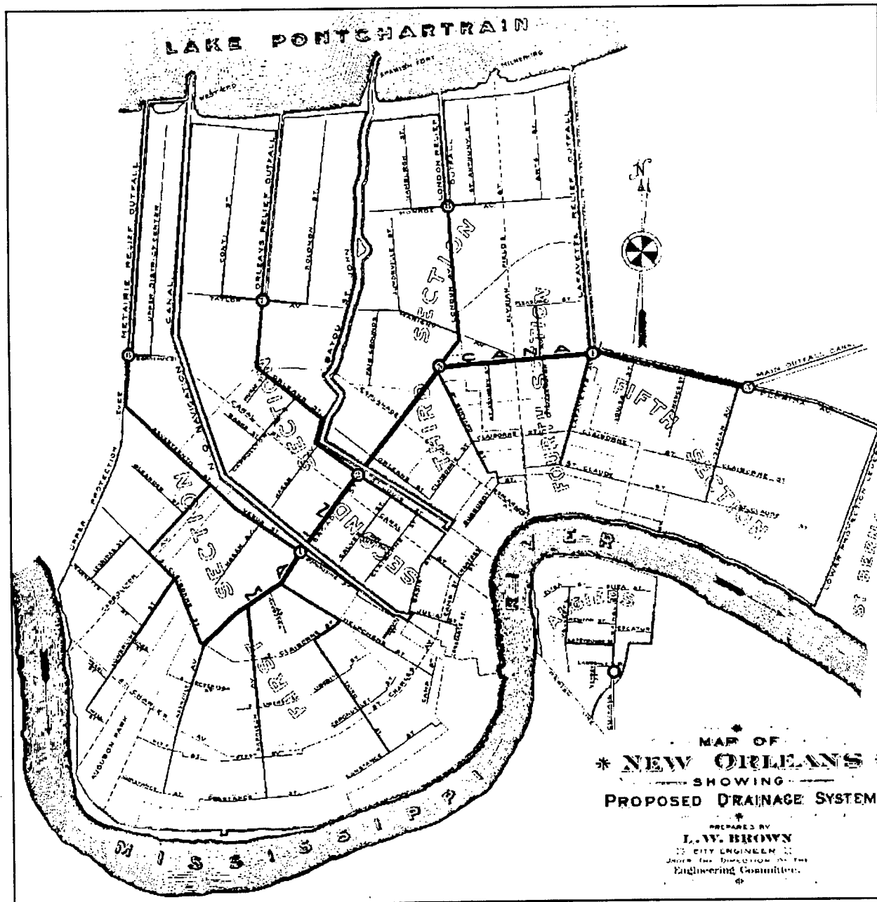
Figure 6. The New Orleans Drainage System as proposed in the 1895 Drainage Plan (from Fitzpatrick et al. 1895).
