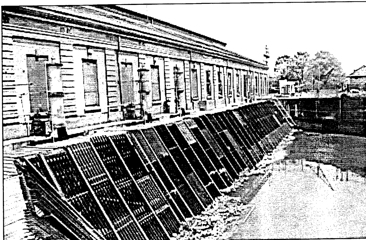
Figure 63. Drainage Pumping Station No. 7. Viewed from the northeast, showing trash screen and hydraulic sluice gate mechanisms.
