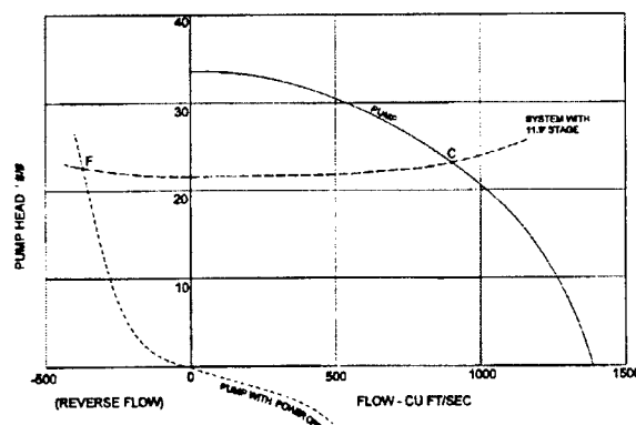
Figure 115. Effect of reverse flow.
