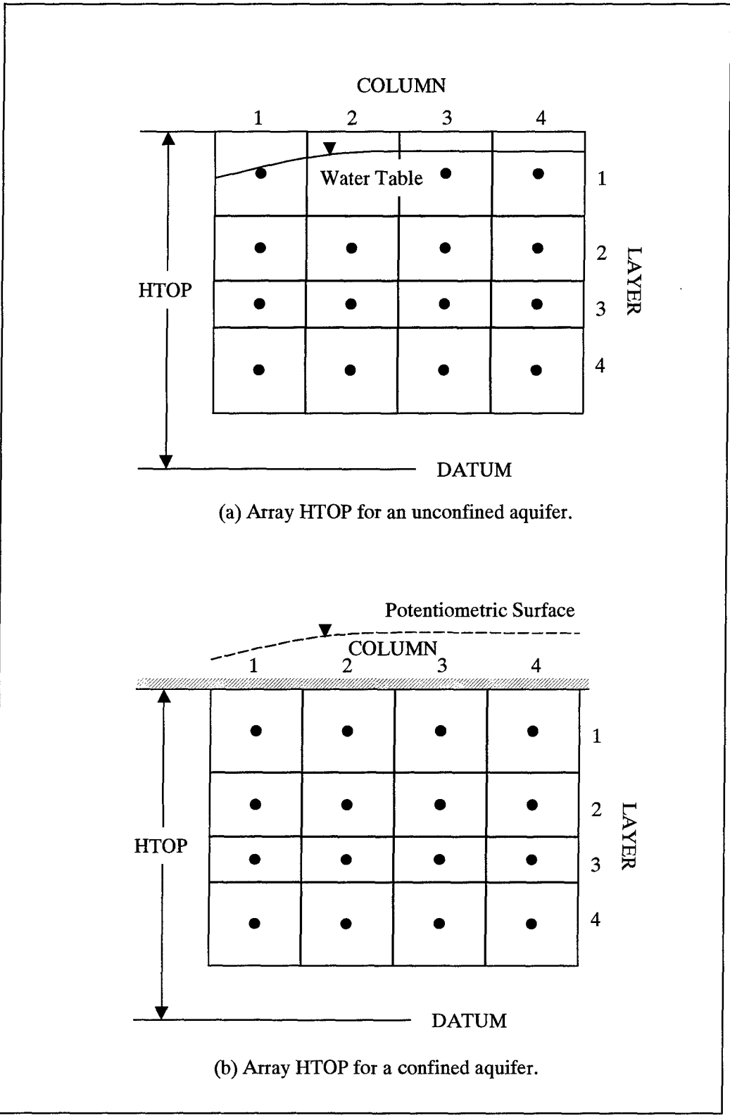
Figure 27. Illustration of array HTOP for (a) unconfined and (b) confined aquifer layers
