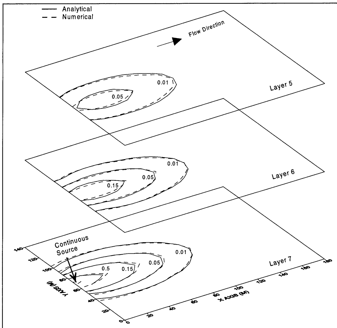
Figure 39. Comparison of the analytical and numerical solutions for three-dimensional transport from a continuous point source in a uniform flow field
