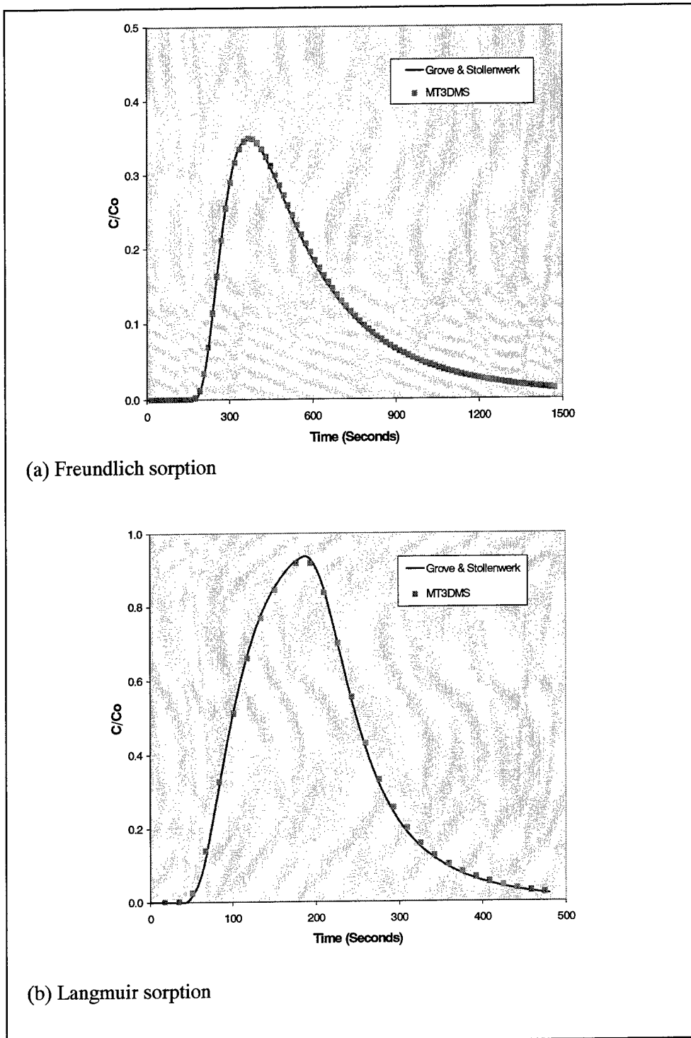
Figure 33. Comparison between the numerical solutions of MT3DMS and those based on Grove and Stollenwerk (1984) for one-dimensional transport involving nonlinear (a) Freundlich and (b) Langmuir sorption isotherms
