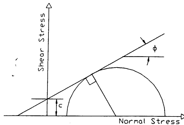
Figure 2.1 Mohr's Circle
