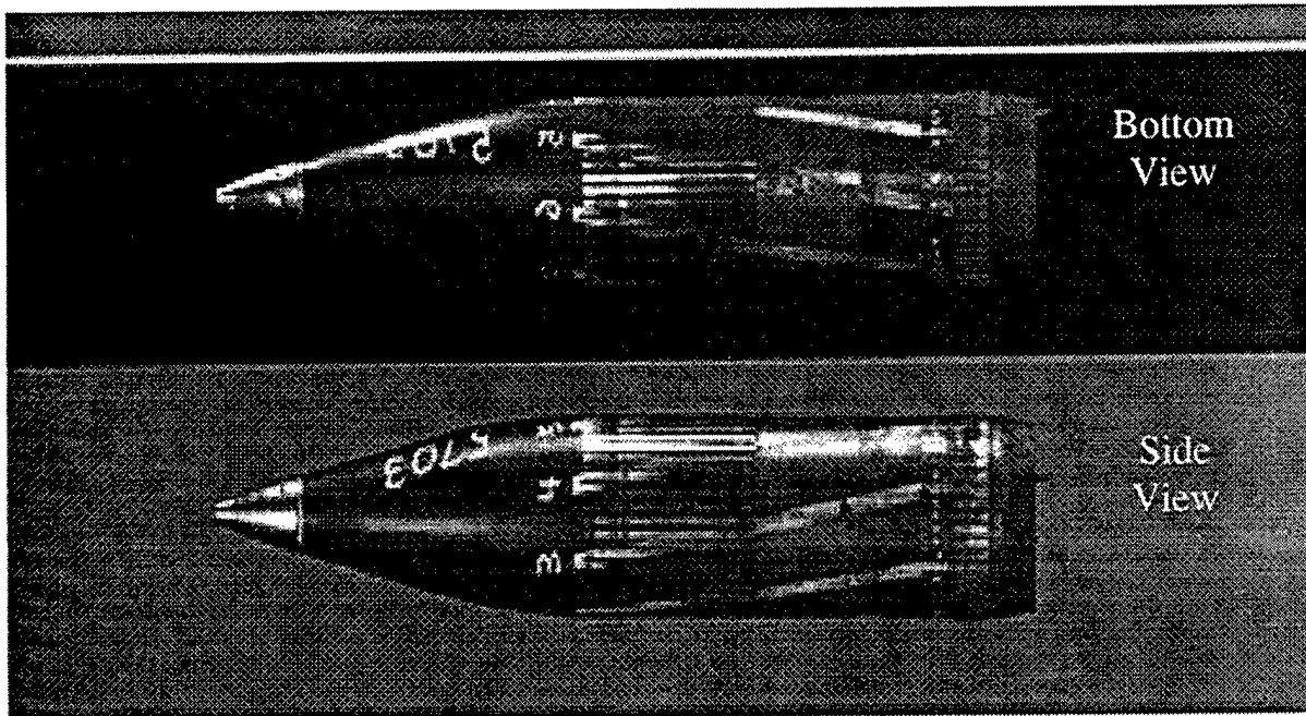
Figure 3. Typical M898 Smear Photograph.
