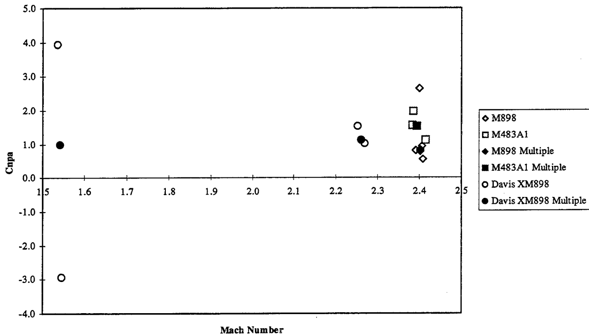
Figure 8. C_{np\alpha} vs. Range.
