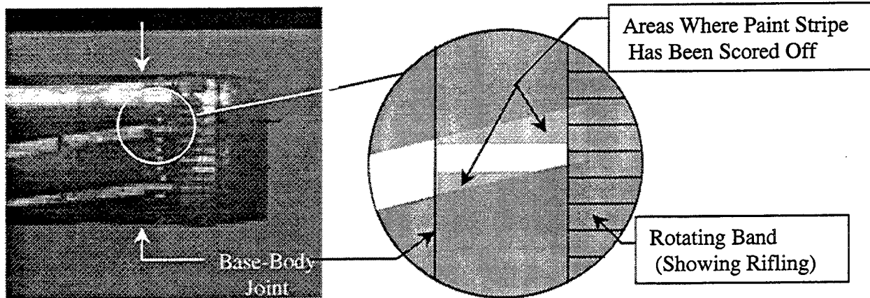
Figure 4. Expanded View of Base-Body Joint.
