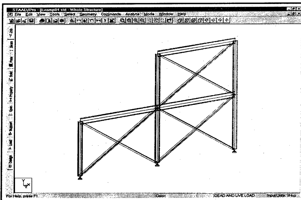
Figure 6. Plane frame (3).
