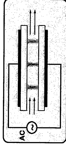
Silent discharge (dielectric-barrier discharge)
