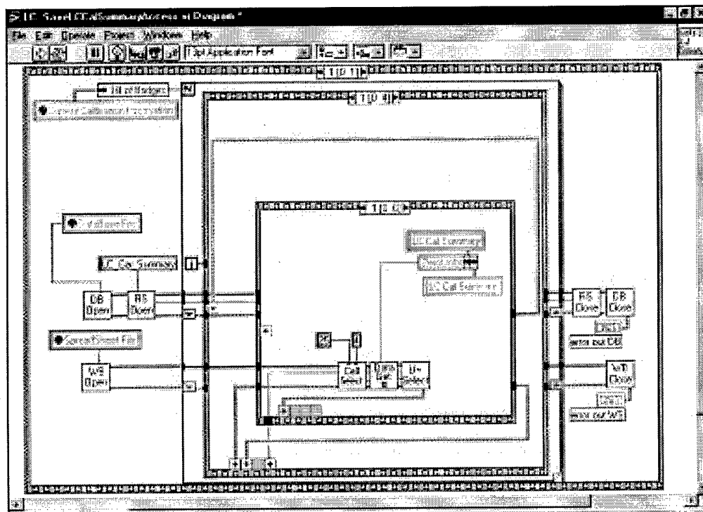
Figure 6. Block Diagram of Reading Excel Data and Writing Data to Access
