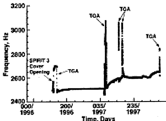
Figure 6. CQCM frequency versus time since launch.
