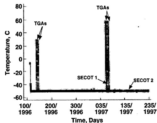
Figure 12. Temperature versus time for TQCMs 2-4 since launch.
