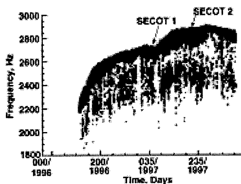
Figure 8. TQCM #1 plot showing increase in frequency due to accreted mass at (+Y,+Z) location.
