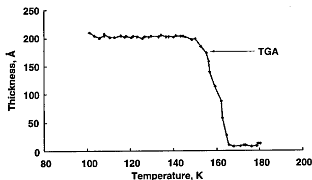
Figure 13. Plot of CQCM film thickness versus temperature TGA performed after accretion during SECOT 1 solar heating experiment.
