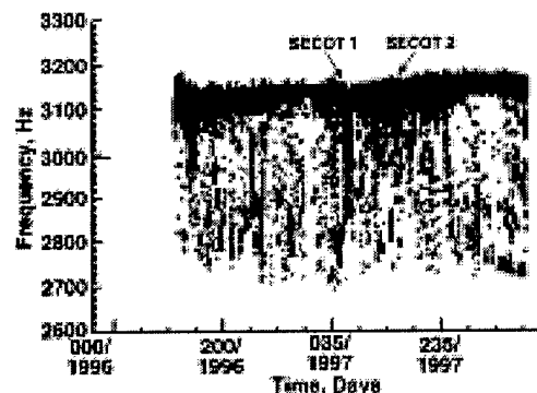
Figure 10. TQCM #3 plot showing increase in frequency due to accreted mass at (+Y, -Z) location.
