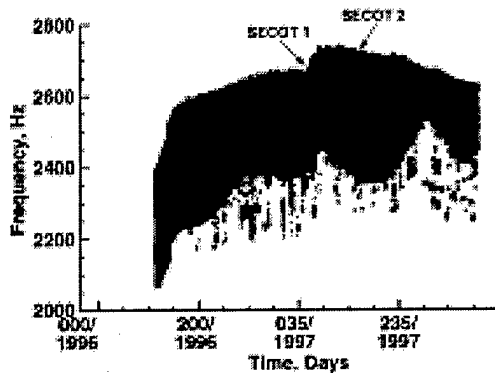
Figure 11. TQCM #4 plot showing increase in frequency due to accreted mass at (+X) location.
