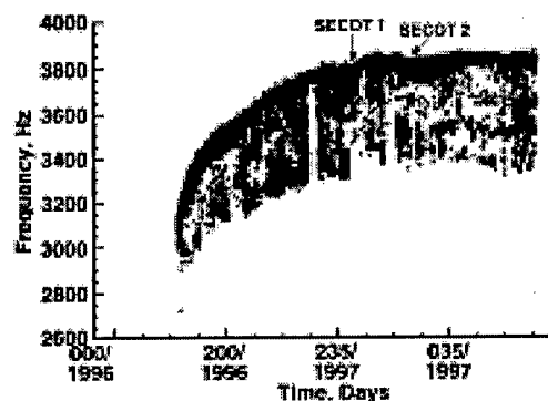
Figure 9. TQCM #2 plot showing increase in frequency due to accreted mass at (+Z) location.
