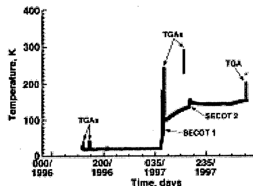
Figure 7. CQCM temperature versus time since launch.
