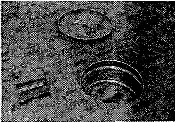
Buried powder keg target with top removed [12]
