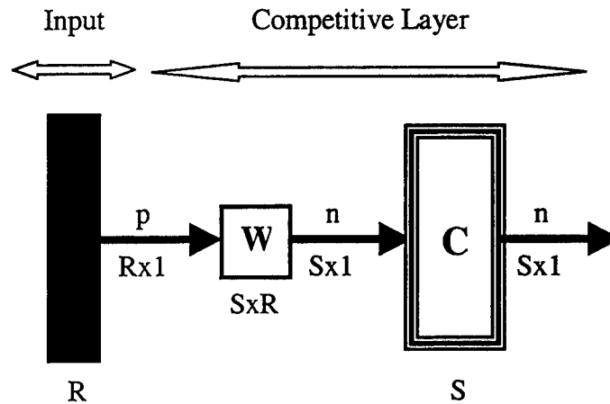
Figure 3.2 Competitive Neural Network
