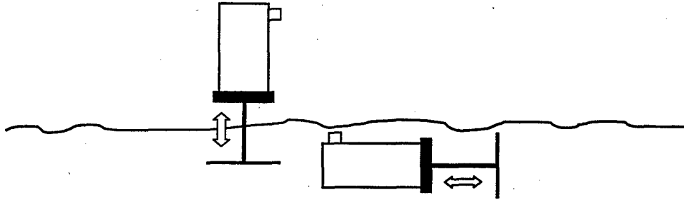
Figure 4.1 Actuator placement for Rayleigh waves generation [11].
