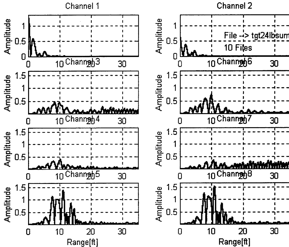
8-Channel data plot of the received signals. Channels 1 and 2 come from the accelerator meters. Channels 3, 4, 5 represent the x, y, z motion of the 1 st geophone, and channels 6, 7, 8 the x, y, z motion of the 2 nd geophone.
