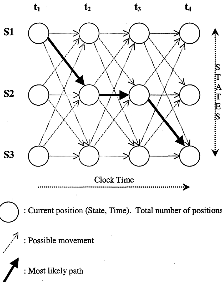
Figure 2.4a Trellis Diagram for T=4 , and N=3 , ergotic model
