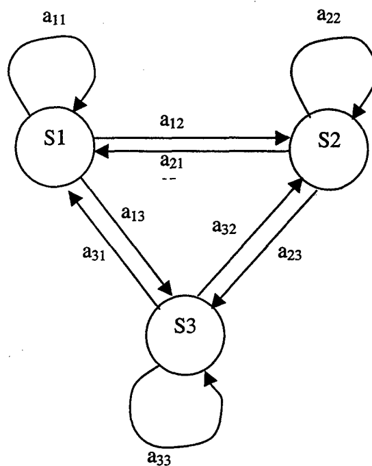
Figure 2.2 A Markov Process (Chain), ergotic model
