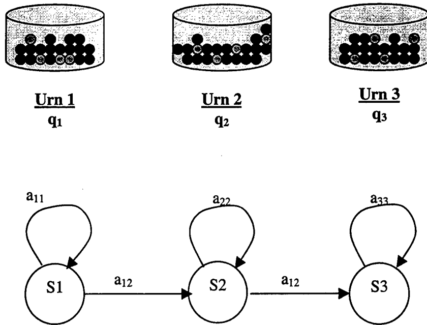
Figure 2.3. The classic Urn-ball example. There are three ( N=3 ) urns that contain a large number of color balls. The colors of the balls are red, green, and blue. The boy we assigned to paint the balls runs out of blue paint sometime while painting and uses sky blue afterwards. Thus, eventhough there are 4 colors, we assign the same symbol for blue and sky blue and the number of symbols is three ( M=3 ). Each time a person randomly selects an urn, he selects a ball, and announces the color. The process is repeated 4 ( T=4 ) times. Note that: 1) we don't know from which urn the ball came from, as we only have a color sequence, and we map those colors with the symbols according from Table, 2.2; 2) we assume that it is a left-to-right model for simplicity.
