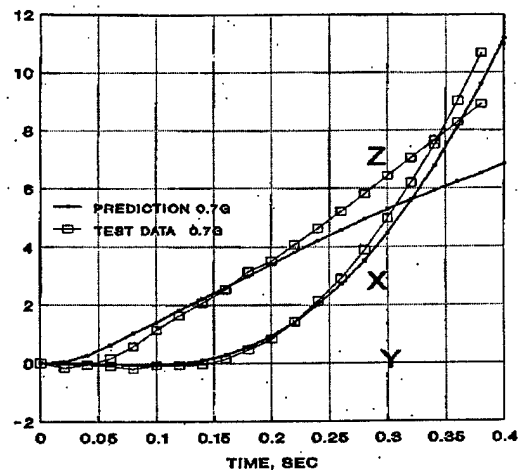
Figure 15 F-14/AIM-7 Trajectory
