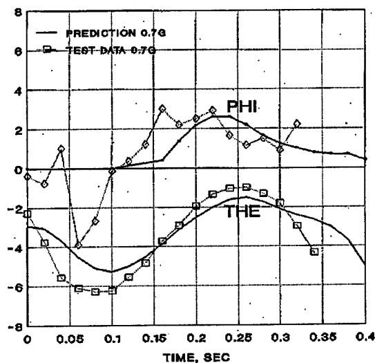
Figure 14. F-14/AIM-7 Trajectory
