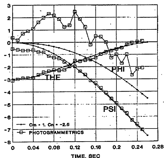
Figure 12. GBU-24/F-14 Station 5 Trajectory
