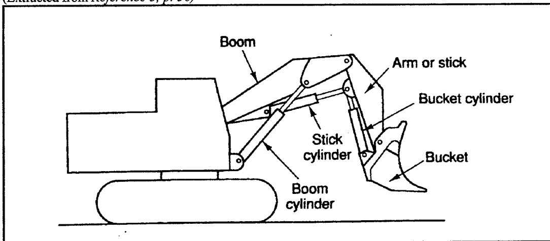
Figure 6-1 Front Shovel Components (Extracted from Reference 3, p. 50 )
