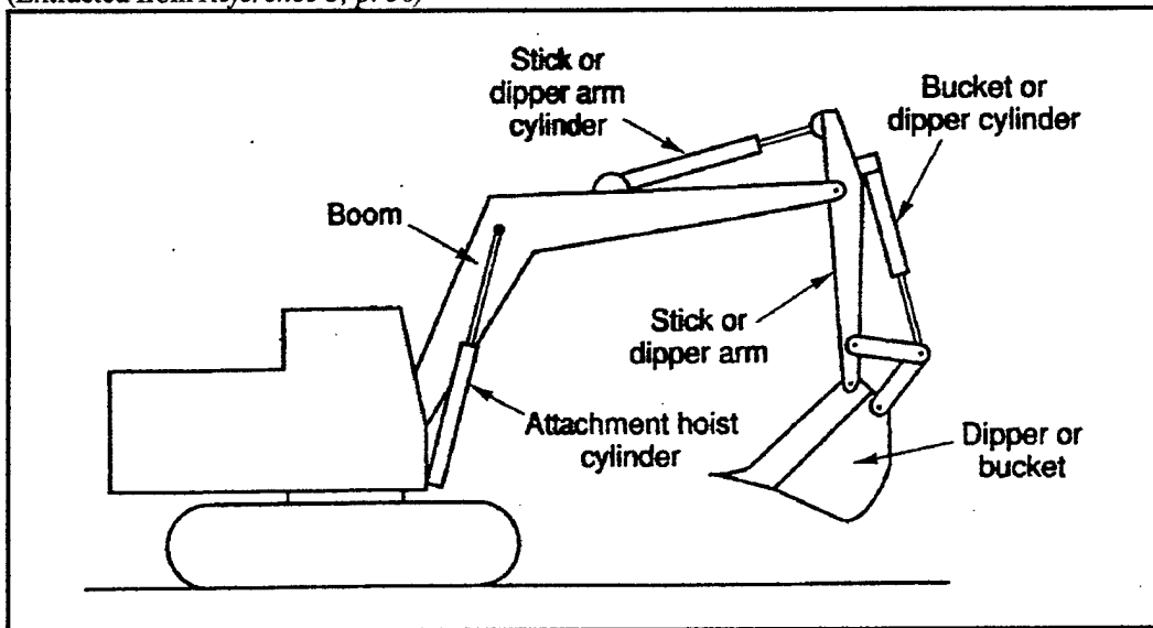
Figure 6-5 Backhoe Components (Extracted from Reference 3, p. 58 )
