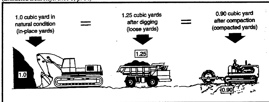
Figure 4-1, Typical Volume Change During Earthmoving (Extracted from Reference 3, p. 30 )
