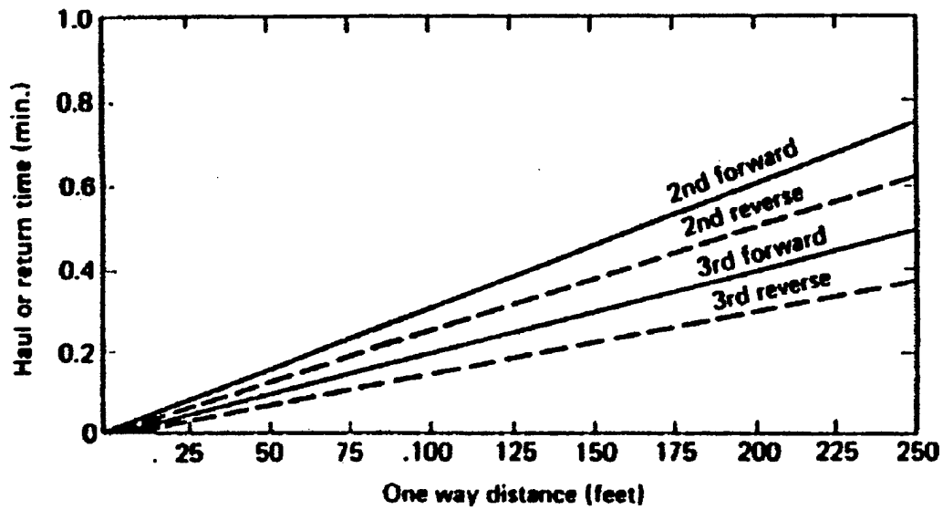
Figure 8-4 Track loader travel time (Extracted from Reference 4, p. 56 )
