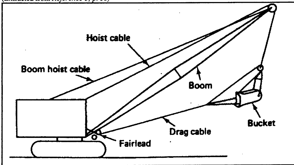
Figure 6-6 Dragline Components (Extracted from Reference 3, p. 53 )
