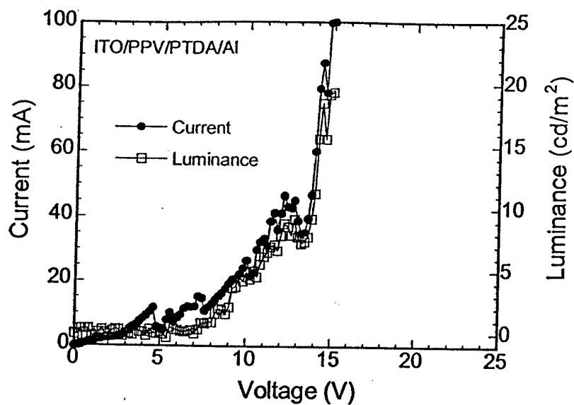
Figure S18. Current-voltage and luminance-voltage characteristics of the ITO/PPV(35 nm)/PTDA(25 nm)/Al diode.
