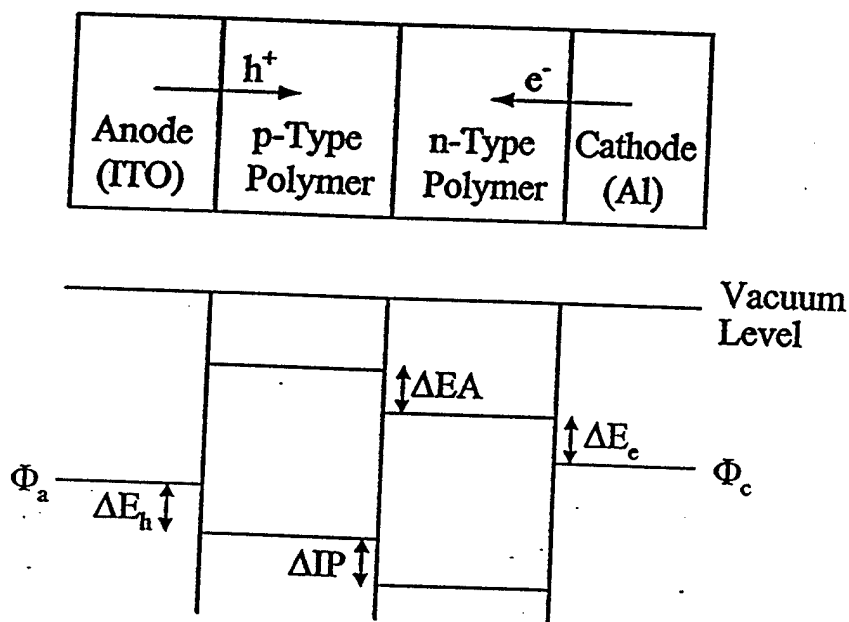
(b) Two-layer Heterojunction LED
