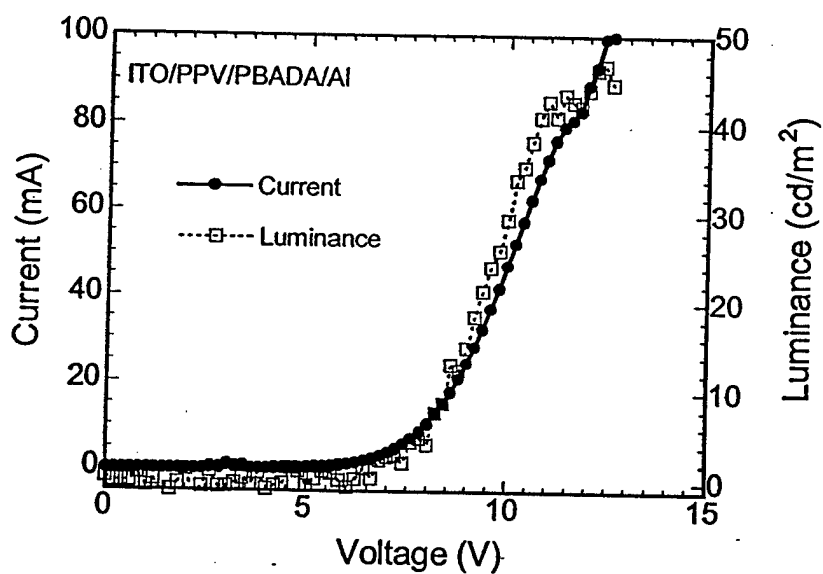
Figure S15. Current-voltage and luminance-voltage characteristics of the ITO/PPV(35 nm)/PBADA(20 nm)/Al diode.
