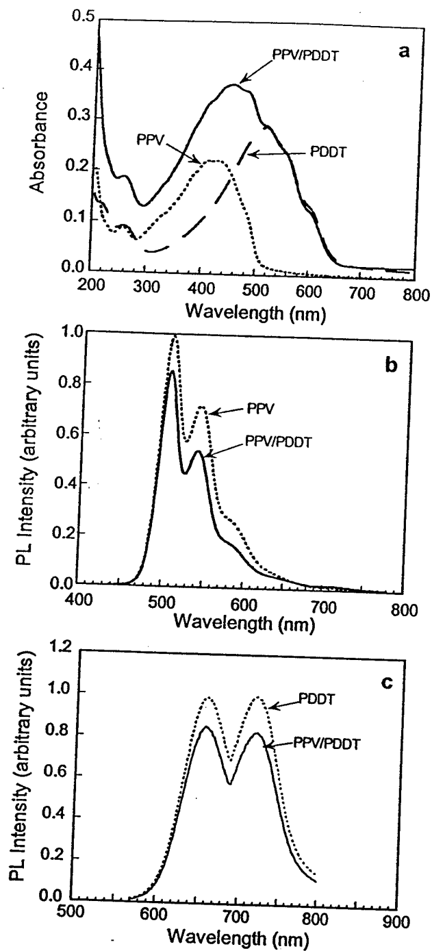
Figure S7. (a) Optical absorption spectra of PDDT, PPV, and PDDT/PPV thin films. (b) PL spectra of PPV and PDDT/PPV thin films excited at 400 nm. (c) PL spectra of PDDT and PDDT/PPV thin films excited at 580 nm.
