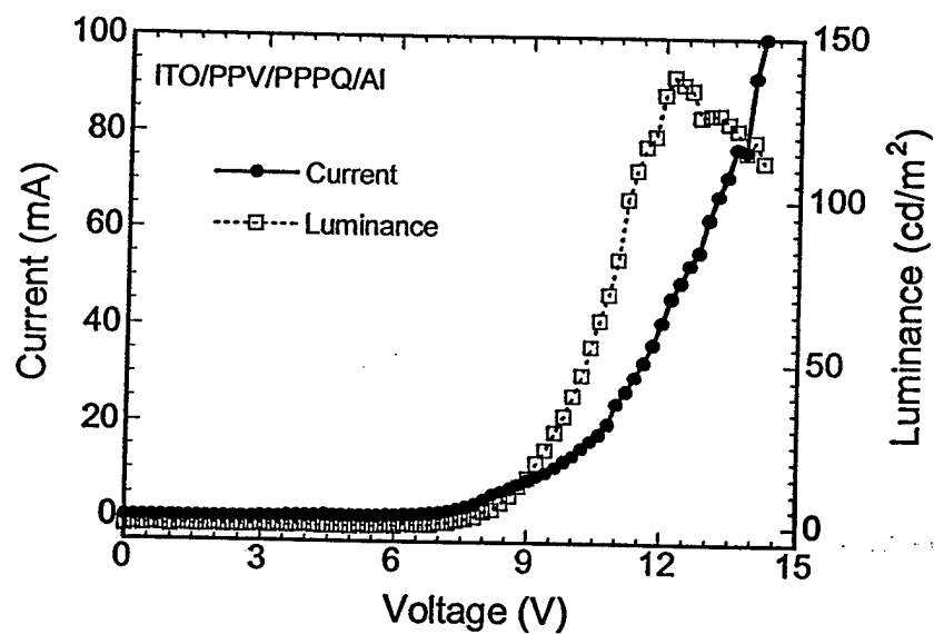
Figure S9. Current-voltage and luminance-voltage characteristics of the ITO/PPV(35 nm)/PPPQ(30 nm)/Al diode.
