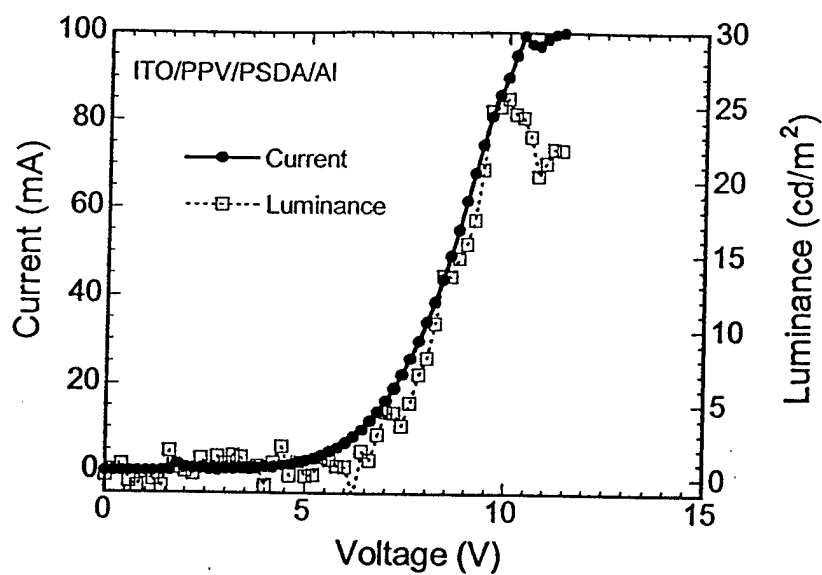
Figure S16. Current-voltage and luminance-voltage characteristics of the ITO/PPV(35 nm)/PSDA(25 nm)/Al diode.
