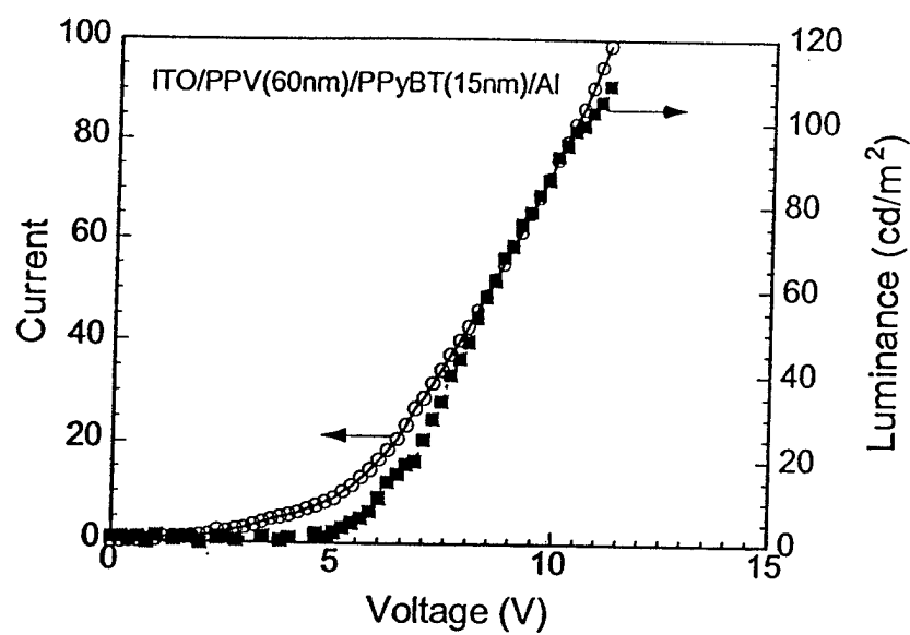
Figure S20. Current-voltage and luminance-voltage characteristics of the ITO/PPV(60 nm)/PPyBT(15 nm)/Al diode.
