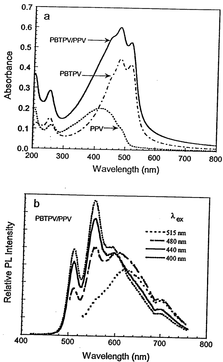
Figure S2. (a) Optical absorption spectra of PBTPV, PPV and PBTPV/PPV films. (b) PL spectra of the PBTPV/PPV film with different excitation wavelength.
