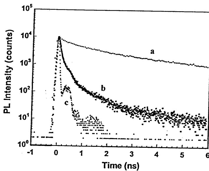
Figure S6. Time-resolved PL decay dynamics of PPQ (a) and PDDT/PPQ (b) thin films. Both PPQ and PDDT/PPQ thin films were excited at 380 nm, and the emission was monitored at 580 nm. The curve c represents the instrument response.
