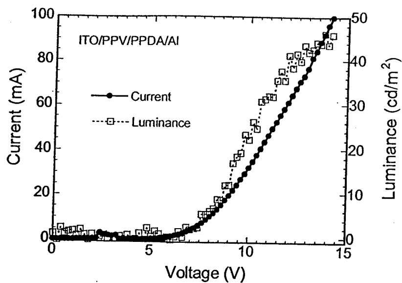
Figure S14. Current-voltage and luminance-voltage characteristics of the ITO/PPV(35 nm)/PPDA(20 nm)/Al diode.
