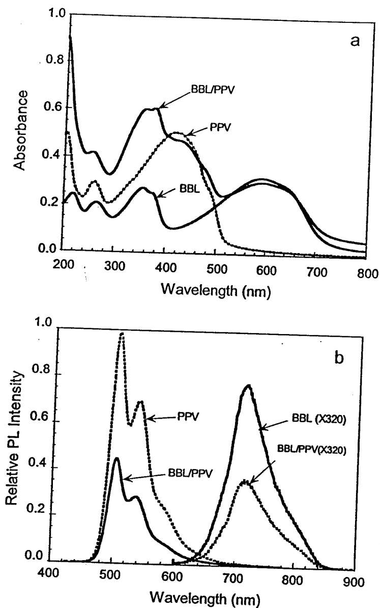
Figure S3. Optical absorption (a) and photoluminescence (b) spectra of BBL, PPV and PPV/BBL films. PPV was excited at 400 nm; BBL was excited at 580 nm; the bilayer PPV/BBL was excited at both 400 and 580 nm. The spectra excited at 580 nm were enlarged 320 times compared to spectra excited at 400 nm.
