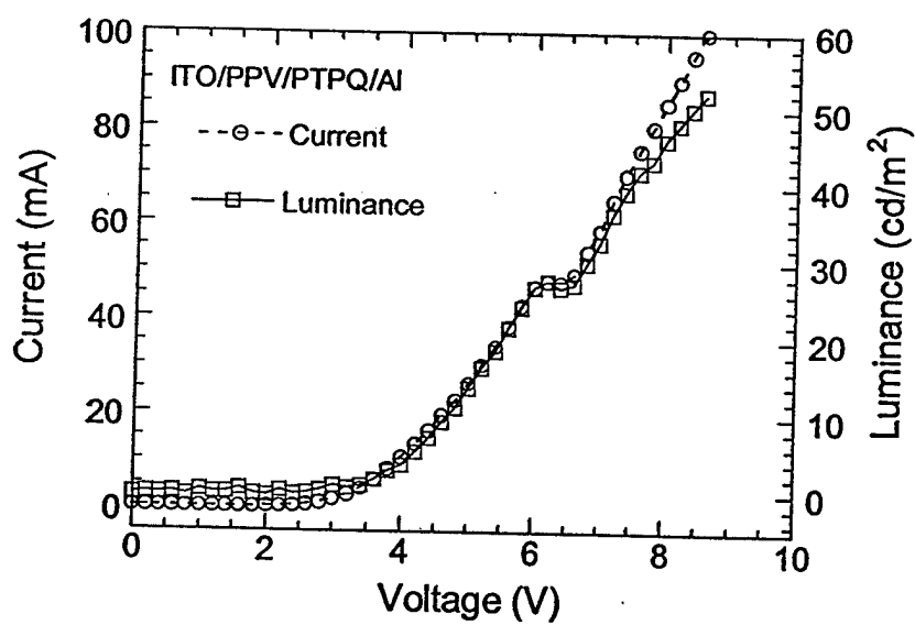
Figure 13. Current-voltage and luminance-voltage characteristics of the ITO/PPV(35 nm)/PTPQ(40 nm)/Al diode.
