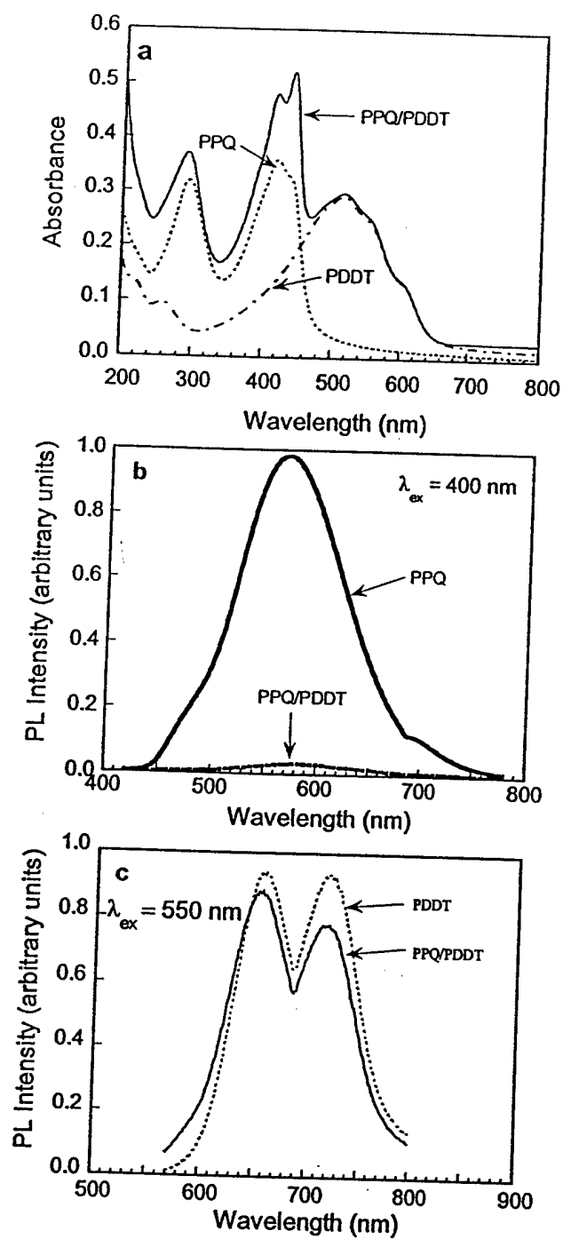
Figure S5. (a) Optical absorption spectra of PPQ, PDDT, and PDDT/PPQ thin films. (b) PL spectra of PPQ and PDDT/PPQ thin films excited at 400 nm. (c) PL spectra of PDDT and PDDT/PPQ thin film excited at 550 nm.
