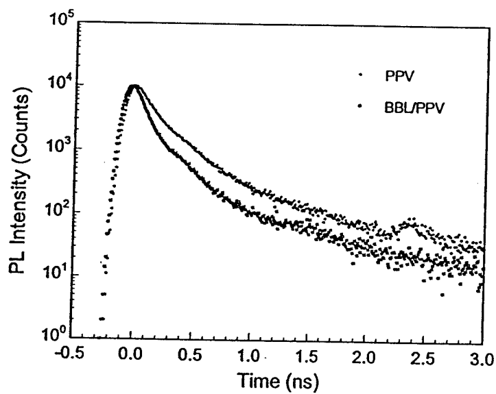
Figure S4. Time-resolved photoluminescence decay dynamics of PPV/BBL and PPV films. Both PPV and PPV/BBL films were excited at 420 nm, and the emission was monitored at 540 nm.
