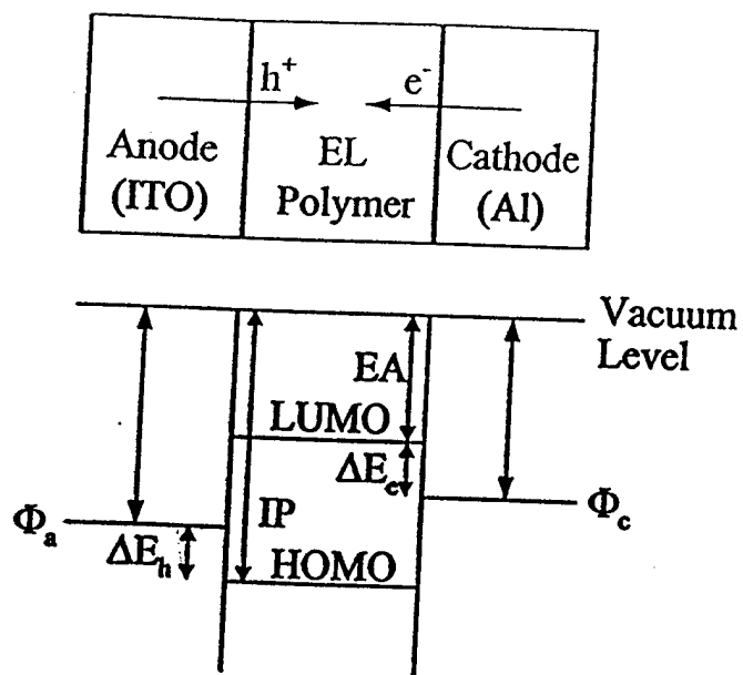
(a) Single-layer LED
