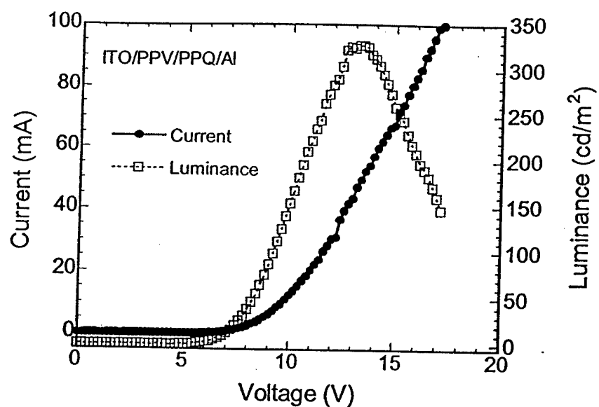
Figure S8. Current-voltage and luminance-voltage characteristics of the ITO/PPV(35 nm)/PPQ(35 nm)/Al diode.
