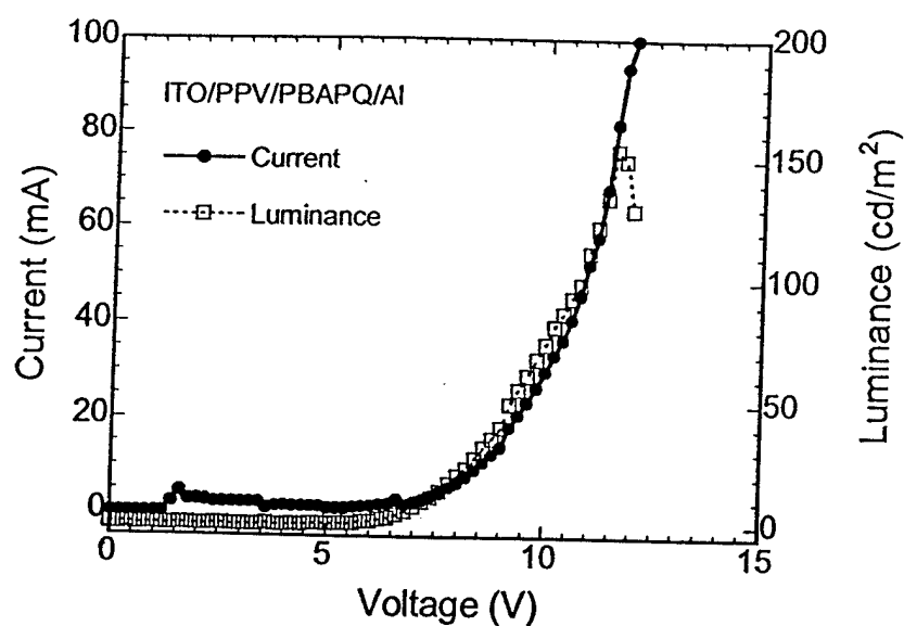
Figure S10. Current-voltage and luminance-voltage characteristics of the ITO/PPV(35 nm)/PBAPQ(35 nm)/Al diode.
