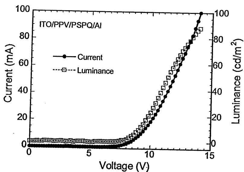
Figure S11. Current-voltage and luminance-voltage characteristics of the ITO/PPV(35 nm)/PSPQ(35 nm)/Al diode.
