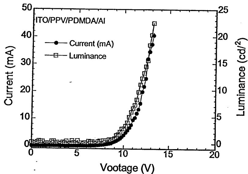
Figure S17. Current-voltage and luminance-voltage characteristics of the ITO/PPV(35 nm)/PDMDA(25 nm)/Al diode.
