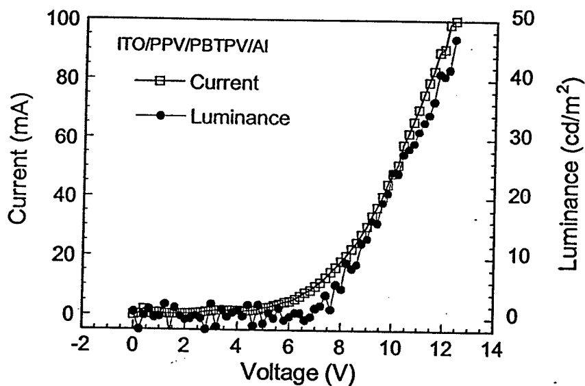
Figure S19. Current-voltage and luminance-voltage characteristics of the ITO/PPV(60 nm)/PBTPV(15 nm)/Al diode.
