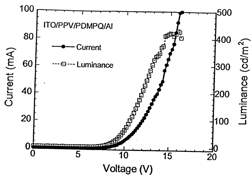
Figure S12. Current-voltage and luminance-voltage characteristics of the ITO/PPV(35 nm)/PDMPQ(30 nm)/Al diode.
