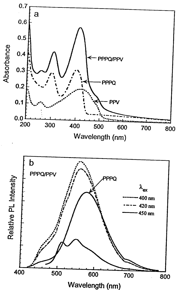
Figure S1. (a) Optical absorption spectra of PPPQ, PPV and PPPQ/PPV thin films. (b) PL spectra of the PPPQ/PPV thin film with different excitation wavelengths. The PL spectrum of PPPQ (excited at 400 nm) was also included.
