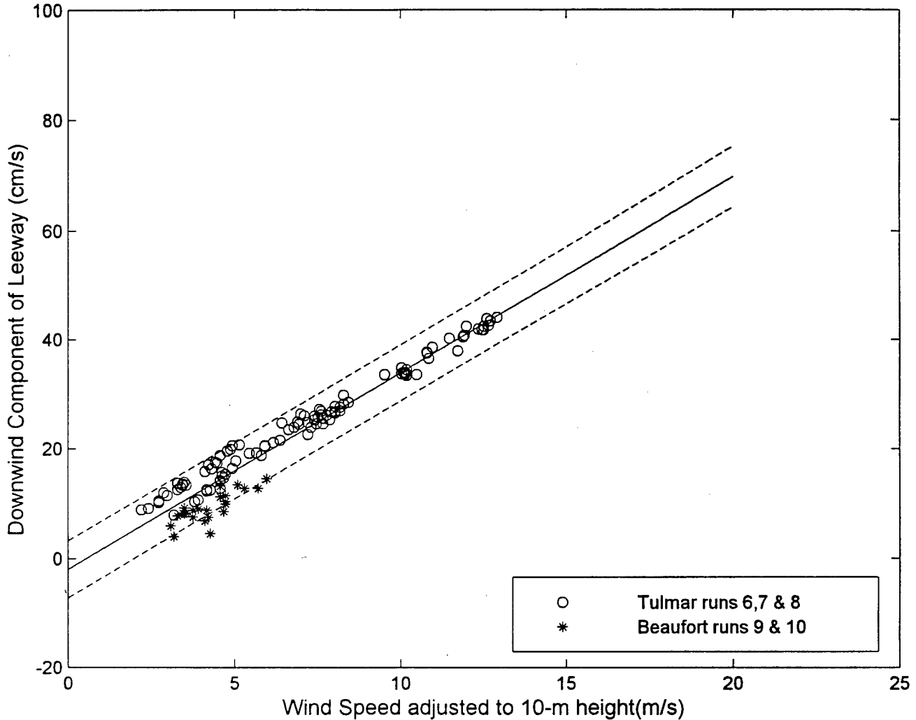
Figure 7-10. The Unconstrained Linear Regression and 95% Prediction Limits of the Downwind Component of Leeway versus Wind Speed at 10 m, Maritime Life Rafts, deep ballast systems, canopy, without drogue, 4-6 person capacity, heavy loading.
