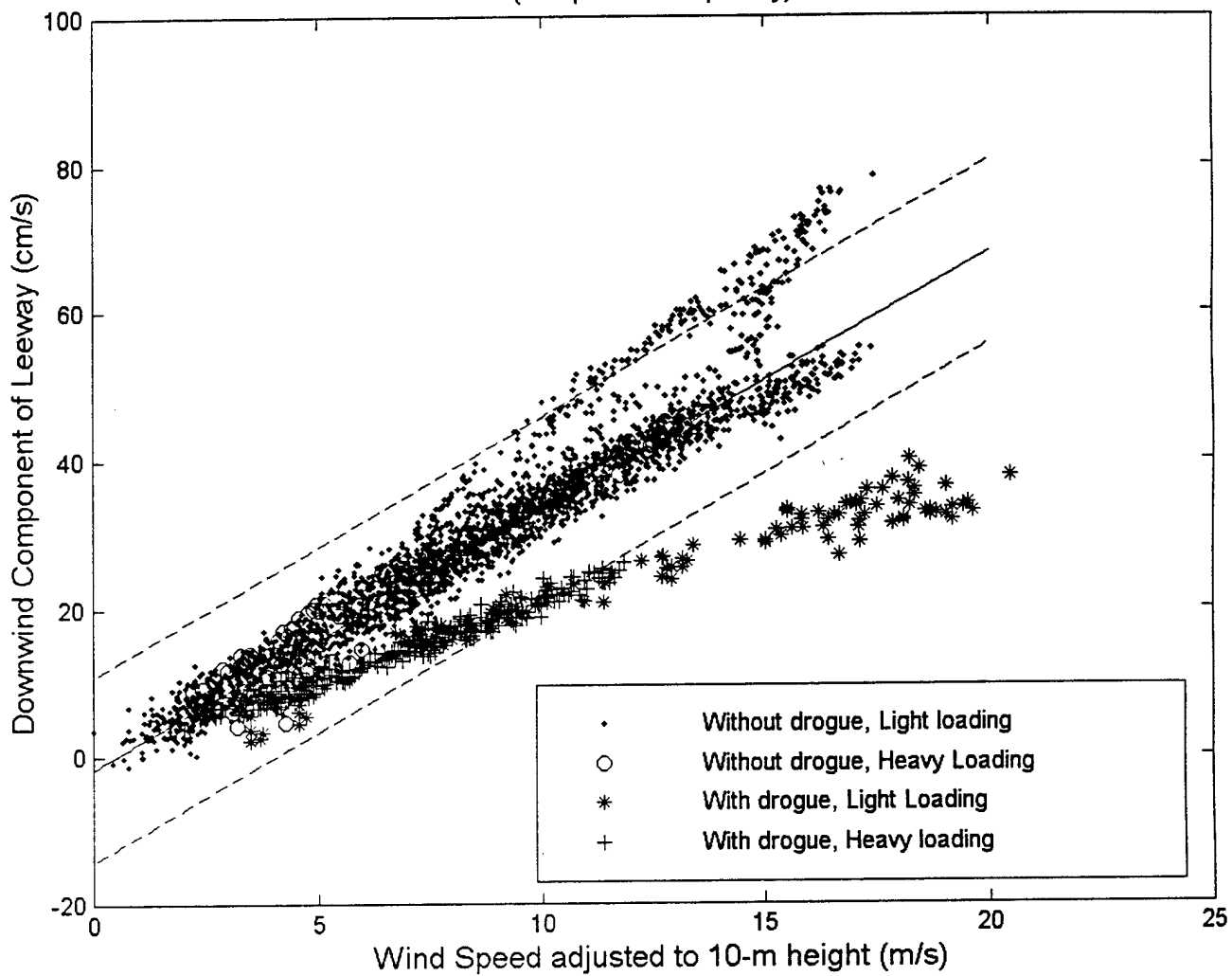
Figure 7-21. The Unconstrained Linear Regressions and 95% Prediction Limits of the Downwind Component of Leeway versus Wind Speed at 10 m, Maritime Life Rafts, deep ballast systems, canopy, 4-6 person capacity.
