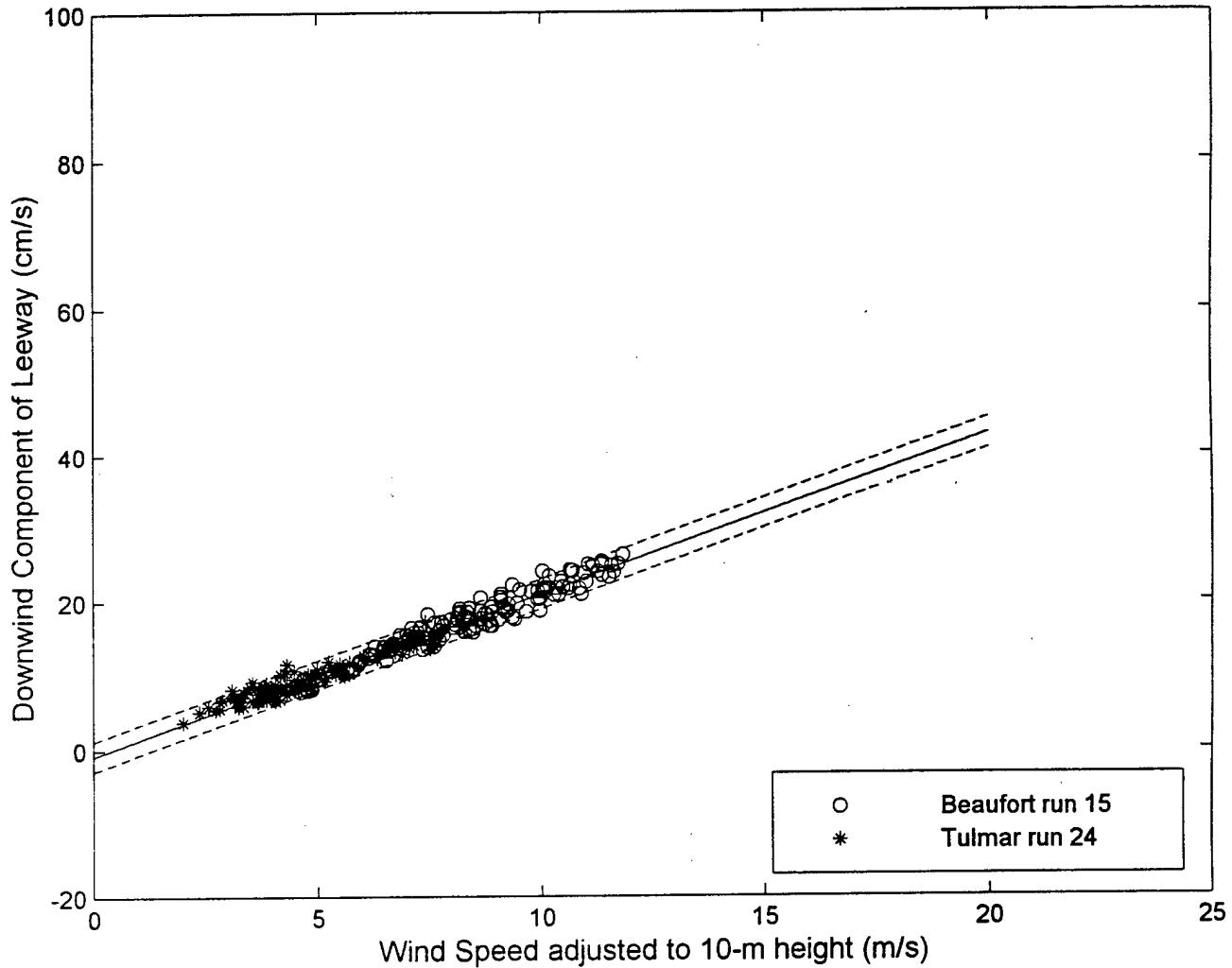
Figure 7-14. The Unconstrained Linear Regression and 95% Prediction Limits of the Downwind Component of Leeway versus Wind Speed at 10m, Maritime Life Rafts, deep ballast systems, canopy, with drogue, 4-6 person capacity, heavy loading.
