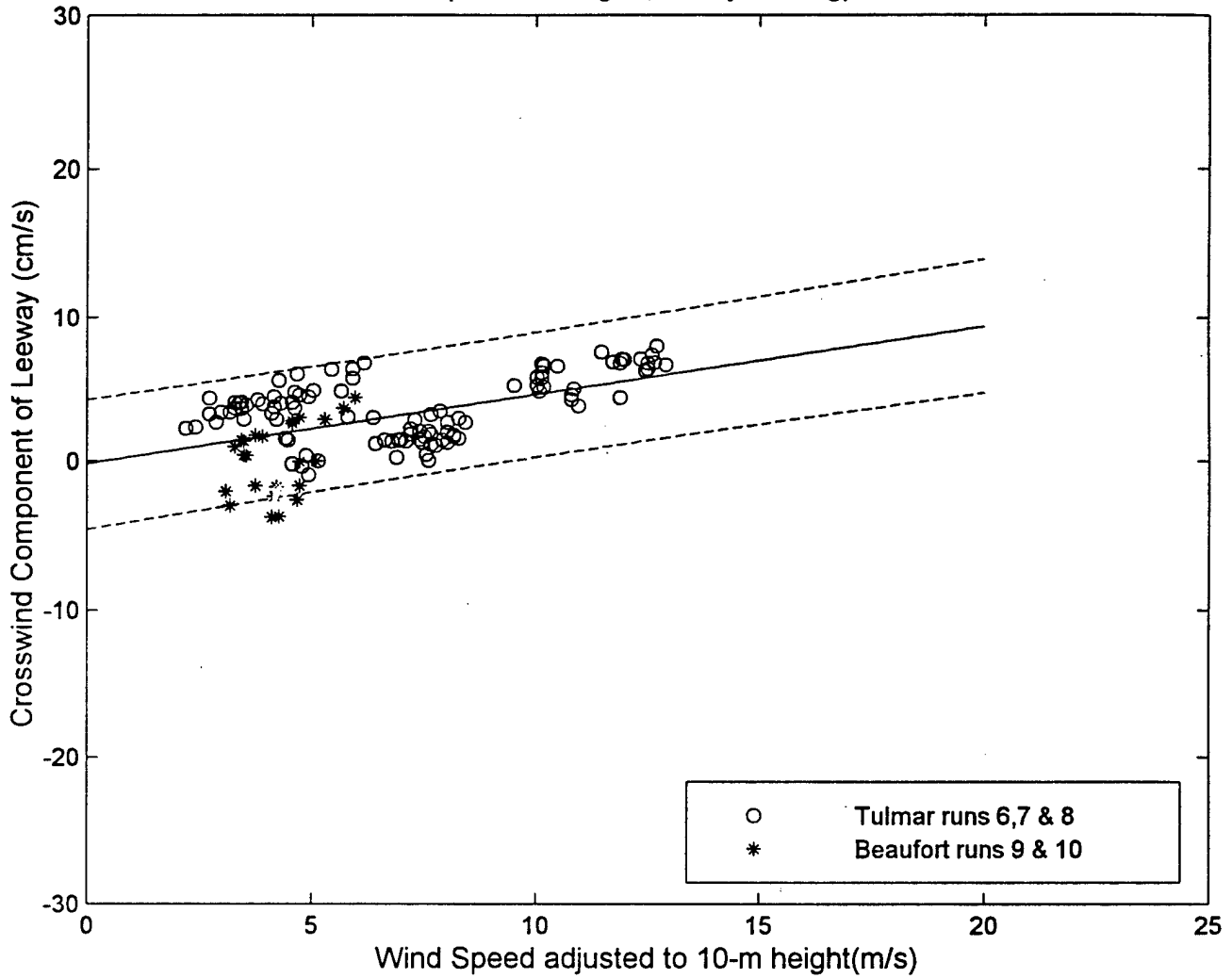
Figure 7-12. The Unconstrained Linear Regression and 95% Prediction Limits of the Crosswind Components of Leeway versus Wind Speed at 10 m, Maritime Life Rafts, deep ballast systems, canopy, without drogue, 4-6 person capacity, heavy loading.
