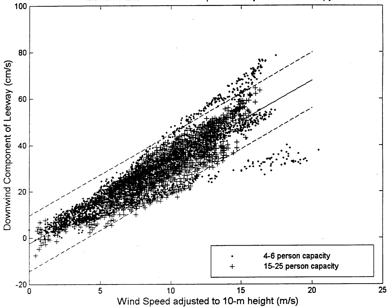
Figure 7-27. The Unconstrained Linear Regression and 95% Prediction Limits of the Downwind Component of Leeway versus Wind Speed at 10 m, Maritime Life Rafts, deep ballast systems and canopy.
