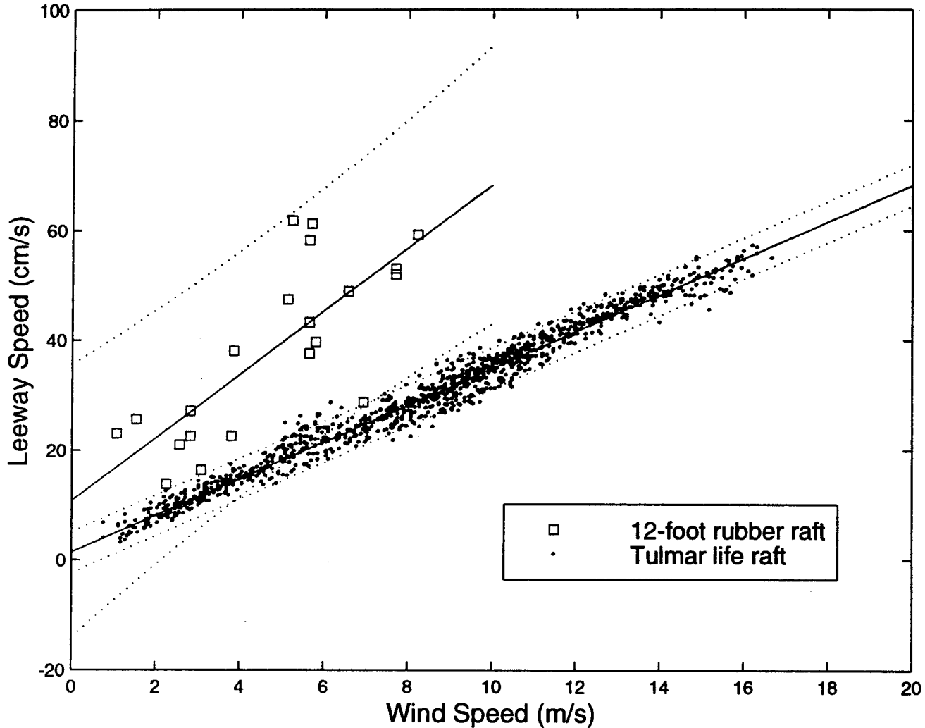
Hufford and Brodia (1974) 12 ft Rubber Raft with sea anchor This report, Tulmar 4-person life raft, 1-person loading, no drogue
