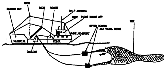
Side Trawler
