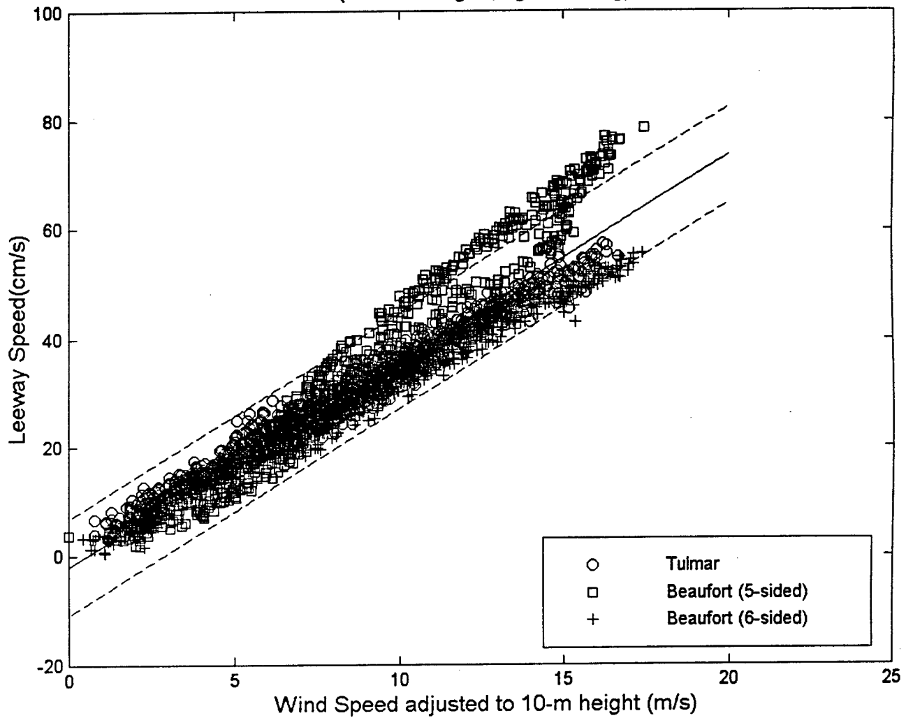
Figure 7-1. The Unconstrained Linear Regression and 95% Prediction Limits of the Leeway Speed versus Wind Speed at 10 m, Maritime Life Rafts, deep ballast systems, canopy, without drogue, 4-6 person capacity, light loading.
