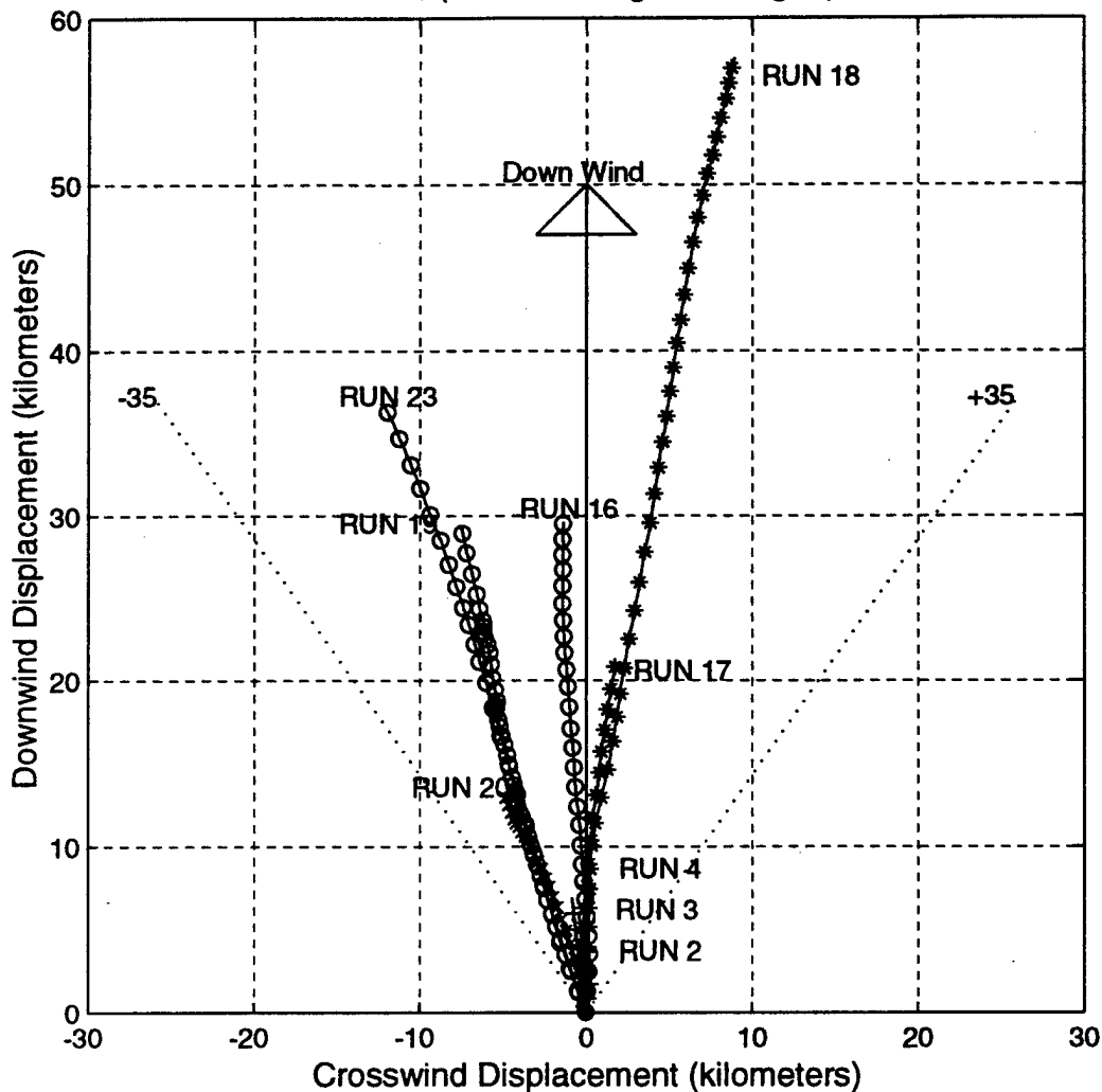
Tulmar 4-Person Life Raft, (1man loading, No Drogue) RUNS 2-4,16-20,23
