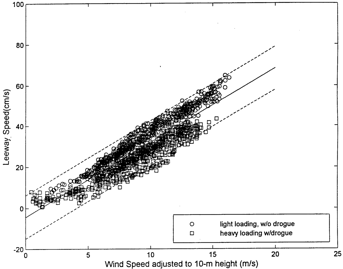
Figure 7-22. The Unconstrained Linear Regression and 95% Prediction Limits of the Leeway Speed versus Wind Speed at 10 m, Maritime Life Rafts, deep ballast systems, canopy, 15-25 person capacity.
