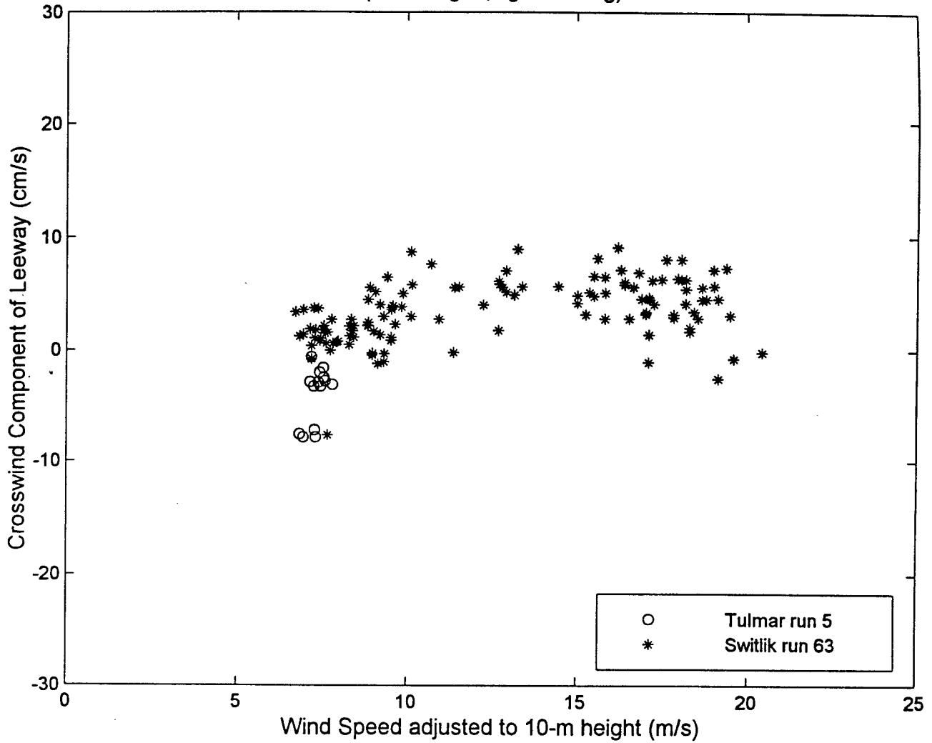
Figure 7-7. The Crosswind Component of Leeway versus Wind Speed at 10 m, Maritime Life Rafts, deep ballast systems, canopy, with drogue, 4-6 person capacity, light loading.
