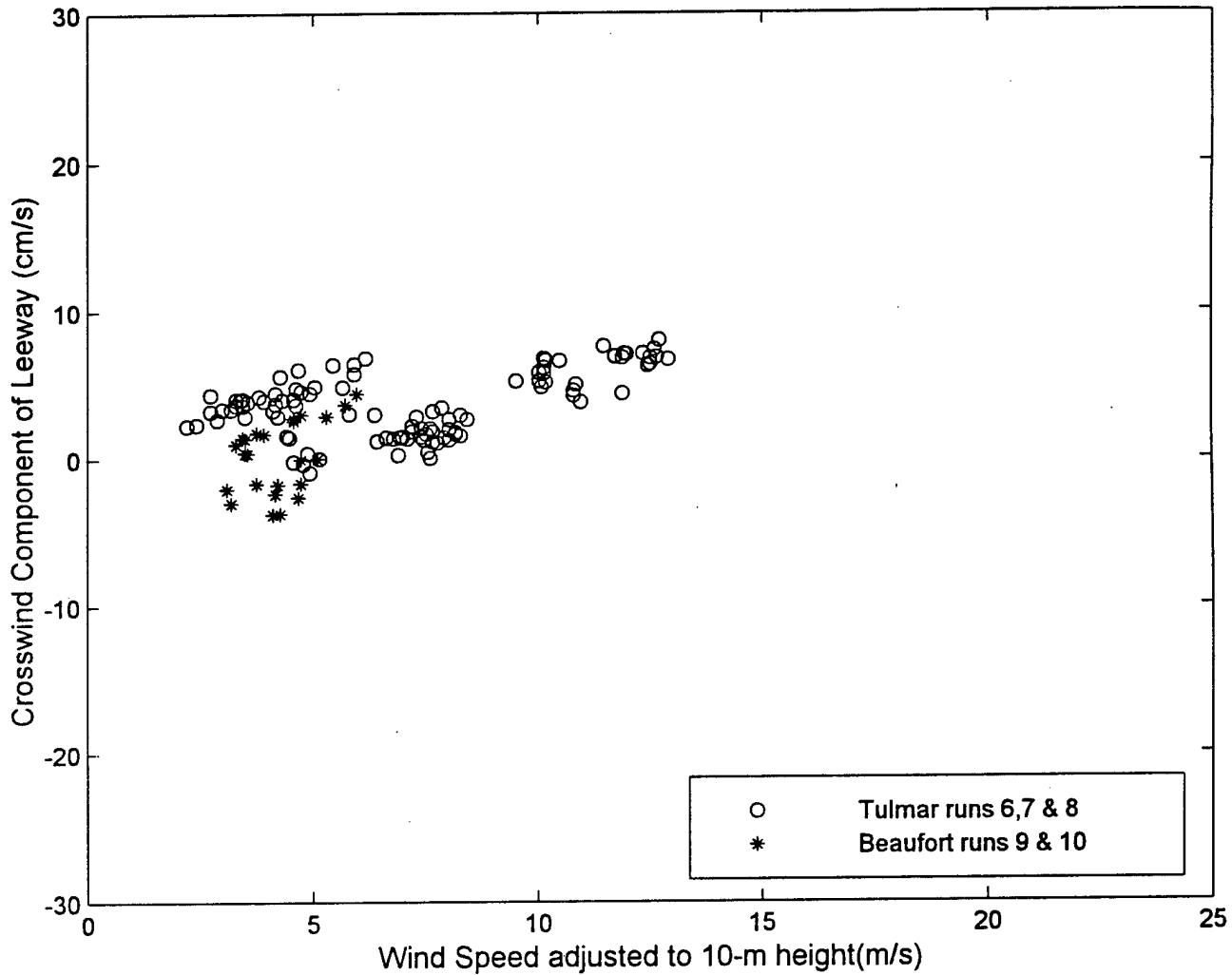
Figure 7-11. The Crosswind Component of Leeway versus Wind Speed at 10 m, Maritime Life Rafts, deep ballast systems, canopy, without drogue, 4-6 person capacity, heavy loading.
