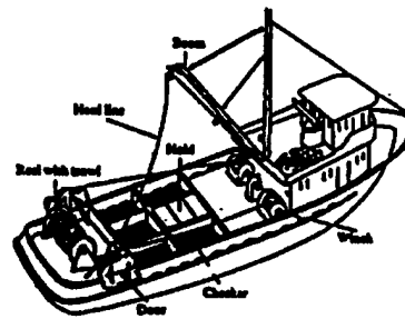
Stern Trawler
