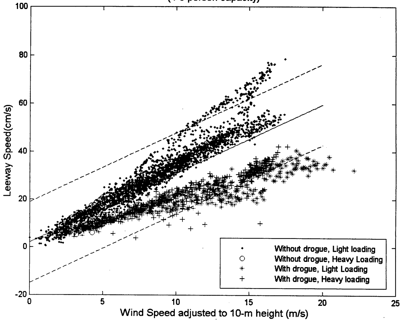
Figure 7-20. The Unconstrained Linear Regression and 95% Prediction Limits of the Leeway Speed versus Wind Speed at 10 m, Maritime Life Rafts, deep ballast systems, canopy, 4-6 person capacity.
