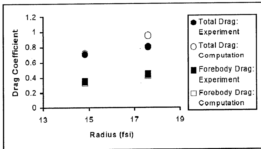
Figure 15. Drag Coefficients for Configuration A.
