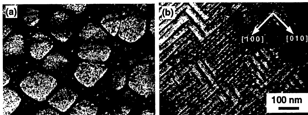
Fig. 1 Dark field images of the (a)Ir-15at% Nb and (b)Ir-15at% Zr alloys which were taken with superlattice reflections ( g=110 ) from the L1_2 structure in the beam direction of [001] . Lattice misfit of Ir-15at% Nb and Ir-15at% Zr alloys are 0.3 and 2.0%, respectively.
