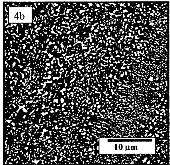
Figure 4: Back-scattered SEM image of a) Mo-20B-10Si (at. %) sput-quenched alloy b) Mo-20B-10Si (at. %) alloy sput-quenched and annealed at 1200°C for 150 hours showing the two-phase microstructure consisting of Mo (bright) phase dispersed in the T2 (dark) matrix.
