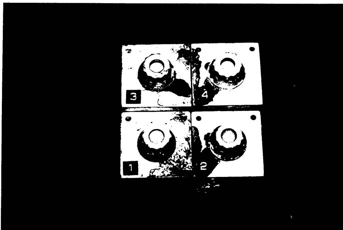
Figure 36. Inconel 718 Nickel-Based Superalloy Bolt Heads With IVD Al Coating After 30 Days of Salt Spray. Reduced 25%.
