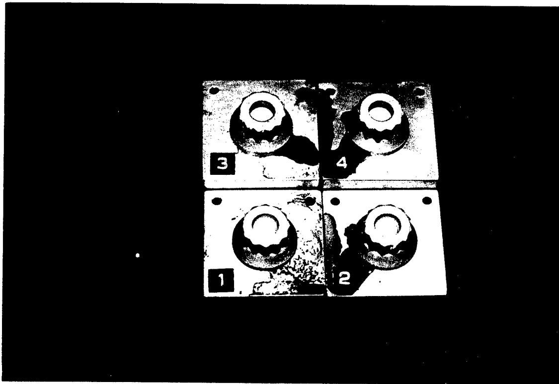
Figure 2. Inconel 718 Nickel-Based Superalloy Bolt Heads With IVD Al Coating Before Salt Spray Exposure. Reduced 25%.
