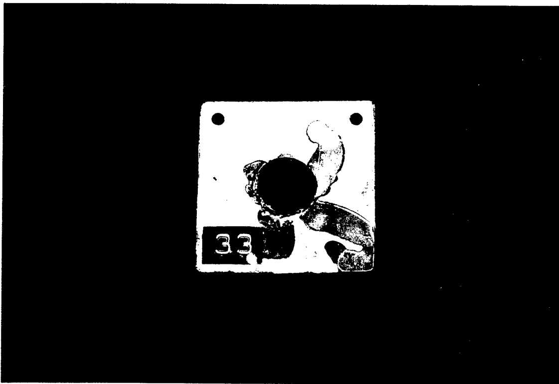
Figure 86. Aluminum Control Block After 62 Days of Salt Spray. Reduced 25%.
