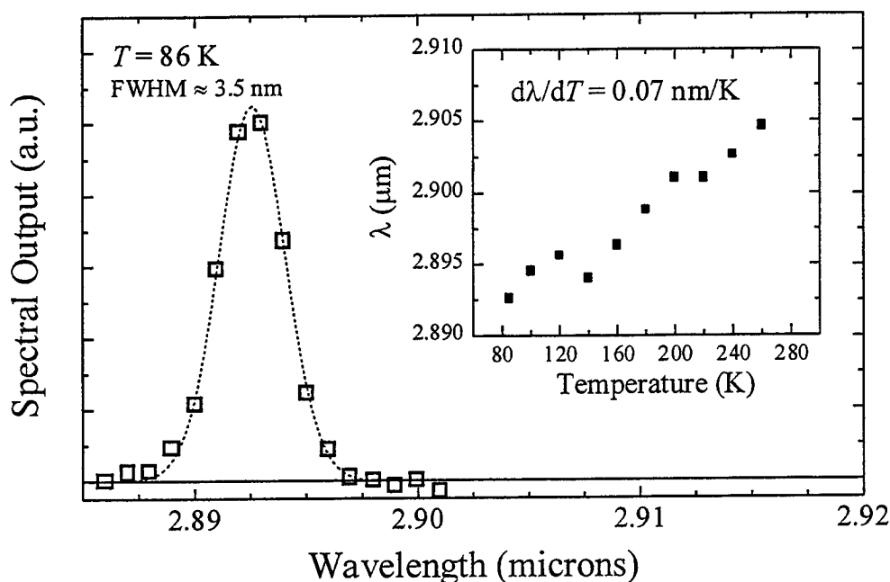
Figure 1. Spectral output (pulsed) vs. wavelength at T = 86 \text{ K} for a 600\text{-}\mu\text{m} -diameter spot (multi-mode), and peak wavelength vs. temperature (inset). The 3.5 \text{ nm} width at 86 \text{ K} , which is typical of the spectra for all temperatures and spot sizes, is much narrower than typical multi-mode edge-emitter widths in the 15\text{-}30 \text{ nm} range.
