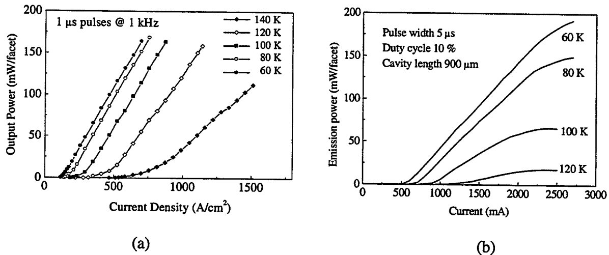
FIGURE 2 (a) L-I curves of a 430 \times 200 \mu\text{m}^2 ridge waveguide IC laser at various heat sink temperatures with 1 \mu s pulses at 0.1% duty cycle and (b) of a 900 \times 200 \mu\text{m}^2 device with 5 \mu s pulses at 10% duty cycle.
