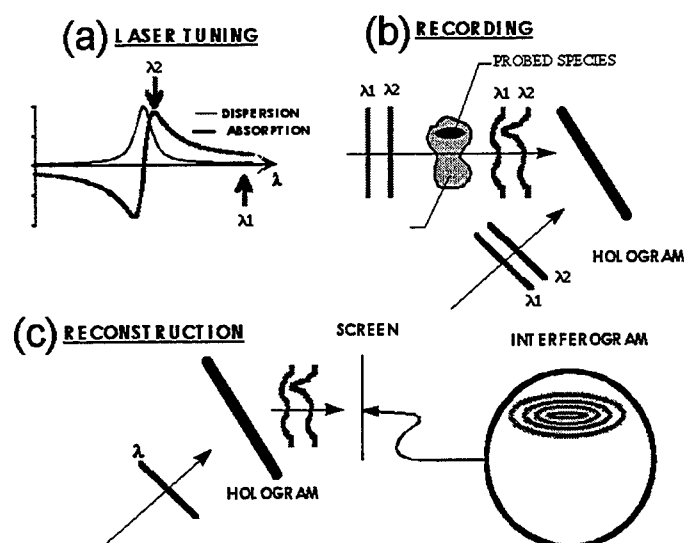
Figure 2: RHI phenomenology
