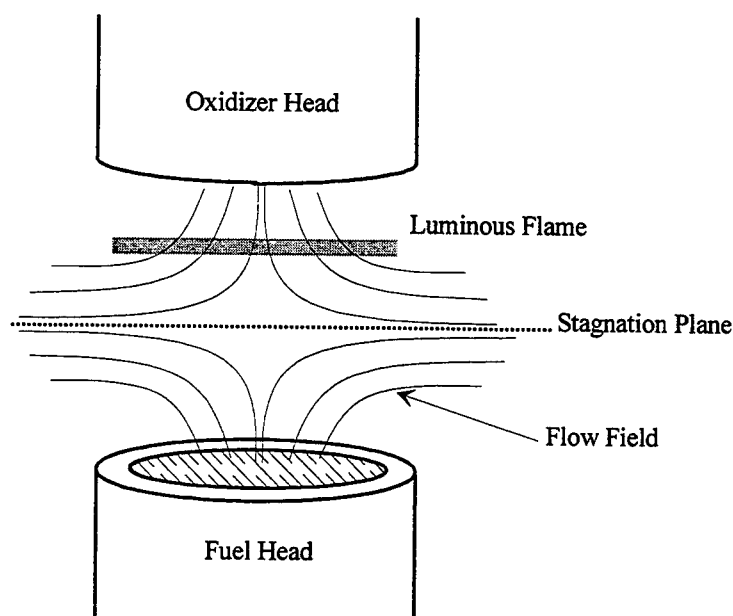
Figure 1. Schematic of a counterflow diffusion burner with the locations of the flame front and stagnation plane indicated. The laser focus will be fixed and the burner heads moved vertically to map the spatial distribution of the species O, H, and OH.
