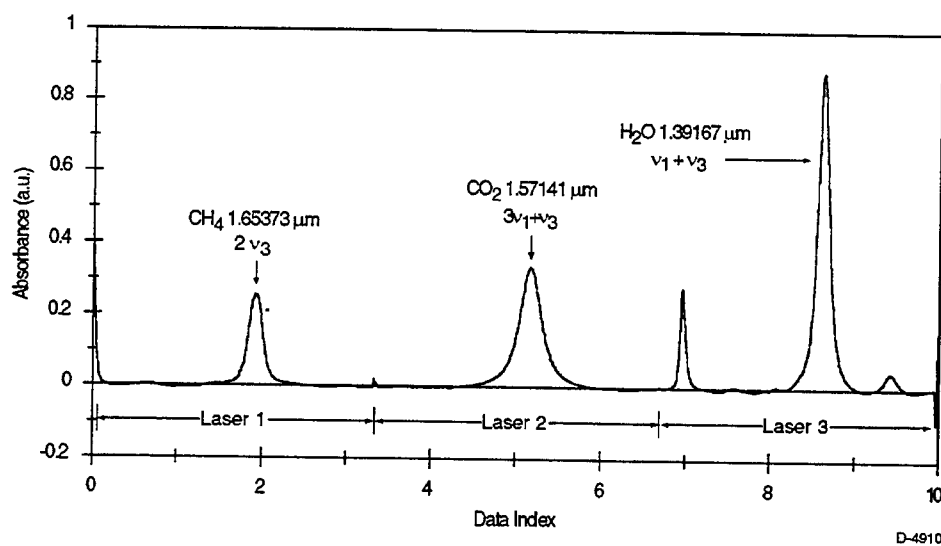
Figure 3. Simultaneous detection of H 2 O, CO 2 , and CH 4 using three separate, multiplexed diode lasers operating at 1.39, 1.57, and 1.65 \mu m.
