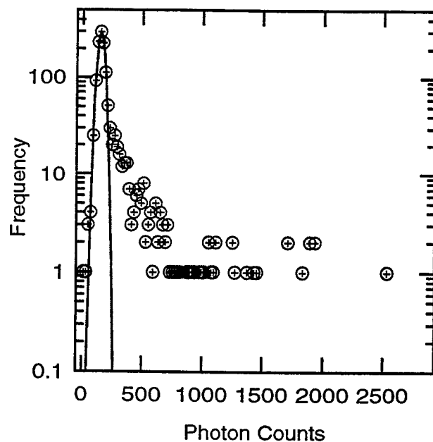
Figure 2: Histogram of photocounts for 1.6 fM Rb solution. The solid line is a Gaussian fit approximating the blank background distribution.
