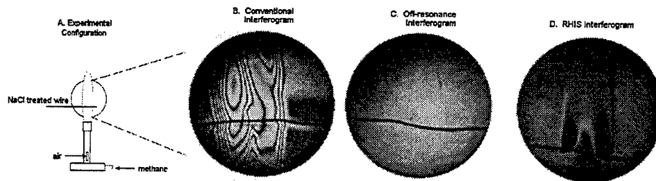
Figure 3: Sodium resonance
