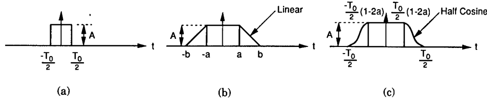
Fig. 4.48 Assumed cloud radiance trace waveform. 10
