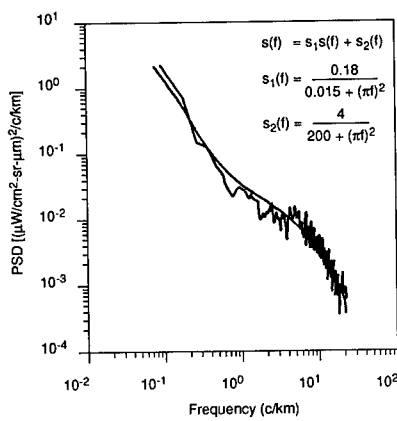
Fig. 4.56 Comparison of model with Fig. 4.55. 10
