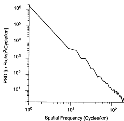
Fig. 4.95 PSD of broken clouds over desert terrain in the 7.88- to 8.80- \mu\text{m} band (HC302R).
