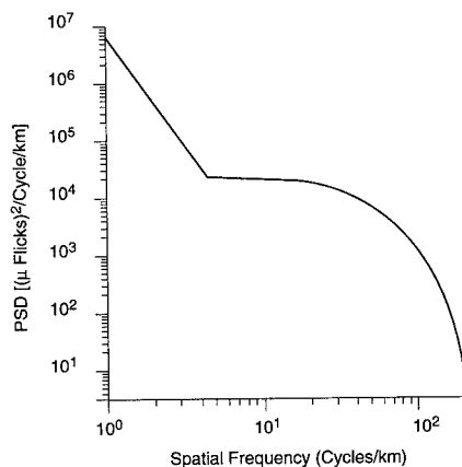
Fig. 4.75 PSD of desert terrain in the 6.68- to 7.28-μm band (HC742R).
