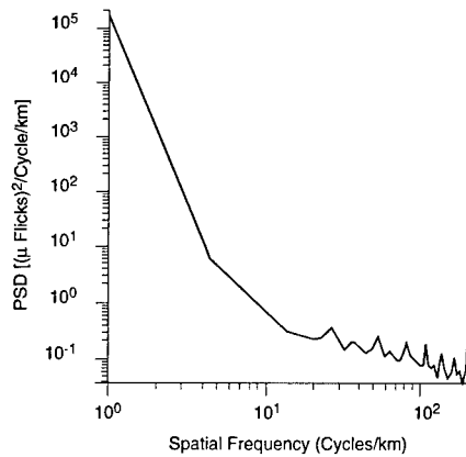
Fig. 4.79 PSD of open ocean in the 4.46- to 5.20-μm band (HC332R).
