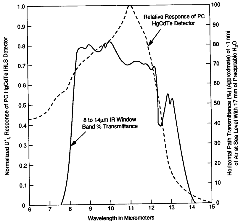
Fig. 1.26 HgCdTe detector response compared to typical 8- to 14- \mu m window transmission at sea level.
