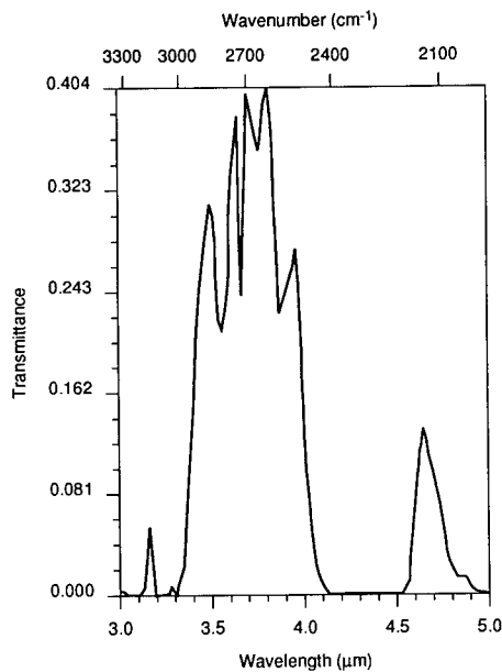
Fig. 4.101 Total horizontal path spectral transmittance in the 3- to 5- \mu m band at 100-km range, 3-km altitude. 1976 Standard Atmosphere is calculated from LOWTRAN 7. Input conditions are shown in Table 4.4. Average band transmittance = 0.0981.
