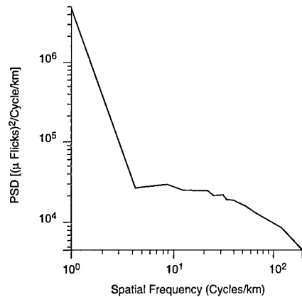
Fig. 4.66 PSD of farm and field terrain at night in the 11.64- to 12.12-μm band (HC426R).
