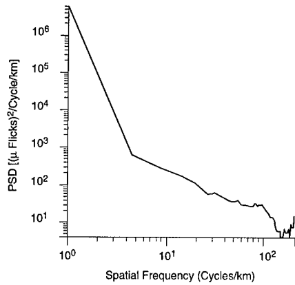
Fig. 4.78 PSD of open ocean in the 8.28- to 8.76-μm band (HC333R).
