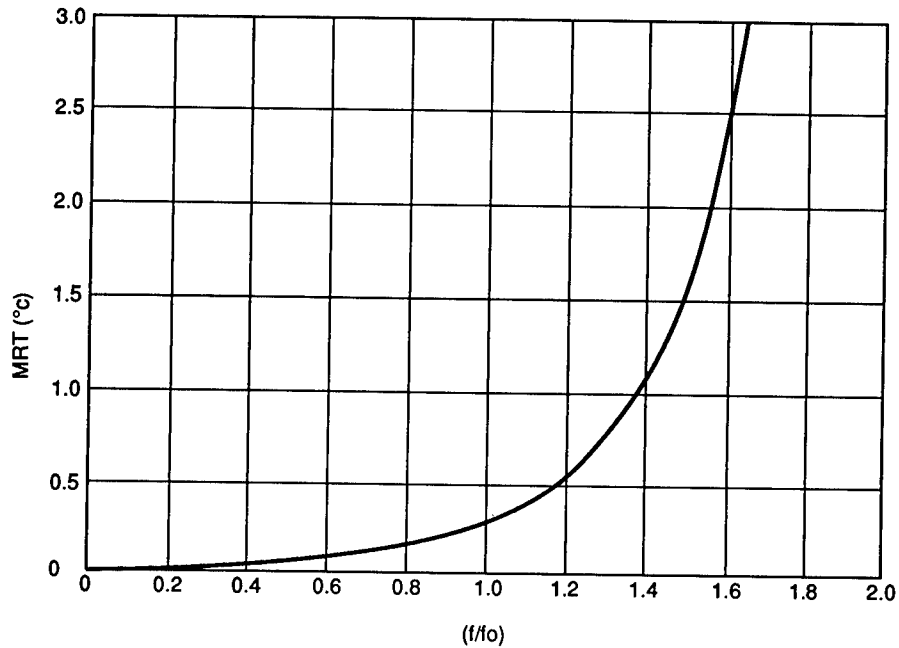
Fig. 2.14 A typical MRT curve for a system with a relative aperture A_R = 0.7 and \text{NET}^* = 0.14^\circ\text{C} . MRT tends to infinity as (f/f_0) approaches 2.0.
