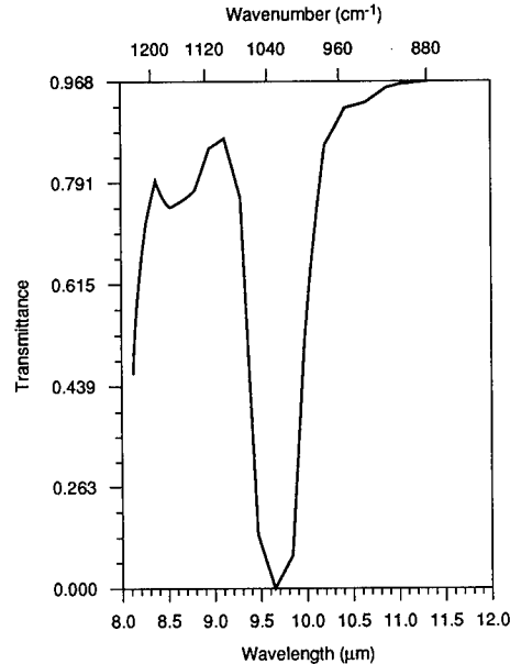
Fig. 4.110 Total horizontal path spectral transmittance in the 8- to 12-μm band at 200-km range, 10-km altitude. 1976 Standard Atmosphere is calculated from LOWTRAN 7. Input conditions are shown in Table 4.4. Average band transmittance = 0.7184.
