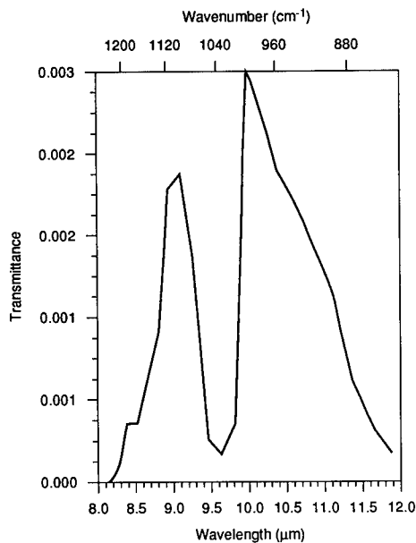
Fig. 4.111 Total horizontal path spectral transmittance in the 8- to 12-μm band at 300-km range, 3-km altitude. 1976 Standard Atmosphere is calculated from LOWTRAN 7. Input conditions are shown in Table 4.4. Average band transmittance = 0.0010.
