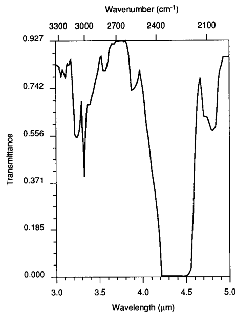
Fig. 4.102 Total horizontal path spectral transmittance in the 3- to 5- \mu m band at 100-km range, 10-km altitude. 1976 Standard Atmosphere is calculated from LOWTRAN 7. Input conditions are shown in Table 4.4. Average band transmittance = 0.6211.
