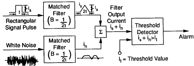
Fig. 4.158 Description of threshold detection process.
