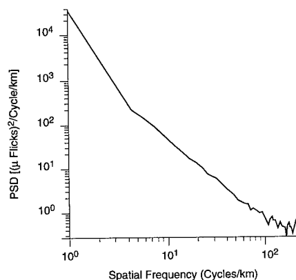
Fig. 4.76 PSD of clear night sky in the 3.74- to 4.08-μm band (HC770R).
