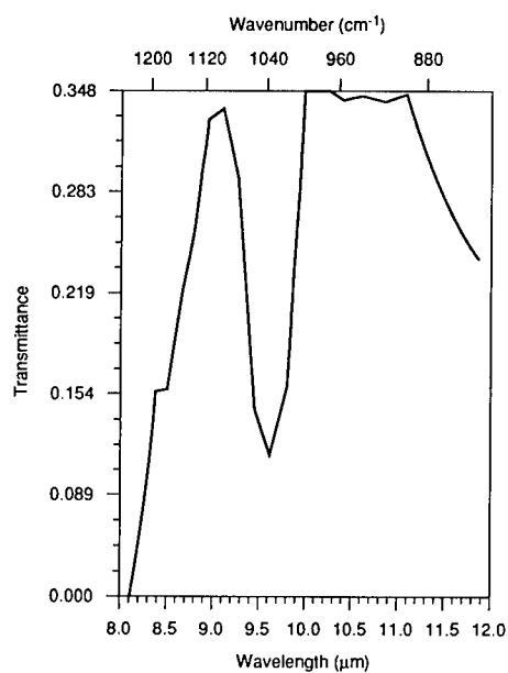
Fig. 4.107 Total horizontal path spectral transmittance in the 8- to 12- \mu m band at 100-km range, 3-km altitude. 1976 Standard Atmosphere is calculated from LOWTRAN 7. Input conditions are shown in Table 4.4. Average band transmittance = 0.232.
