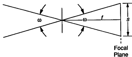
Fig. 1.15 Simplified use of f/\# in line scanners.
