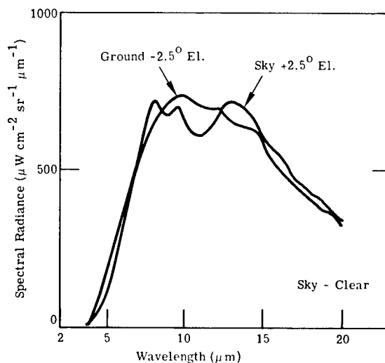
Fig. 4.32 Comparative spectra of the ground and sky near the horizon (Peterson Field, Colorado). 11
