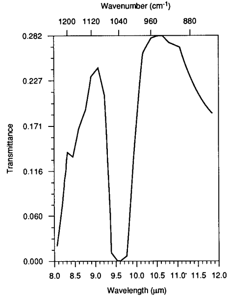
Fig. 4.138 Total uplooking path spectral transmittance to space in the 8- to 12- \mu\text{m} band at a solar zenith angle of 85 deg. 1976 Standard Atmosphere is calculated from LOW-TRAN 7. Input conditions are shown in Table 4.5. Average band transmittance = 0.163.
