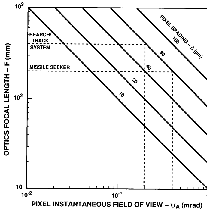
Fig. 3.13 Pixel-spacing requirements.
