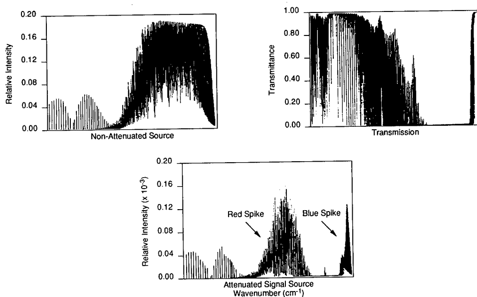
Fig. 4.10 Synthetic spectrum of engine plume at a resolution of 0.01 \text{ cm}^{-1} showing the formation of the blue and red spike. 10
