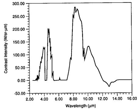
Fig. 4.20 Calculated contrast signature of a 500-m 2 target at an altitude of 1 km observed from space, midlatitude summer conditions, T = 294 K. 10
