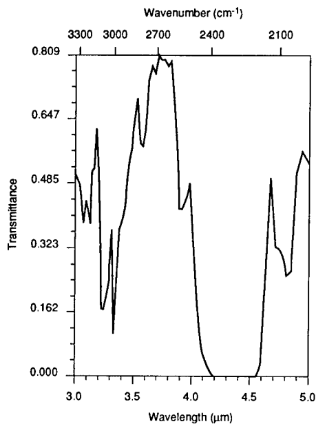
Fig. 4.106 Total horizontal path spectral transmittance in the 3- to 5- \mu m band at 300-km range, 10-km altitude. 1976 Standard Atmosphere is calculated from LOWTRAN 7. Input conditions are shown in Table 4.4. Average band transmittance = 0.3659.
