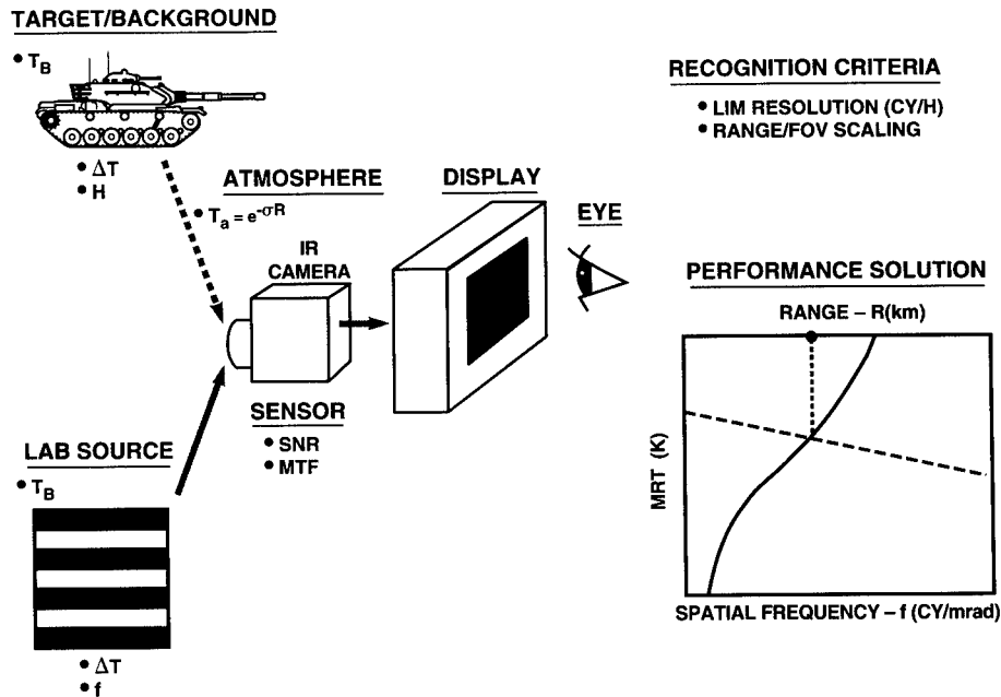
Fig. 3.15 Recognition-range prediction.
