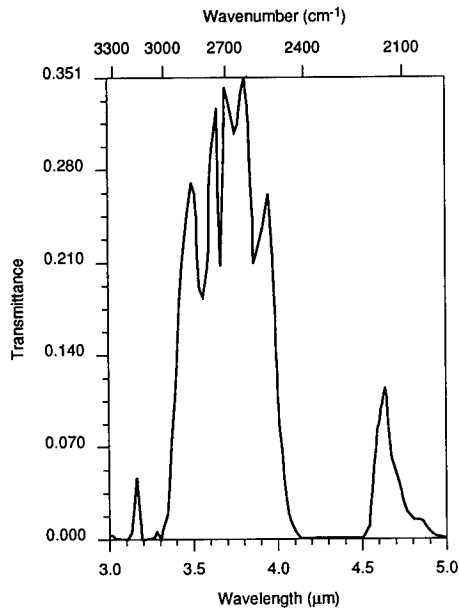
Fig. 4.137 Total uplooking path spectral transmittance to space in the 3- to 5- \mu\text{m} band at a solar zenith angle of 85 deg. 1976 Standard Atmosphere is calculated from LOW-TRAN 7. Input conditions are shown in Table 4.5. Average band transmittance = 0.0866.
