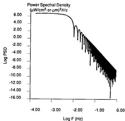
Fig. 4.52 The PSD of 1-km clouds moving at 10 \text{ m s}^{-1} across a 1-km pixel using a half-cosine waveform. 10
