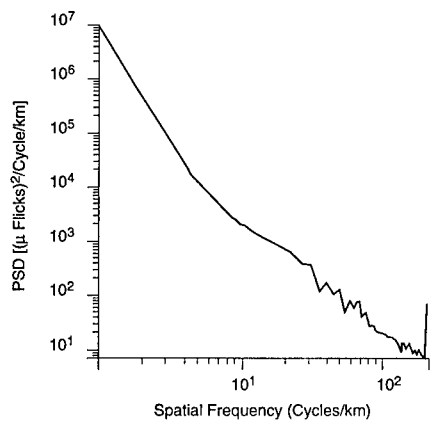
Fig. 4.82 PSD of ocean coastline in the 8.28- to 8.76-μm band (HC506R).
