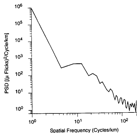
Fig. 4.72 PSD of mountain hills and fields in the 4.46- to 5.20-μm band (HC633R).
