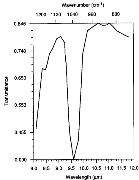
Fig. 4.140 Total uplooking path spectral transmittance to space in the 8- to 12- \mu\text{m} band at a solar zenith angle of 30 deg. 1976 Standard Atmosphere is calculated from LOW-TRAN 7. Input conditions are shown in Table 4.5. Average band transmittance = 0.6966.
