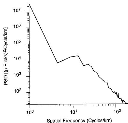
Fig. 4.73 PSD of mountain hills and fields in the 8.28- to 8.76-μm band (HC635R).
