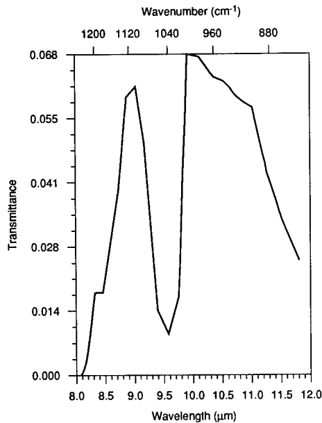
Fig. 4.109 Total horizontal path spectral transmittance in the 8- to 12-μm band at 200-km range, 3-km altitude. 1976 Standard Atmosphere is calculated from LOWTRAN 7. Input conditions are shown in Table 4.4. Average band transmittance = 0.0352.
