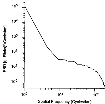
Fig. 4.83 PSD of ocean coastline in the 4.46- to 5.20-μm band (HC505R).
