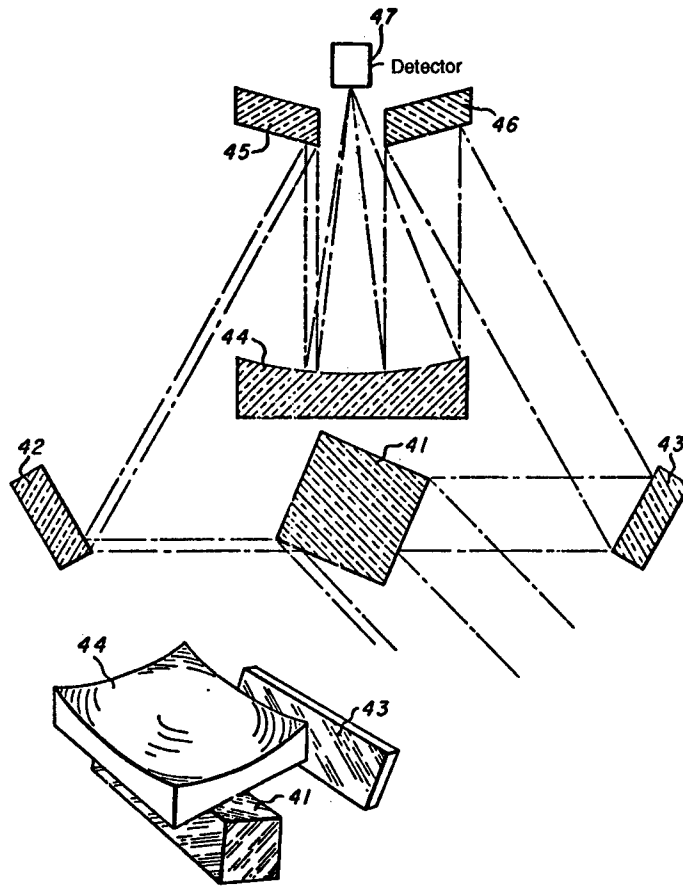
Fig. 1.9 Single-parabola Kennedy scanner. 1
