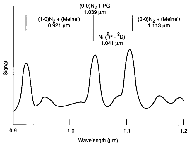
Fig. 4.40 Auroral spectrum, 0.9 to 1.2 \mu\text{m} , obtained with a lead sulfide spectrometer; projected slit width 100 Å. 11
