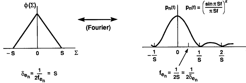
Fig. 3.4 Fourier transform pairs—rectangular aperture functions.
