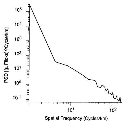
Fig. 4.67 PSD of farm and field terrain at night in the 4.46- to 5.20-μm band (HC425R).
