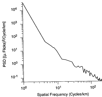
Fig. 4.96 PSD of urban area in the 4.46- to 5.20-μm band (HC652R).
