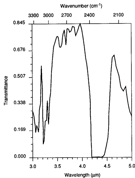
Fig. 4.139 Total uplooking path spectral transmittance to space in the 3- to 5- \mu\text{m} band at a solar zenith angle of 30 deg. 1976 Standard Atmosphere is calculated from LOW-TRAN 7. Input conditions are shown in Table 4.5. Average band transmittance = 0.4242.
