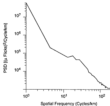
Fig. 4.69 PSD of farmland terrain in the 8.28- to 8.76-μm band (HC442R).
