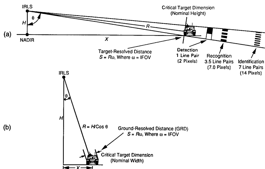
Fig. 1.22 Comparison between oblique and plan viewing: (a) oblique viewing where \theta > 60^\circ ; (b) plan viewing where \theta \leq 60^\circ .
