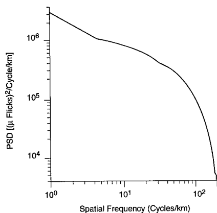
Fig. 4.74 PSD of desert terrain in the 4.56- to 4.78-μm band (HC741R).
