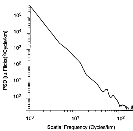
Fig. 4.81 PSD of ocean island coast background in the 4.46- to 5.20-μm band (HC654R).
