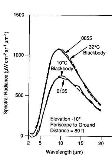
Fig. 4.31 Day and night radiance of grass-covered field (Peterson Field, Colorado). 11
