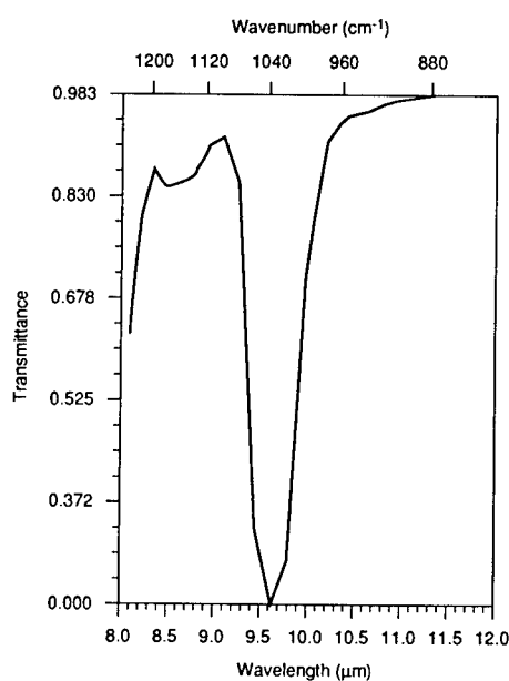
Fig. 4.108 Total horizontal path spectral transmittance in the 8- to 12- \mu m band at 100-km range, 10-km altitude. 1976 Standard Atmosphere is calculated from LOWTRAN 7. Input conditions are shown in Table 4.4. Average band transmittance = 0.798.
