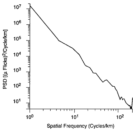
Fig. 4.80 PSD of ocean island coast background in the 8.28- to 8.76-μm band (HC655R).
