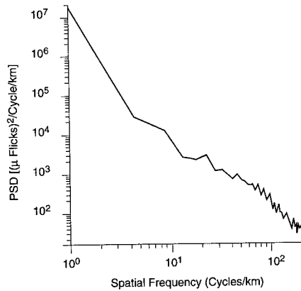
Fig. 4.97 PSD of urban area in the 8.28- to 8.76-μm band (HC653R).
