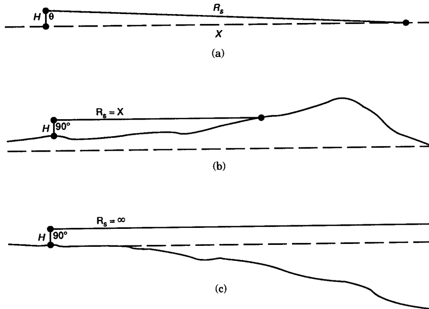
Fig. 1.19 Terrain effects in low-level missions: (a) flat earth; (b) rising terrain limits offset distance (defocus effect must be considered); (c) falling terrain causes view of sky in imagery.
