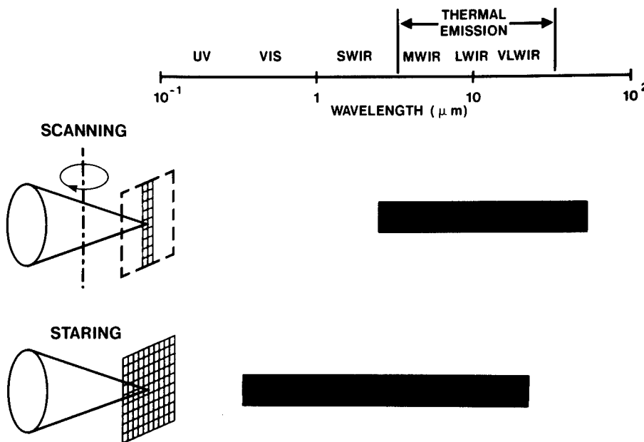
Fig. 3.1 Sensor design alternatives.
