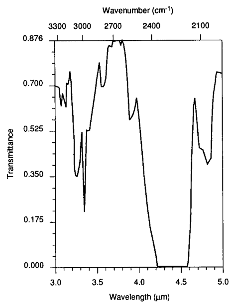
Fig. 4.104 Total horizontal path spectral transmittance in the 3- to 5- \mu m band at 200-km range, 10-km altitude. 1976 Standard Atmosphere is calculated from LOWTRAN 7. Input conditions are shown in Table 4.4. Average band transmittance = 0.4950.
