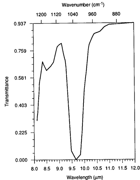
Fig. 4.112 Total horizontal path spectral transmittance in the 8- to 12-μm band at 300-km range, 10-km altitude. 1976 Standard Atmosphere is calculated from LOWTRAN 7. Input conditions are shown in Table 4.4. Average band transmittance = 0.6487.
