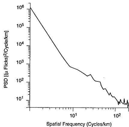
Fig. 4.68 PSD of farmland terrain in the 3.74- to 4.08-μm band (HC441R).
