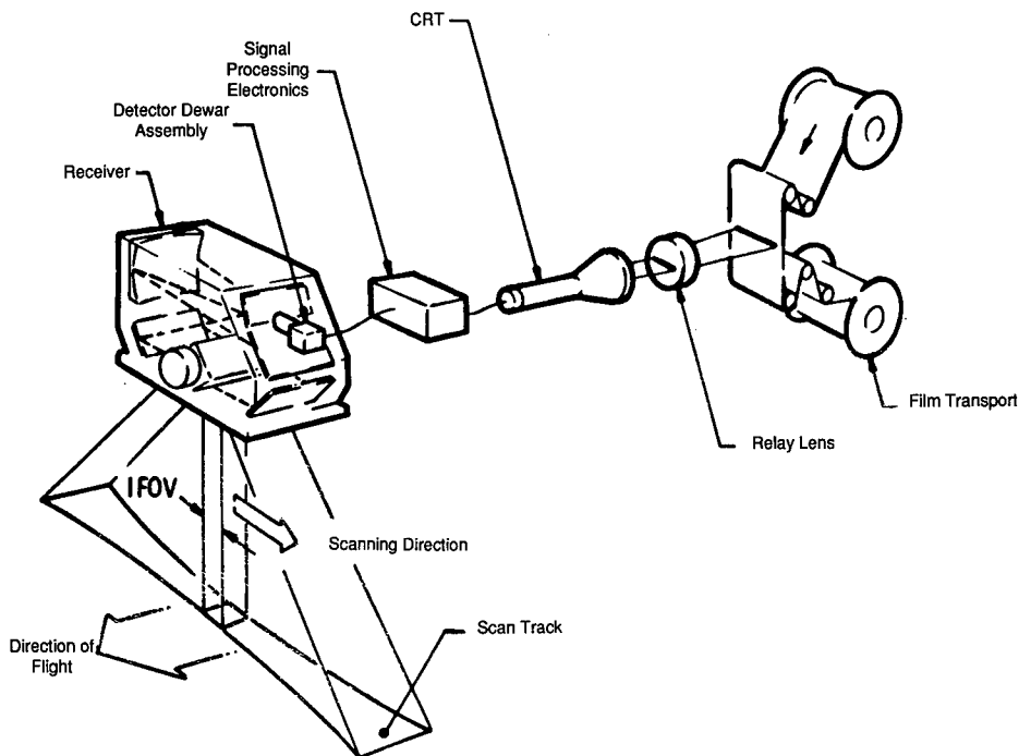
Fig. 1.1 Typical IR reconnaissance set.
