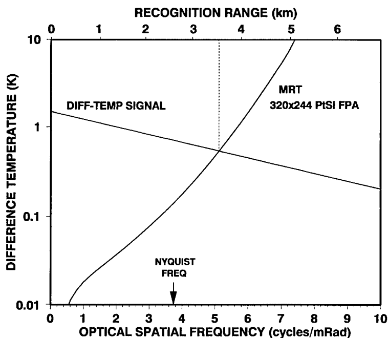
Fig. 3.18 Minimum resolvable temperature.
