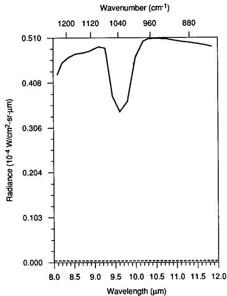
Fig. 4.142 Total downlooking path spectral radiance from space in the 8- to 12- \mu\text{m} band. Solar zenith angle of 0 deg. The dotted line is the contribution from the earth's albedo, \approx 0.4 . Input conditions are shown in Table 4.6. Average band radiance = 2.147 \times 10^{-3} \text{ W cm}^{-2} \text{ sr}^{-1} \mu\text{m}^{-1} .
