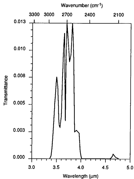
Fig. 4.105 Total horizontal path spectral transmittance in the 3- to 5- \mu m band at 300-km range, 3-km altitude. 1976 Standard Atmosphere is calculated from LOWTRAN 7. Input conditions are shown in Table 4.4. Average band transmittance = 0.0019.
