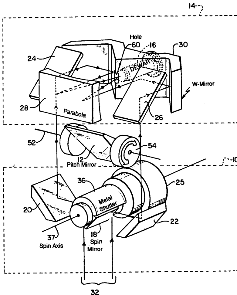
Fig. 1.12 Dual IRLS/FLIR in downward mode. 2
