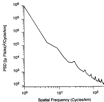
Fig. 4.77 PSD of the clear night sky in the 7.80- to 13.50-μm band (HC771R).
