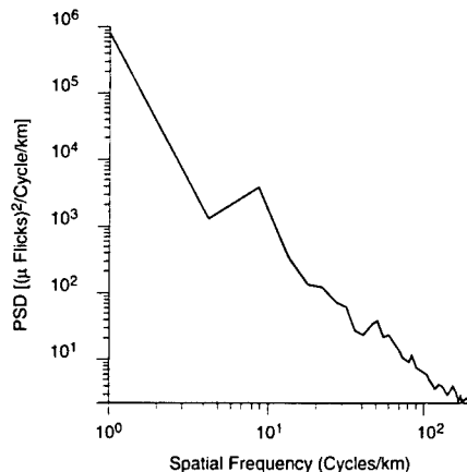
Fig. 4.71 PSD of mountain terrain with some clouds in the 11.64- to 12.12-μm band (HC478R).
