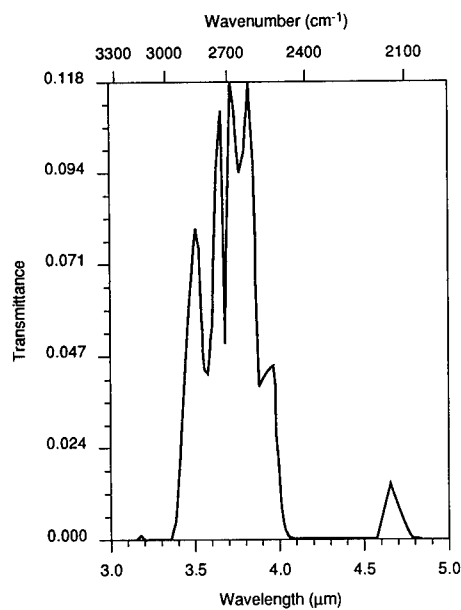
Fig. 4.103 Total horizontal path spectral transmittance in the 3- to 5- \mu m band at 200-km range, 3-km altitude. 1976 Standard Atmosphere is calculated from LOWTRAN 7. Input conditions are shown in Table 4.4. Average band transmittance = 0.0213.
