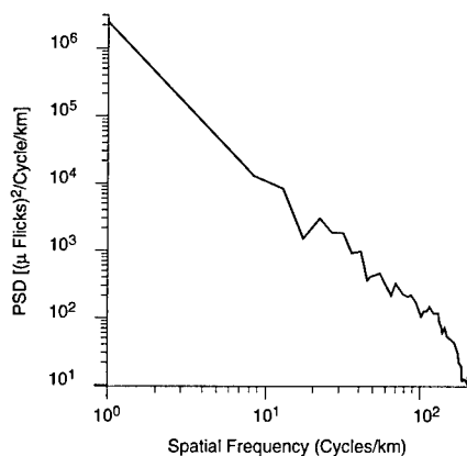
Fig. 4.93 PSD of broken clouds over farm and field background in the 11.64- to 12.12- \mu\text{m} band (HC306R).
