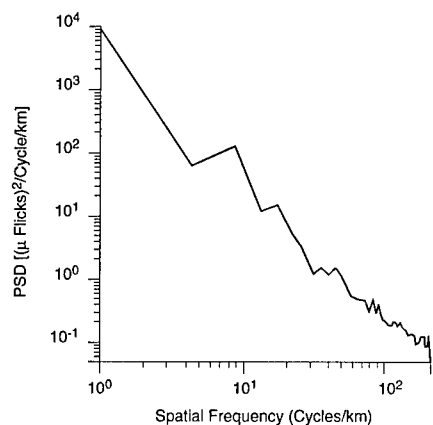
Fig. 4.70 PSD of mountain terrain with some clouds in the 4.46- to 5.20-μm band (HC477R).
