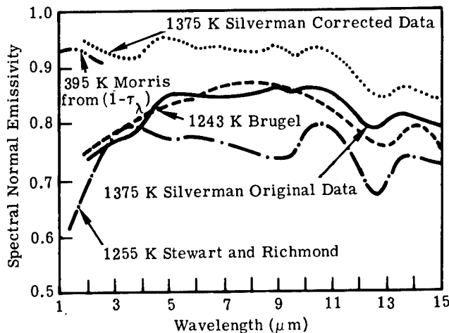
Fig. 2.13 The spectral emissivity of a globar. 14
