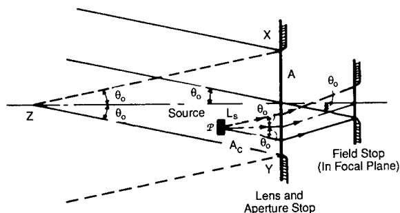
Fig. 4.14 Near-small-source (Jones method) calibration. The source with area A_s and radiance L_s is completely within the region bounded by XZ and YZ , each of which makes an angle, \theta_s , with the optical axis, where \theta_0 is the half-field angle. P is any arbitrary point of the source. Rays from any such point, P , within a cone of half-angle \theta_s , will uniformly irradiate the circular field stop as shown.
