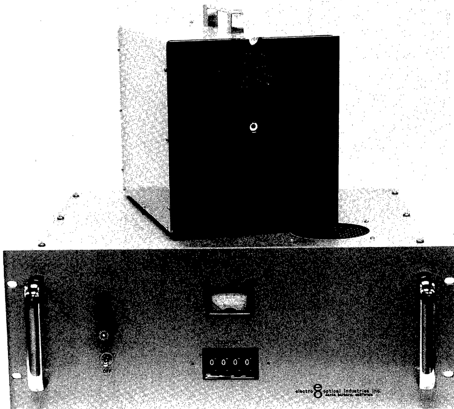
Fig. 2.8 EOI blackbody.
