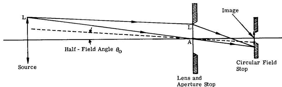
Fig. 4.12 Distant-extended-source configuration. The source image completely fills the circular field stop and R_L \equiv V/L .
