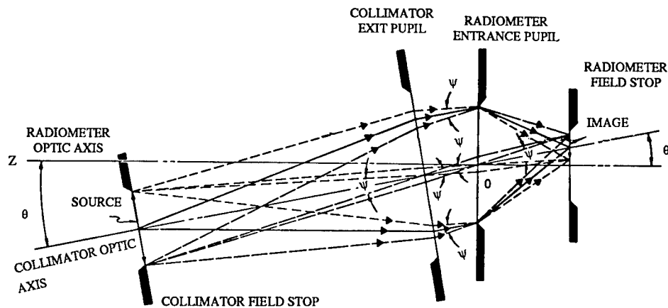
Fig. 4.11 Geometry for mapping the field with a collimator, where 0 is the center of the radiometer entrance pupil, \theta is the angle between the optic axes, which intersect at 0, and \psi is the angle between the extreme rays in the collimated beam and the angle subtended at 0 by the image of the source \psi \ll \theta (the relative dimensions are exaggerated to emphasize the angles).
