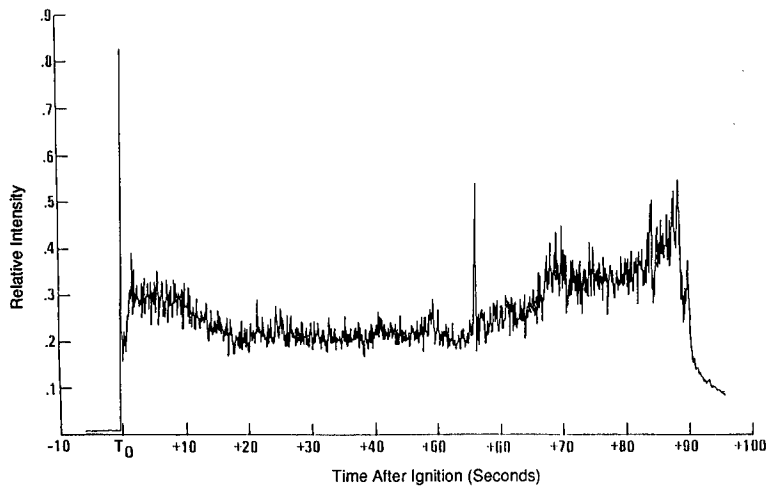
Fig. 2.80 Temporal characteristics of the M49-A1 flare, 3.5- to 5.0- \mu\text{m} band.
