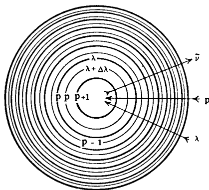
Fig. 4.48 Interference system of two close lines.
