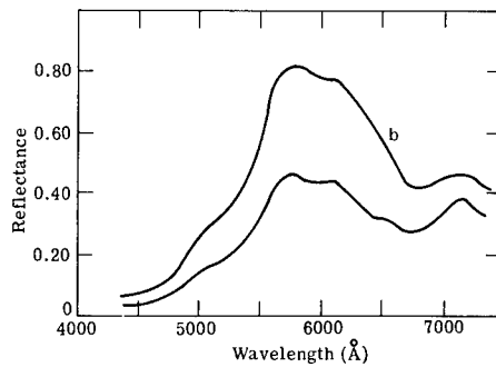
Fig. 3.55. Spectral reflectance, measured at 90,000-ft (27.5-km) altitude above summertime cultivated farmland at 50^\circ solar zenith angle. Curve b shows the effect of the intrusion of 0.6 cumular cloud structure. 93
