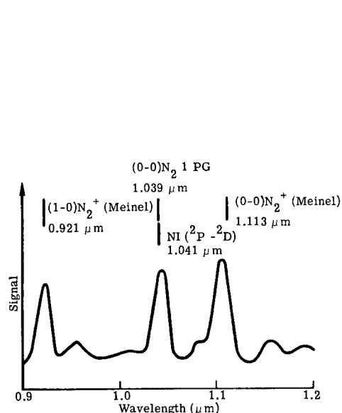
Fig. 3.31 Auroral spectrum between 0.9 to 1.2 \mu\text{m} . It was obtained with a lead sulfide spectrometer; projected slit width 100 \text{\AA} (Ref. 65).
