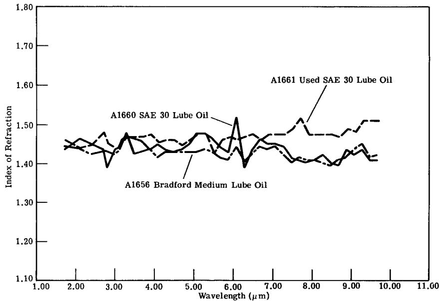
Fig. 3.138 The index of refraction of A1661 used SAE 30 lube oil, A1660 SAE 30 lube oil, and A1656 Bradford medium lube oil. 120
