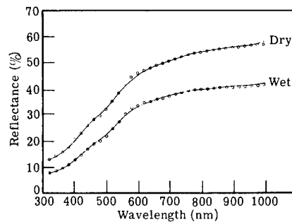
(p) Carbonate sand. Type-two curves. Waikiki Beach, Honolulu, Hawaii.
