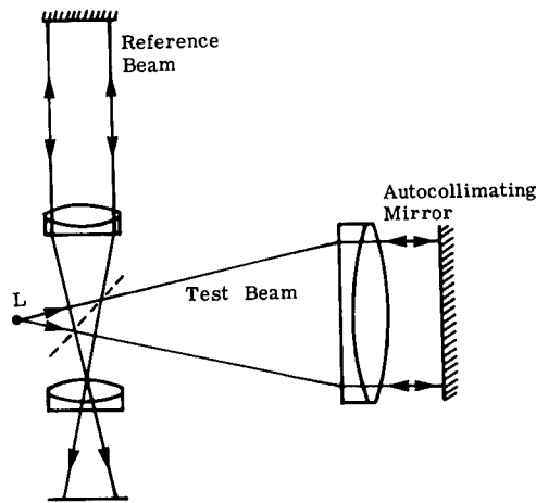
Fig. 4.43 Williams interferometer.
