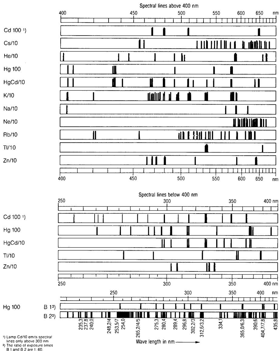
Fig. 2.45 Spectral lamps. 18
