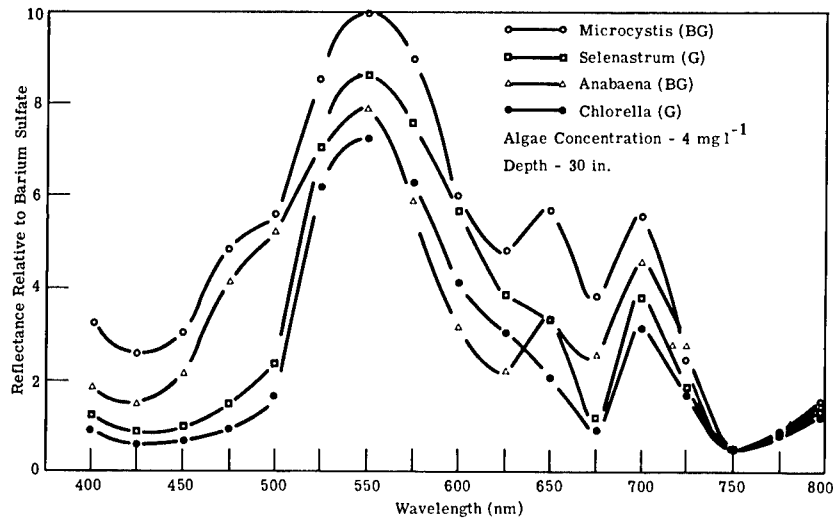
Fig. 3.134 Relative spectral reflectance curves for two green and two blue-green algae at 4 \text{ mg l}^{-1} concentration. 118
