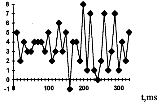
d) random vibration 10 g (\bar{N}=3.290 \text{ pulses}; \sigma_N=0.135 \text{ deg/s})
