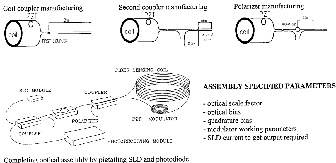
Fig.9.3. The main steps of FOG manufacturing.
