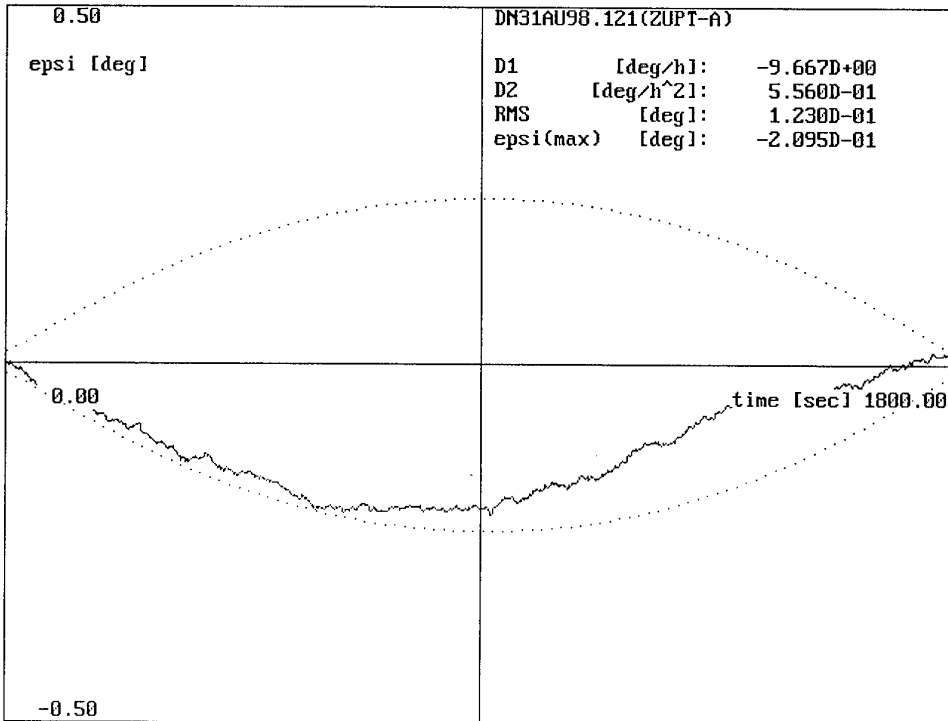
Fig. 6.2a, b Residues for Track Angle Measurement Investigations; a) with 1 Angular Position Update at the Beginning and the End of the Mission b) in Addition 3 × 1 min ZUPTs at 300s, 600s and 900s (FOG Measurements s. Fig. 2.3 bottom)
