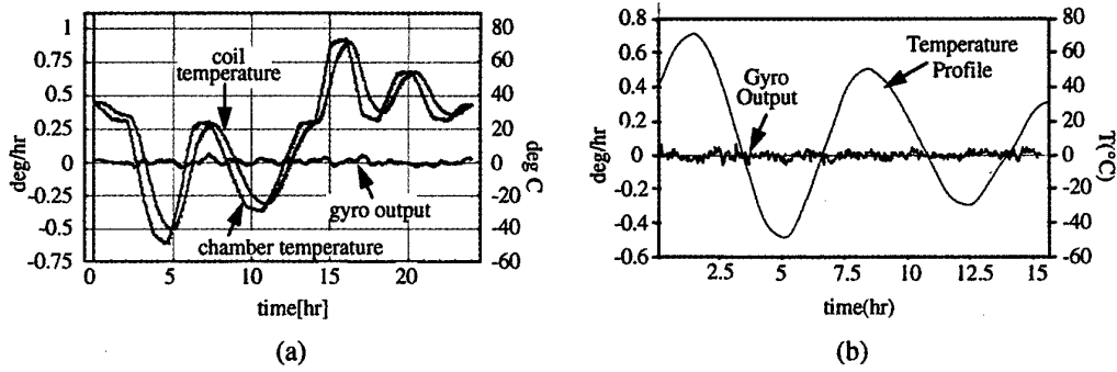
Figure 5: Thermal response of Honeywell depolarized FOG
