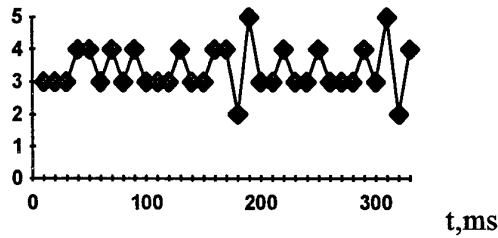
c) random vibration 5 g (\bar{N}=3.326 \text{ pulses}; \sigma_N=0.066 \text{ deg/s})
