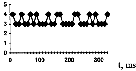
b) random vibration 2.4 g (\bar{N}=3.339 \text{ pulses}; \sigma_N=0.047 \text{ deg/s})
