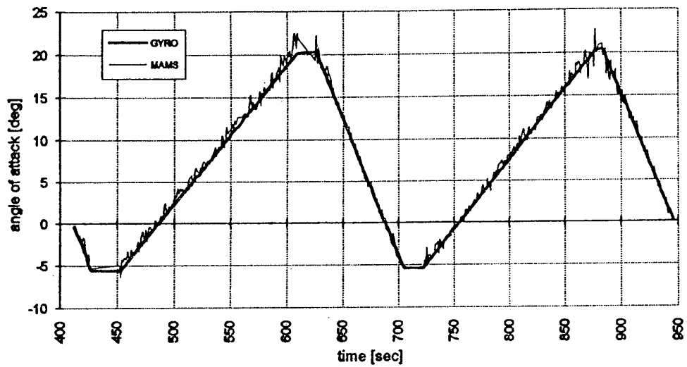
Figure 6.6 Angle of Incidence versus Time as measured by the FOG plus DIMT and by MAMS
