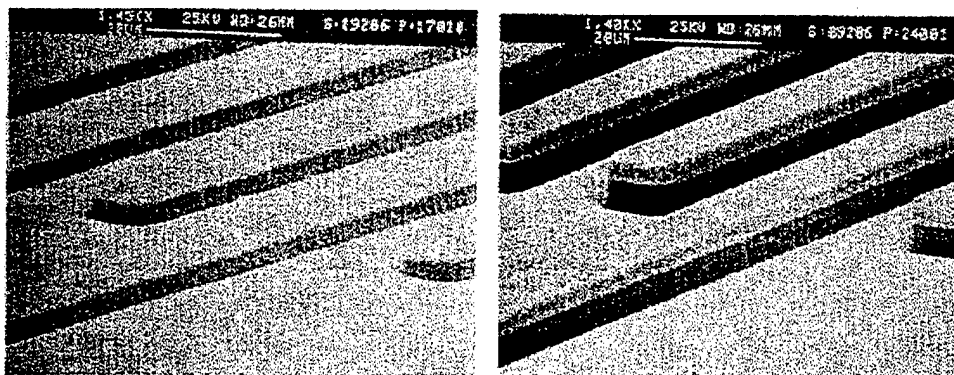
Figure 18 Etching of polymer waveguides using laser ablation
