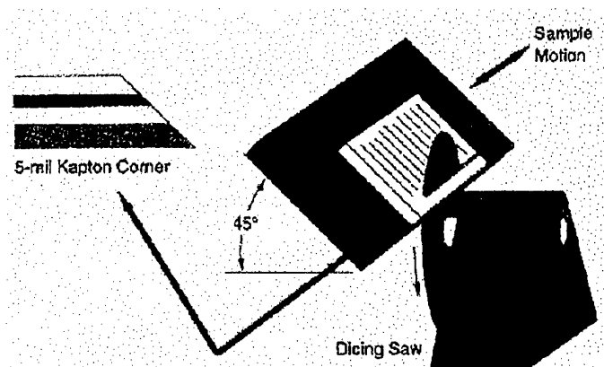
Figure 20 Mechanical preparation of angled end-faces
