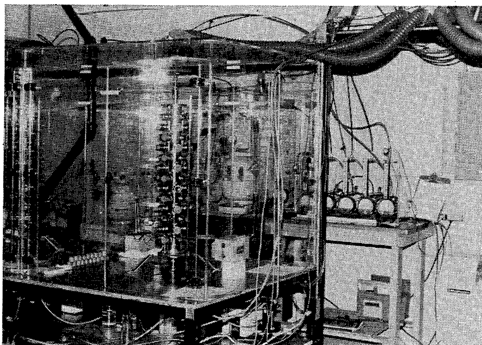
Figure 10.1-2. Nose-Only Inhalation Facility. Plexiglas enclosed chamber showing input and exhaust air lines.
