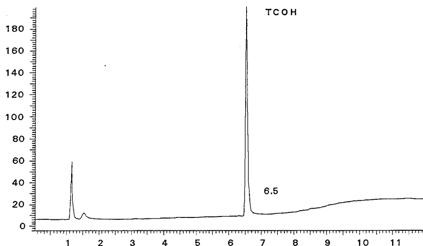
Figure 3.1-1. Chromatogram of a Urine Sample Containing 5 µg/mL TCOH. The retention time of TCOH was 6.5 min. Units of the y axis represent the detector response in millivolts.
