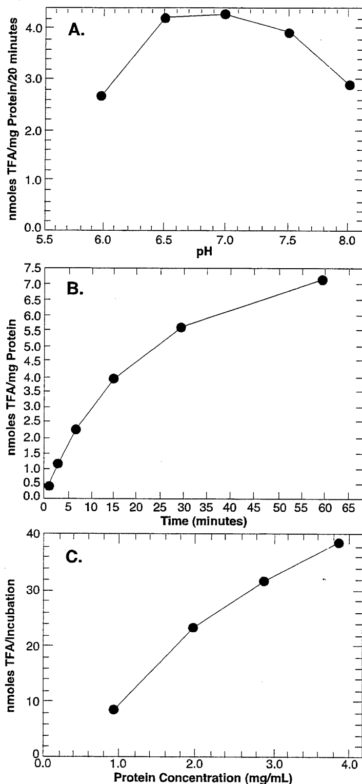
Figure 5.2-1. (A) Effect of pH on the Rate of TFA Formation from HCFC-123 in Human Hepatic Microsomes. Data are from a single experiment. (B) Time Course of the Formation of TFA from HCFC-123 in Human Hepatic Microsomes. Data are from a single experiment. (C) Effect of Human Hepatic Microsomal Protein Concentration on the Formation of TFA from HCFC-123. Data are from a single experiment
