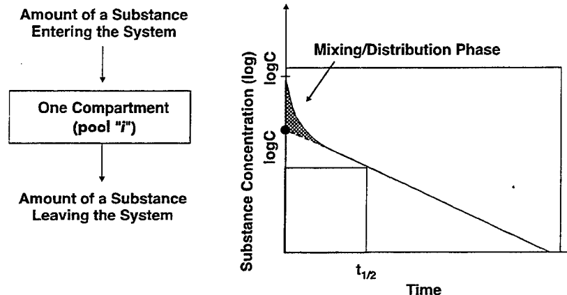
Figure 3.3-1. Basic Concepts of Classical Pharmacokinetics for One-Compartment Linear System.
