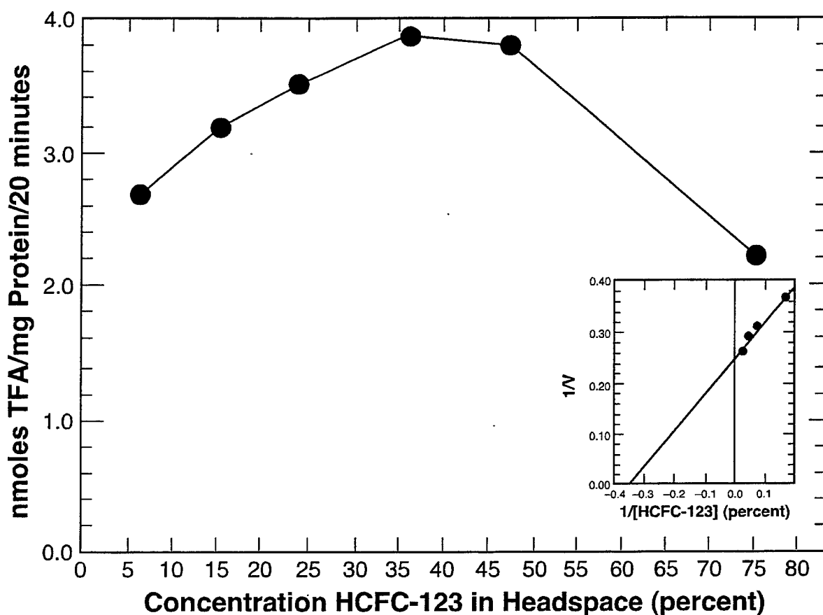
Figure 5.2-2. Substrate-Dependent Kinetics of TFA Formation from HCFC-123 by Human Liver Microsomes. Data are from a single experiment. Inset; double reciprocal plot of the first 4 points. (Apparent maximum rates and half-maximal substrate concentrations are provided in the Results section).
