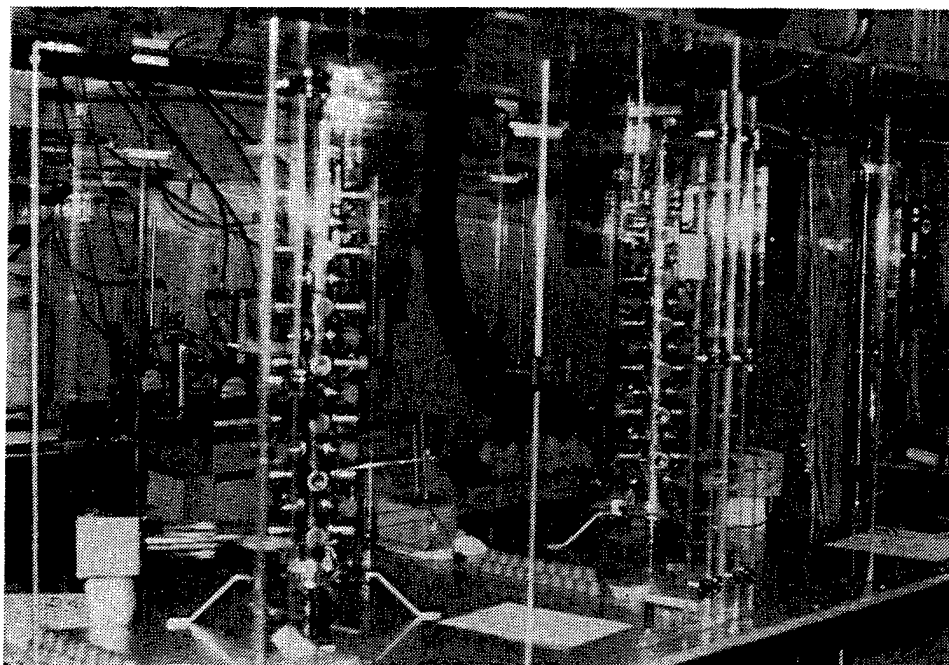
Figure 10.1-1 Nose-Only Inhalation Facility. Bench supporting two Cannon chambers, each within a plexiglas enclosure.
