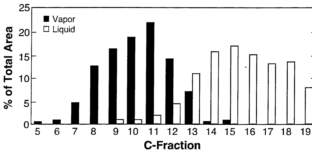
Figure 7.2-2. Bar graph plot of area slices data for shale DFM comparing relative percent of total peak area for vapor and liquid sample.
