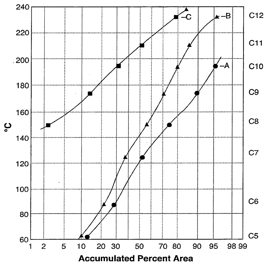
Figure 7.2-3. Probability plot of area slice data to determine the 16, 50, and 84% temperature cut-off points. A = Vapor, B = Liquid, C = Waste of Shale JP-4.
