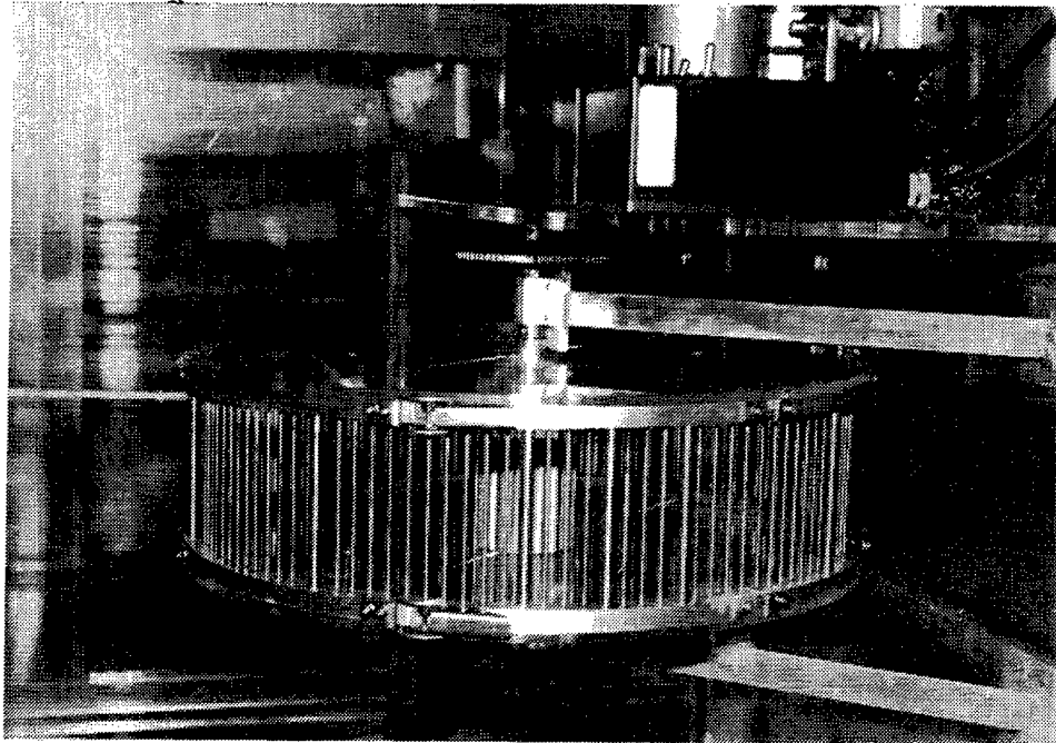
Figure 10.1-5. Combination Rotorod and Running Wheel Training Apparatus. This rotorod/running wheel was designed to function independent of inhalation chambers.
