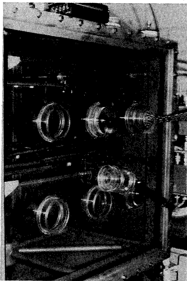
Figure 10.1-8. Nose-Only Chamber Exposure Apparatus. Animal Restraints are shown connected to the top and bottom right ports.
