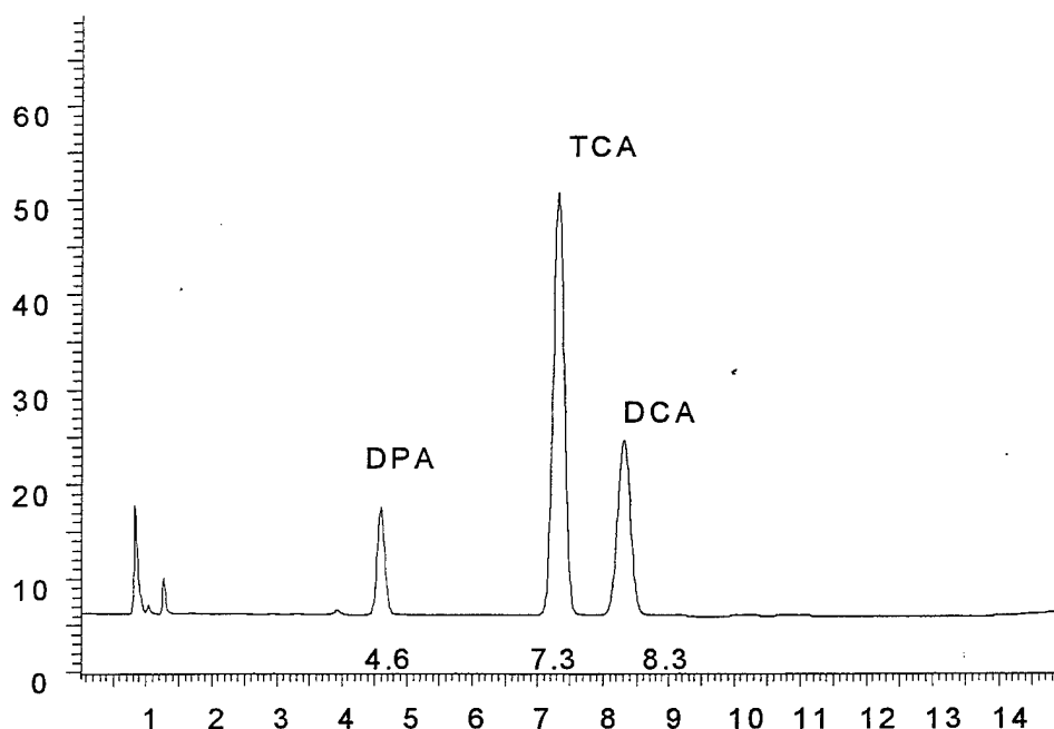
Figure 3.1-3. Chromatogram of 10 \mu g/mL TCA and DCA with Internal Standard DPA from Liver Homogenate. Retention times of DPA, TCA, and DCA were 4.6, 7.3, and 8.3 min, respectively. Units of the y axis is detector response in millivolts.
