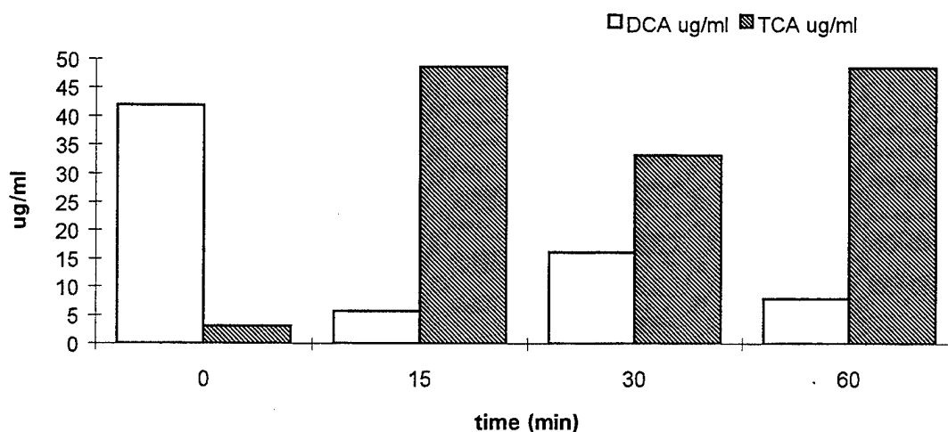
Figure 3.1-5. Conversion of TCA to DCA in Fresh Blood Samples from B6C3F1 Mice Spiked with 50 µg/mL TCA. Concentrated sulfuric acid was added at t = 0, 15, 30, and 60 min.
