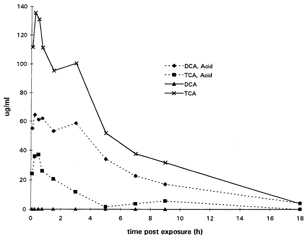
Figure 3.1-6. Conversion of TCA to DCA in Fresh Blood Samples from Mice Exposed to TCE. Samples at each time point were split into two portions. One portion was combined with 10% sulfuric acid (DCA, Acid and TCA, Acid), and the second with water (DCA, TCA).
