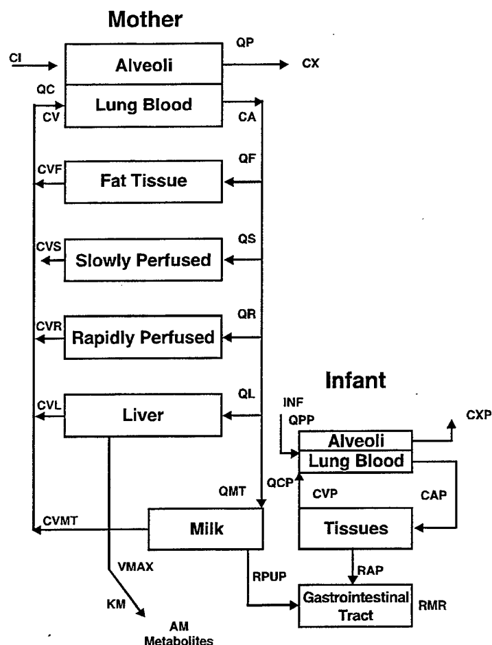
Figure 3.3-4. Scheme of Physiologically Based Pharmacokinetic (PBPK) Model Used to Simulate Lactational Transfer of PCE in Nursing Rats and Humans. (Byczkowski et al, 1994: Byczkowski and Fisher, 1994, 1994a, 1993).
