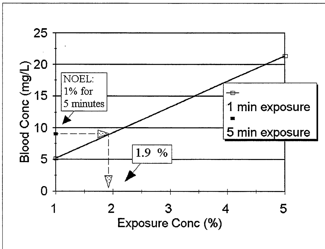
Figure 5.1-5. Extrapolation from the measured blood concentration at the NOEL. The 1-minute line connects blood concentrations measured after a 1-minute exposure to 1% and 5% HCFC-123.
