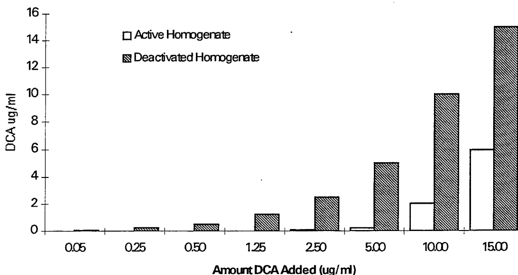
Figure 3.1-4. DCA Loss from Crude Liver Homogenate over 30 min at Room Temperature. Inactivated homogenate was inactivated with sulfuric acid.
