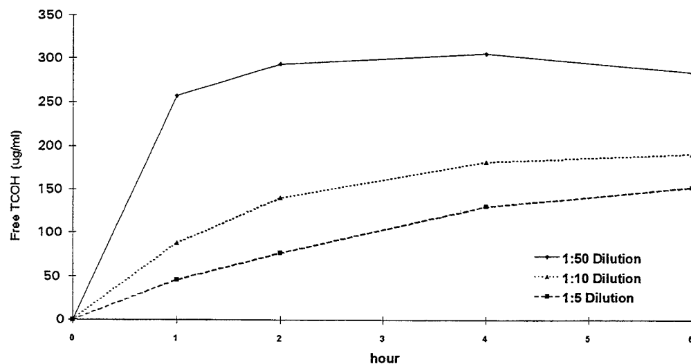
Figure 3.1-2. E. Coli \beta -Glucuronidase Incubations of 24-h Urine from Mice Exposed to 600 ppm TCE for 4 h.
