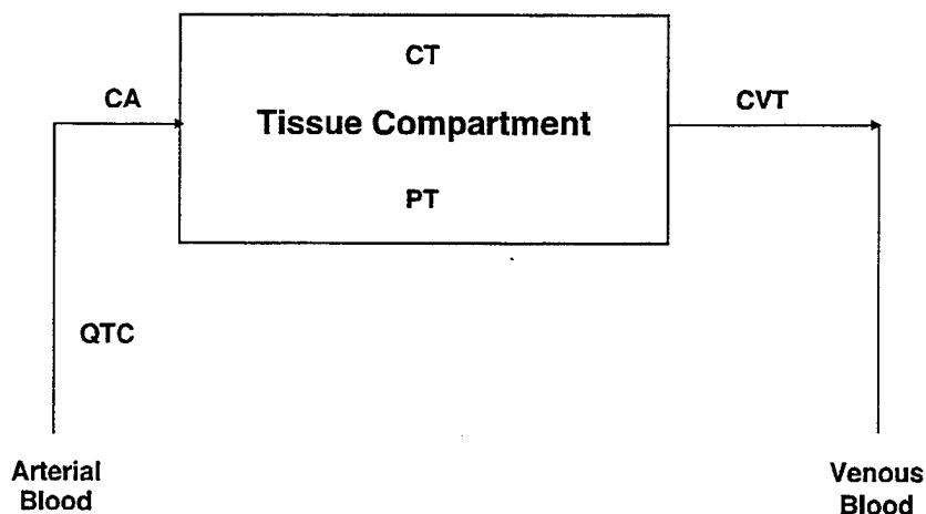
Figure 3.3-2. Basic Concepts of Physiologically Based Pharmacokinetic (PBPK) Modeling.
