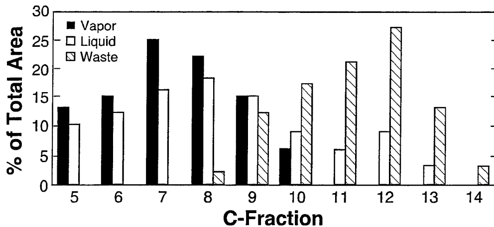
Figure 7.2-1. Bar graph plot of area slices data for shale JP-4 comparing relative percent of total peak area for vapor, liquid, and waste samples
