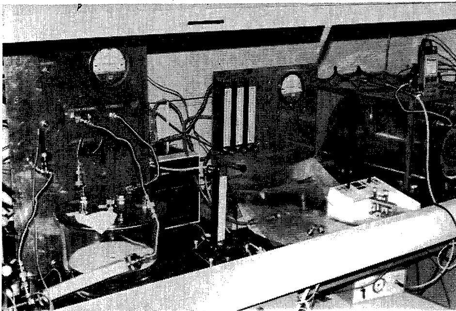
Figure 10.1-6. Gas-Uptake System. Stainless steel lid and exposure system with ancillary connections is shown on left.
