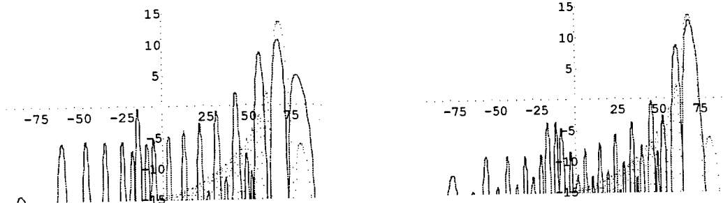
Figure 103. Time Delay Quantization (H) and (V) Configurations.
