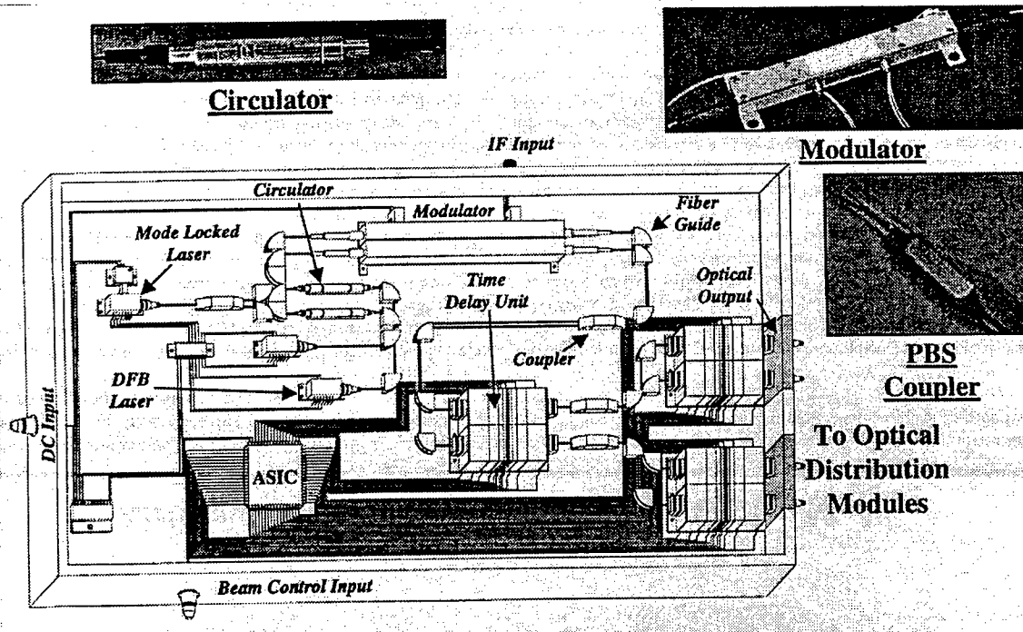
Figure 22. Airborne Transmit Array Optical Source Module.
