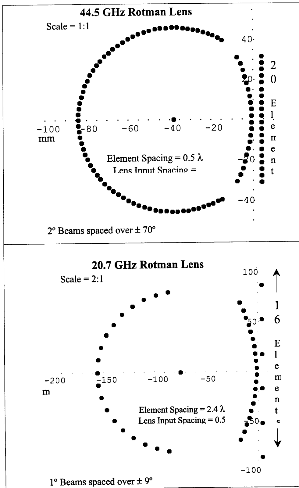
Figure 55. Optical Rotman Lens Geometry @ EHF.
