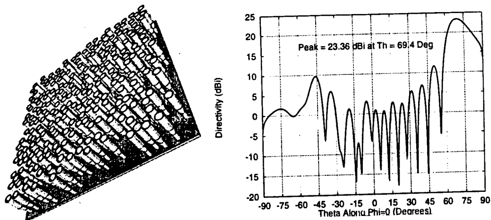
Figure 78. Transmit Antenna EIRP Analysis.
