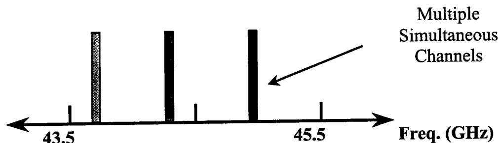
Figure 6. Airborne Transmit Frequency Allocation of COMM Assets.6
