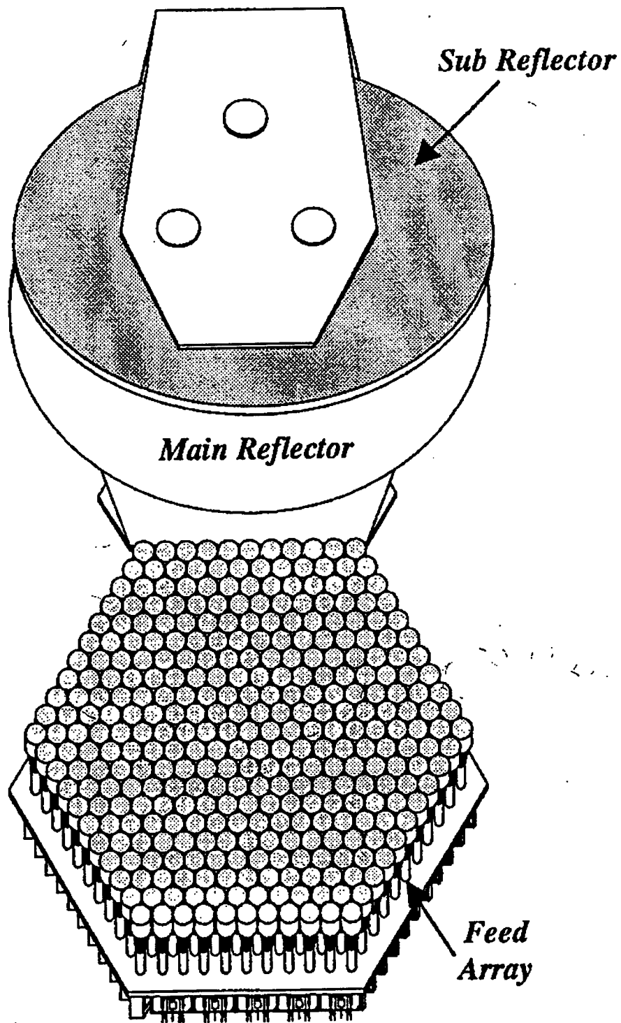
Figure 14. Spacebourne Receive Antenna (Top View).
