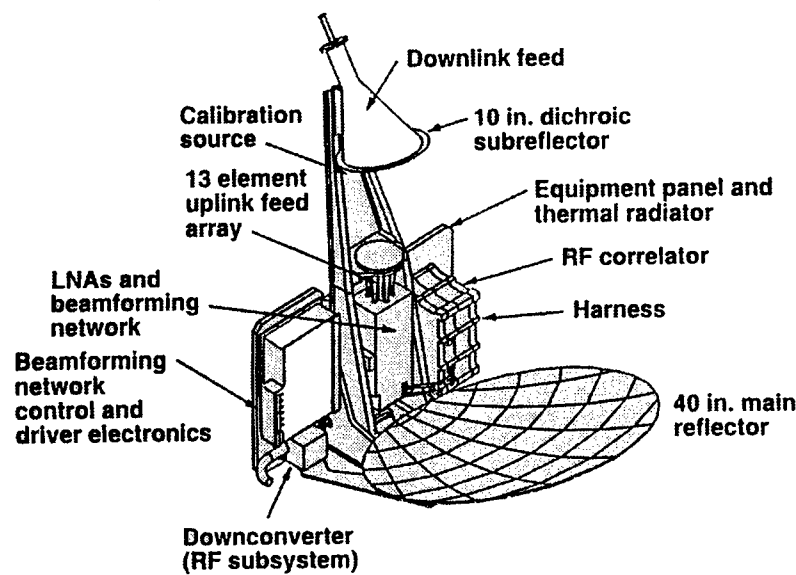
Figure 42. Milstar Nuller.
