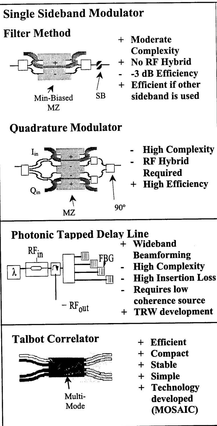
Figure 16. Several component technologies enable nulling antenna beamforming and signal processing.
