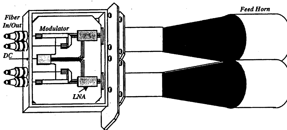
Figure 12. Receive Module.
