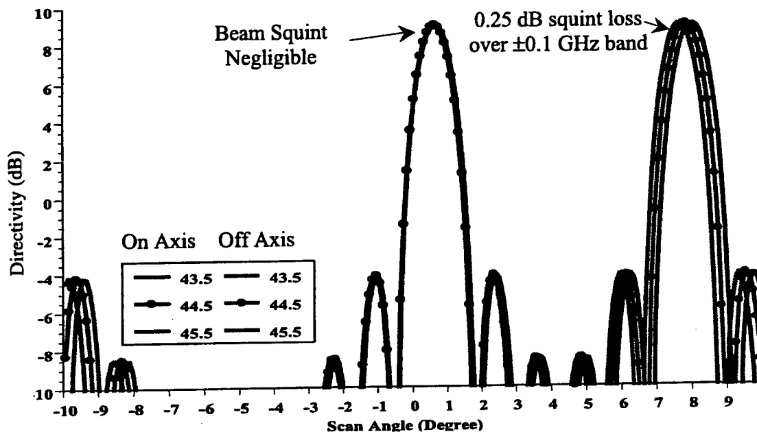
Figure 53. Butler Matrix Beamformer Performance.
