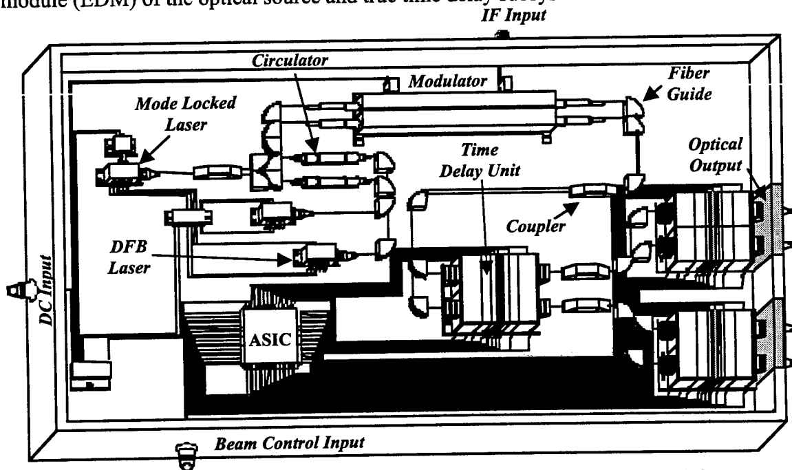
Figure 2.2 Airborne Transmit Optical Source and Time Delay Module
