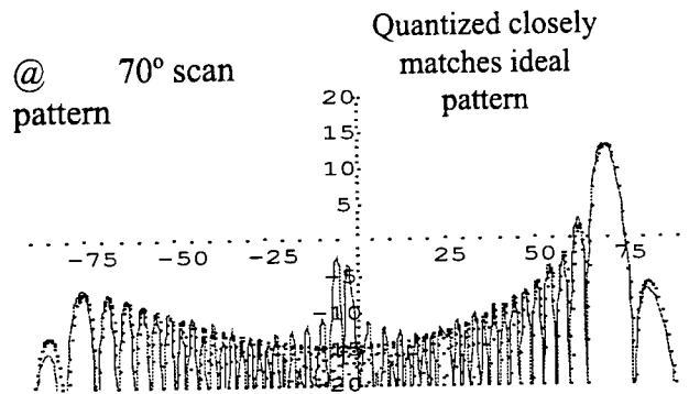
Figure 102. Four Bit Quantization.
