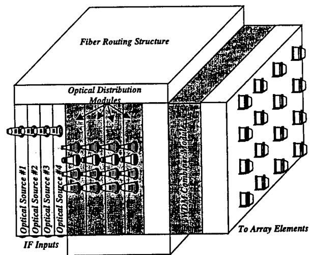
Figure 26. Photonic Implemented Beamformer.
