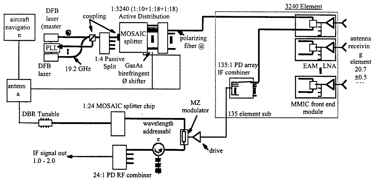
Figure 28. Scanning Array (Photonic).
