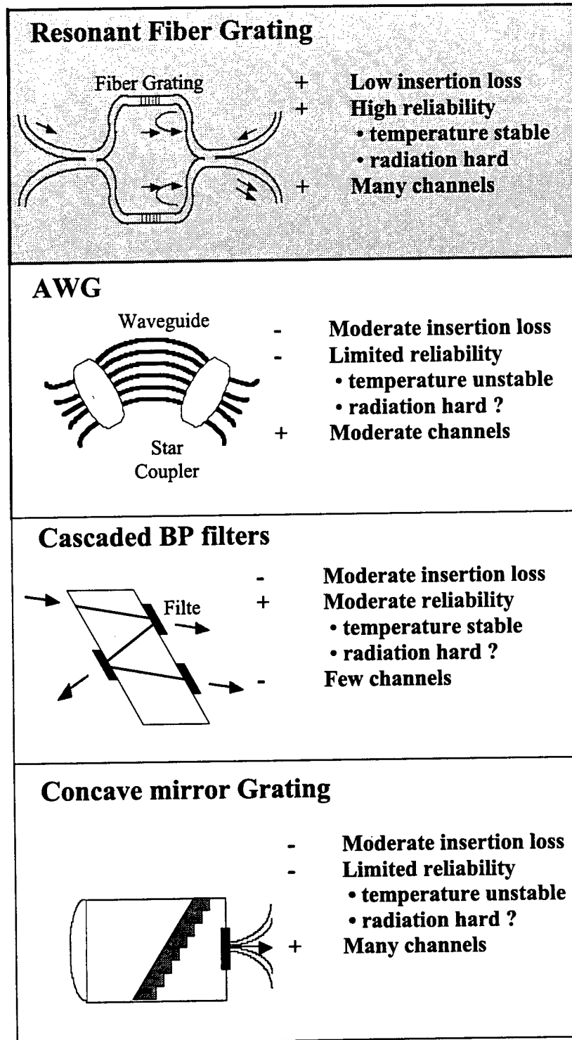
Figure 38. WDM Multiplexing.
