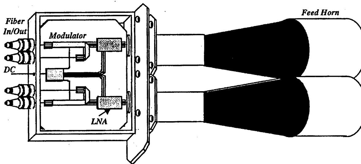
Figure 74. Receive Module.
