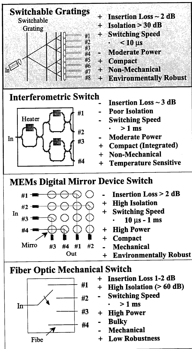
Figure 39. Optical Switching.
