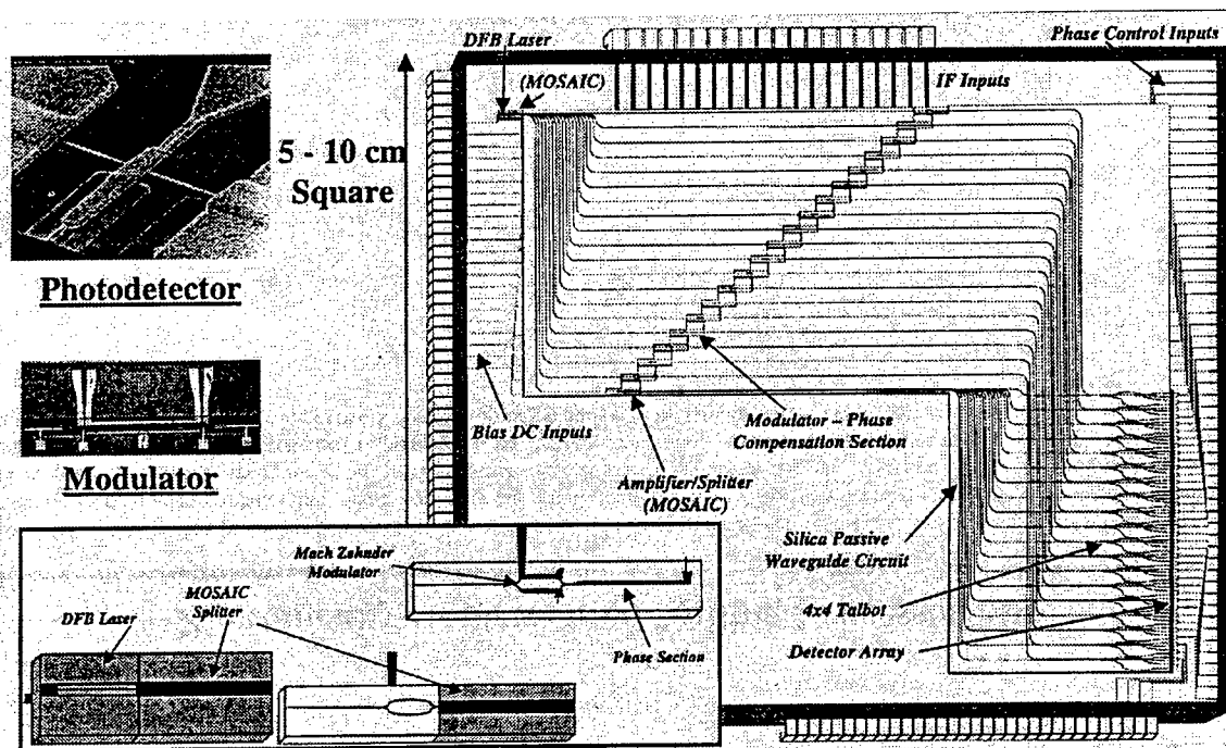
Figure 17. Photonic Correlator Multi-Chip Module.
