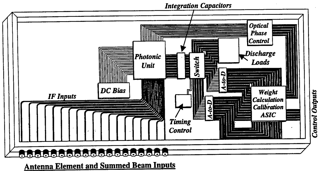
Figure 18. Photonically Implemented Nulling Processor Slice.
