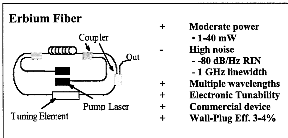
Figure 32. Optical Sources (2).
