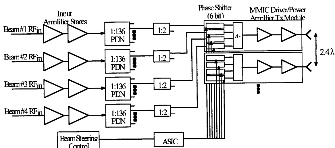
Figure 93. Scanning Array (RF).
