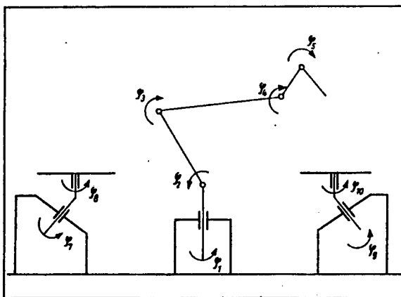
Figure 8. 0J-10 industrial robot
