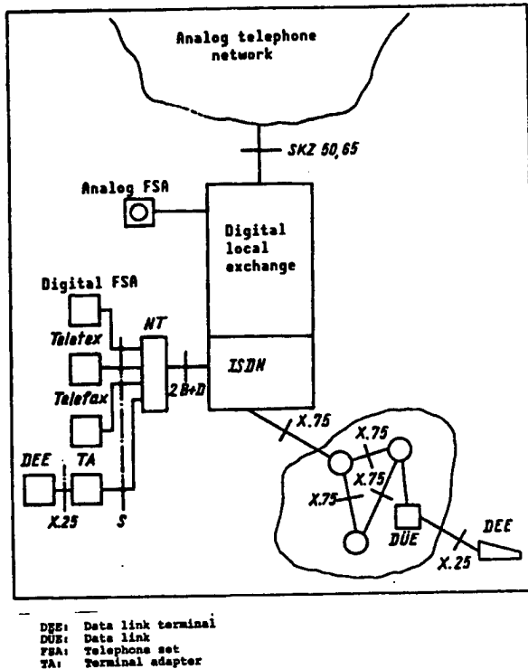
Figure 2. Digital Local Exchanges in the GDR Network
