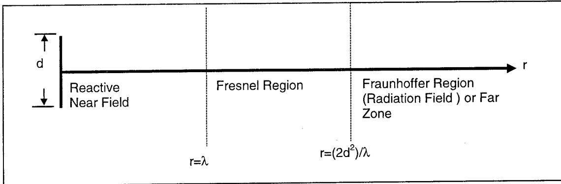
FIGURE 2 ANTENNA FIELD REGION
