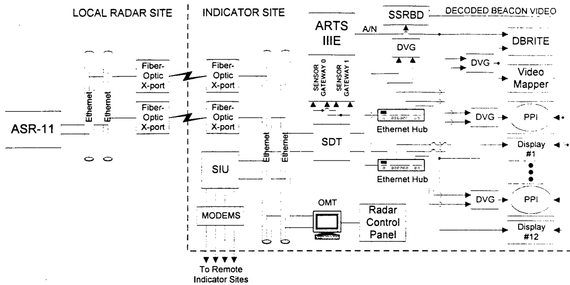
FIGURE 3.3-5. ASR-11 TO ARTS IIIIE INTERFACE
