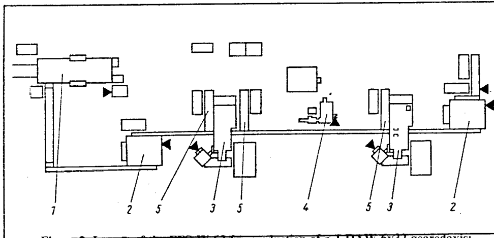
Figure 2. Layout of the FFS W 63 for production of a 1 DAW 6x32 geared axis; 2 WM 5Cx1200; 3 SASL 3 AE; 4 Unitherma 350; 5 cross storage
