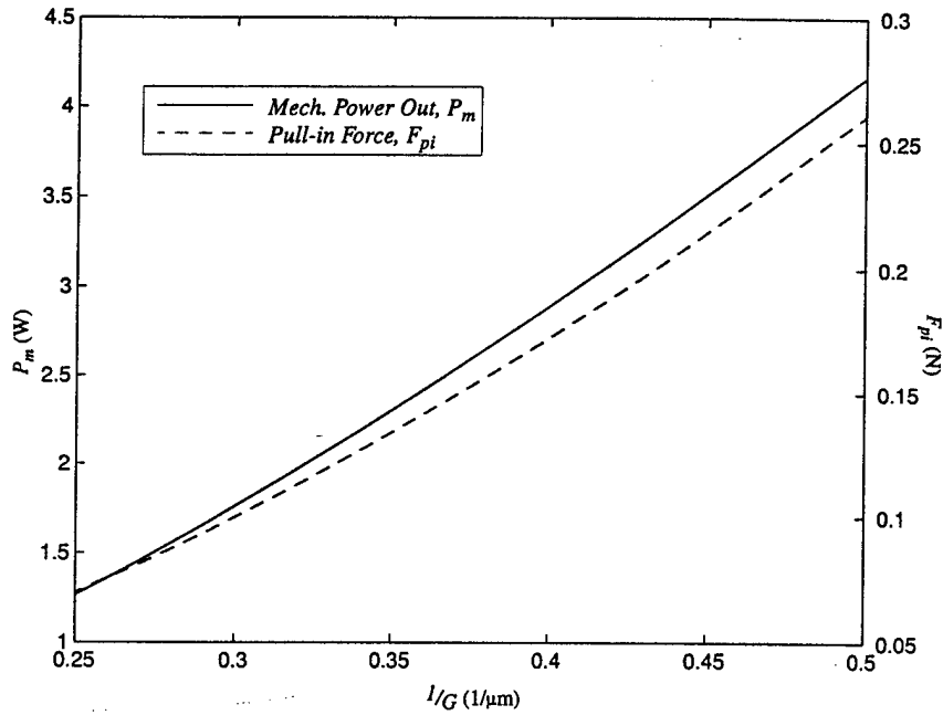
Figure A.4.10: .Peak mechanical power and peak pull-in force vs. the inverse of the air gap length. Peak force is defined as the force at the point of peak power. It is not the maximum force that occurs at synchronous speed, although that force scales similarly. Other model parameters are found in Table A.3.1 and Table A.4.1.
