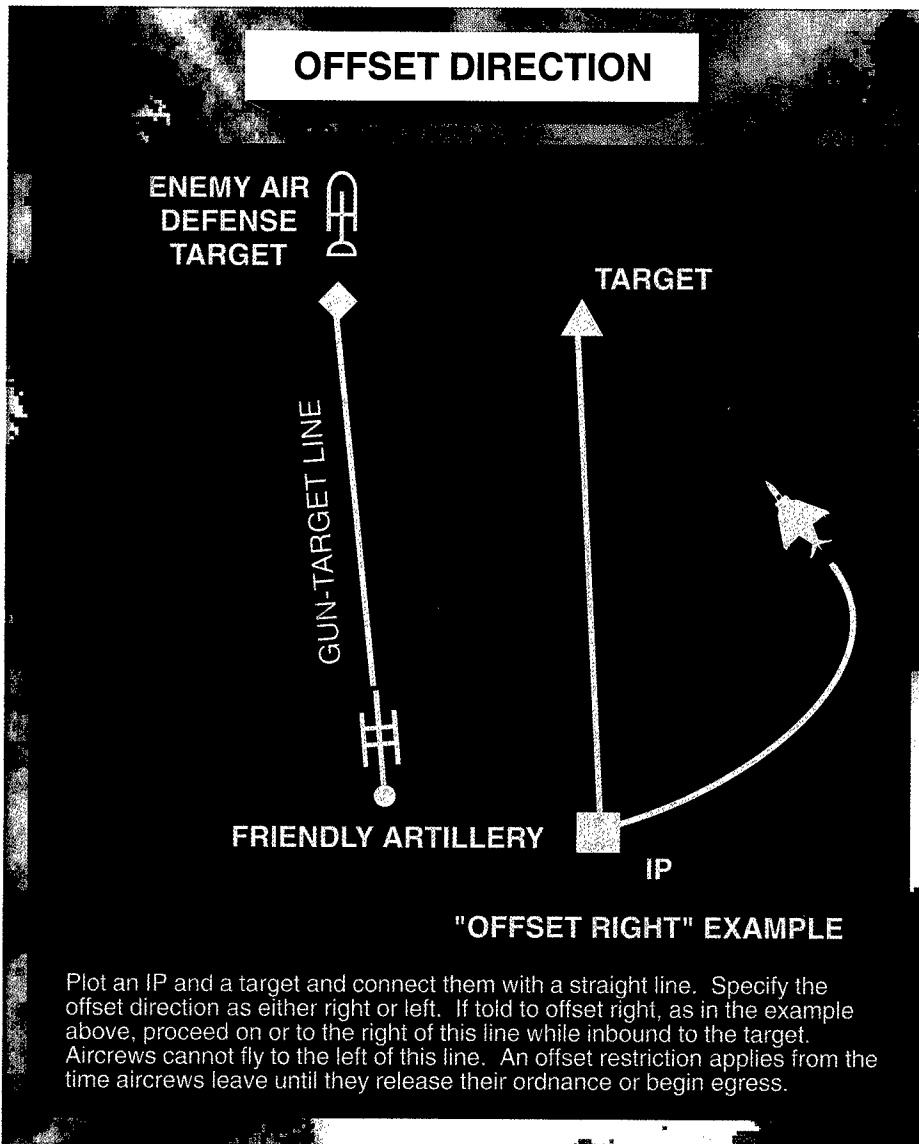
Figure V-16. Offset Direction
