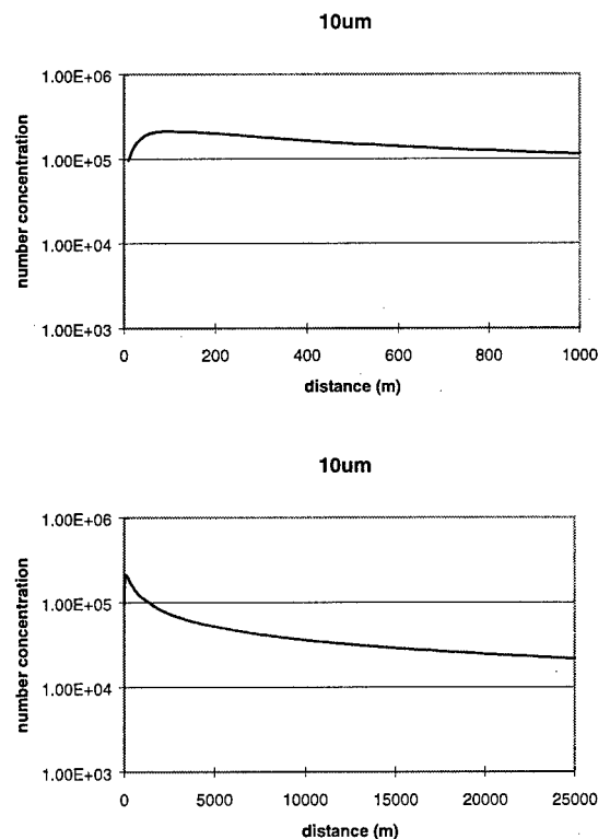
Figure 10. Aerosol concentrations for particles of 10 \mu\text{m} in diameter, calculated as a function of distance from the surf using the aerosol transport model described in the text.
