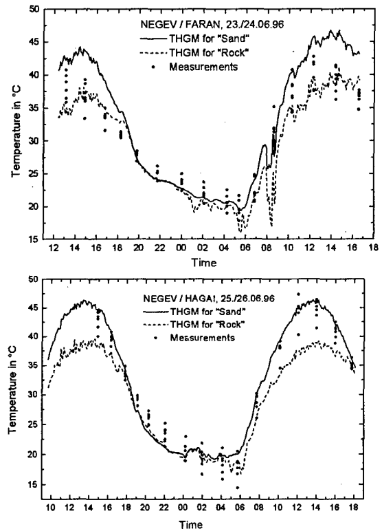
Fig. 13: Comparison between measured (points) and predicted (lines) surface temperatures (background types: "sand" and "rock") for the locations Wadi Faran (top) and Mizpe Hagai (bottom). Predicted time period: 23 - 26 June 1996.
