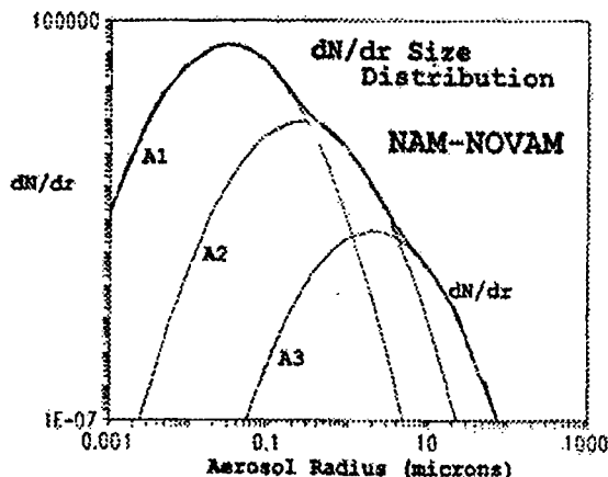
Figure 1. Note that the A_1 component (the largest curve) is dependent of the square of the air mass parameter. The AMP has a significant effect on the aerosol size distribution.
